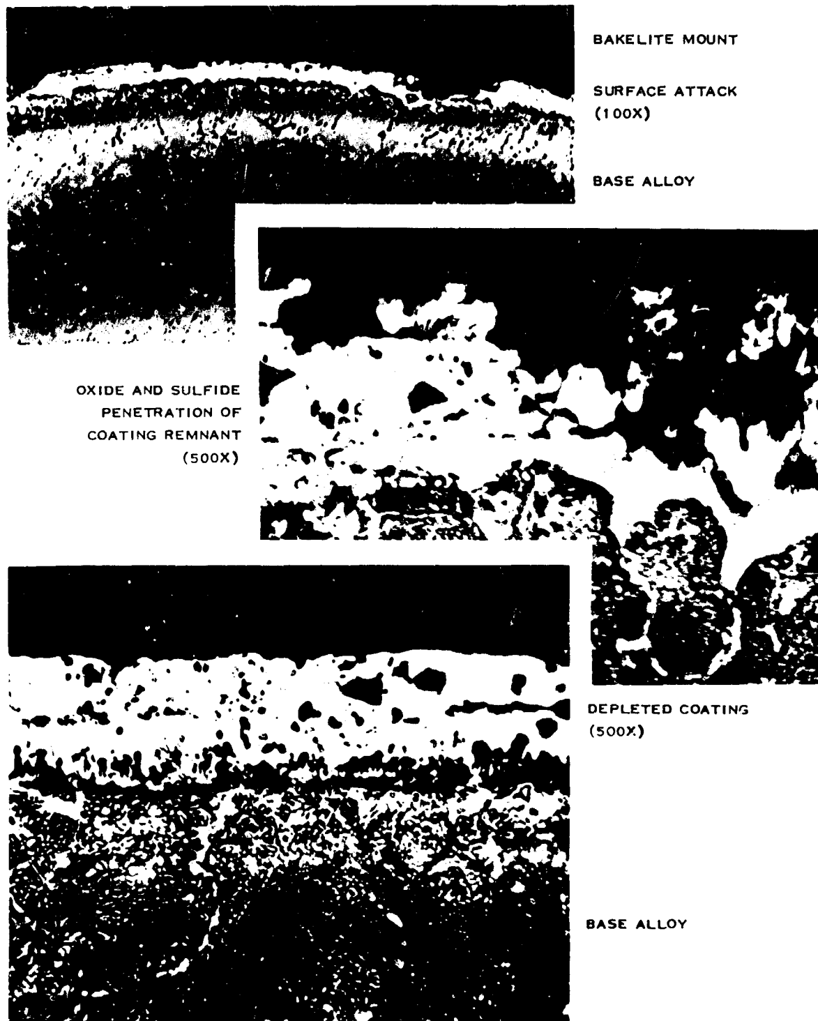
METALLOGRAPHIC CROSS-SECTION OF SPECIMEN FROM 2000 F CYCLIC TEST IN PHILLIPS TURBINE SIMULATOR WITH 1.0 PPM SEA SALT IN AIR AND 0.04 WT % SULFUR IN FUEL. ELECTRO-CLEANED, 10% OXALIC ACID-ELECTROLYTIC ETCHED.
