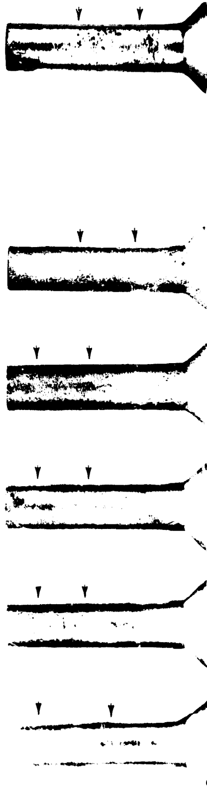
SPECIMENS FROM TEST WITH 0.1 VOL % ETHYL CI-2 ADDED TO FUEL
