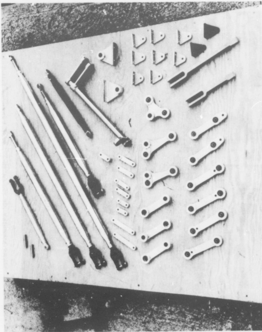
Figure 15. MSAS Components.
