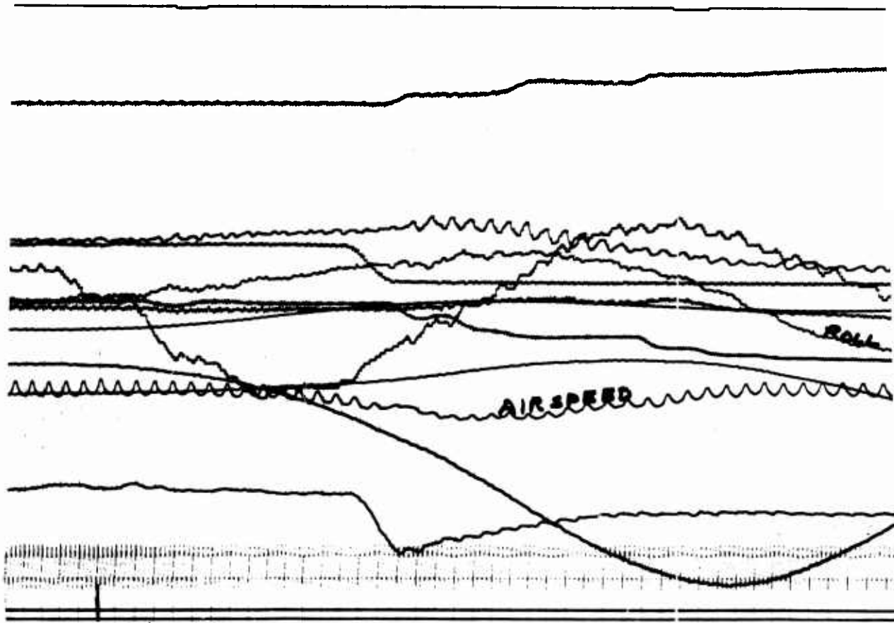
Figure 26. Autorotational Entry - 60 KIAS, 4000 Feet, With Stabilizer Bar.
