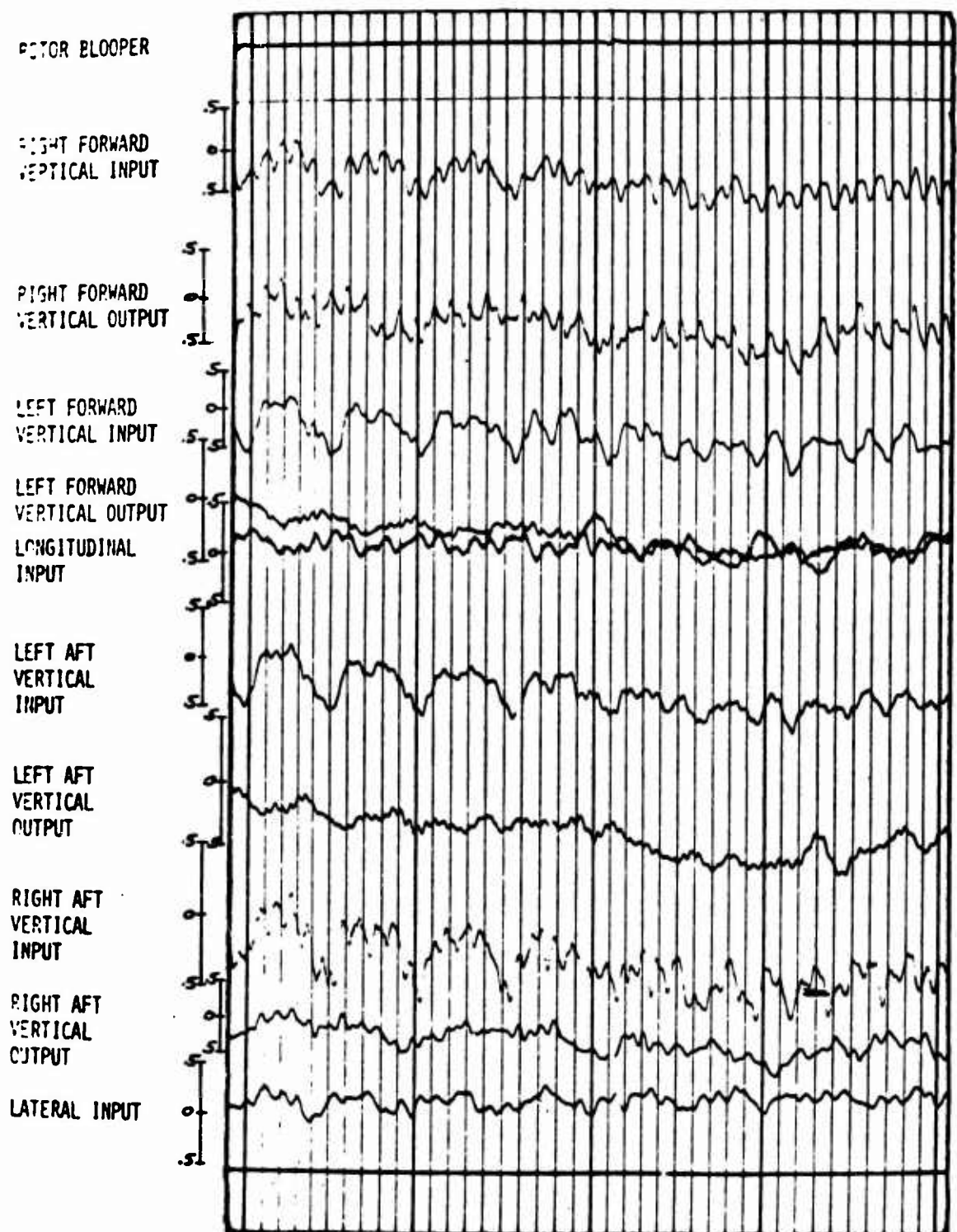
Figure 71. 200-Pound With a Three-Inch CG Offset Unidirectional Platform Oscillograph Traces of a -.5 Pushover at 100 Knots.
