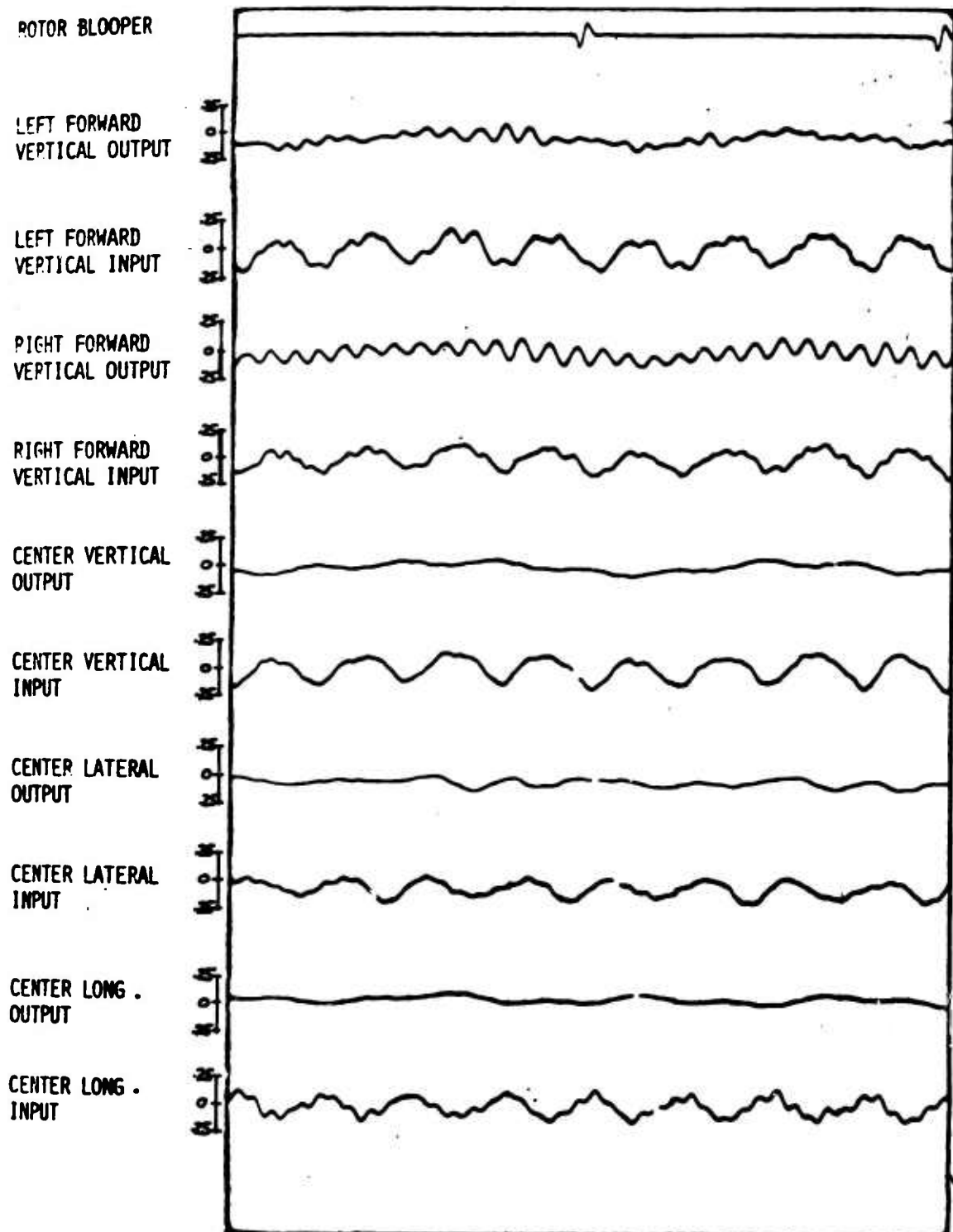
Figure 48. 200-Pound Conventional Platform Level Flight Oscillograph Traces.
