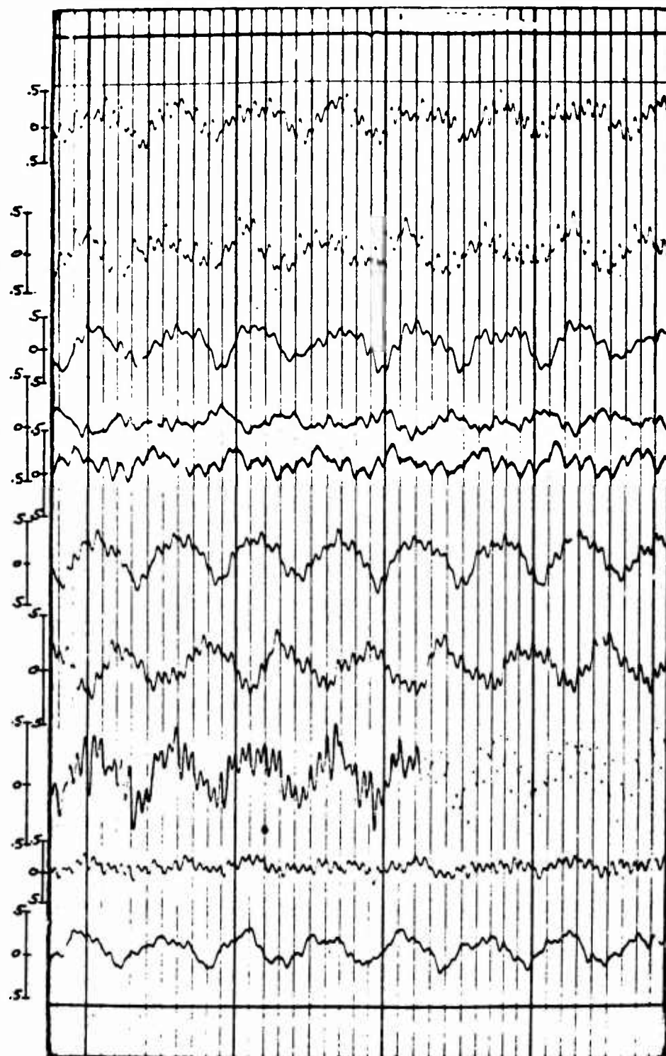
Figure 67. 150-Pound Unidirectional DAVI Platform Level Flight Oscillograph Traces.
