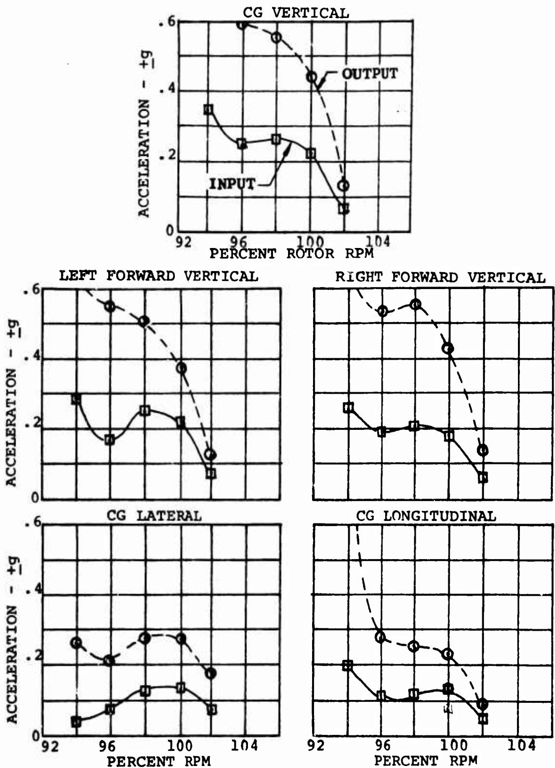
Figure 54. 30-Knot Four-Per-Rev Results of the 50-Pound Conventional Platform.
