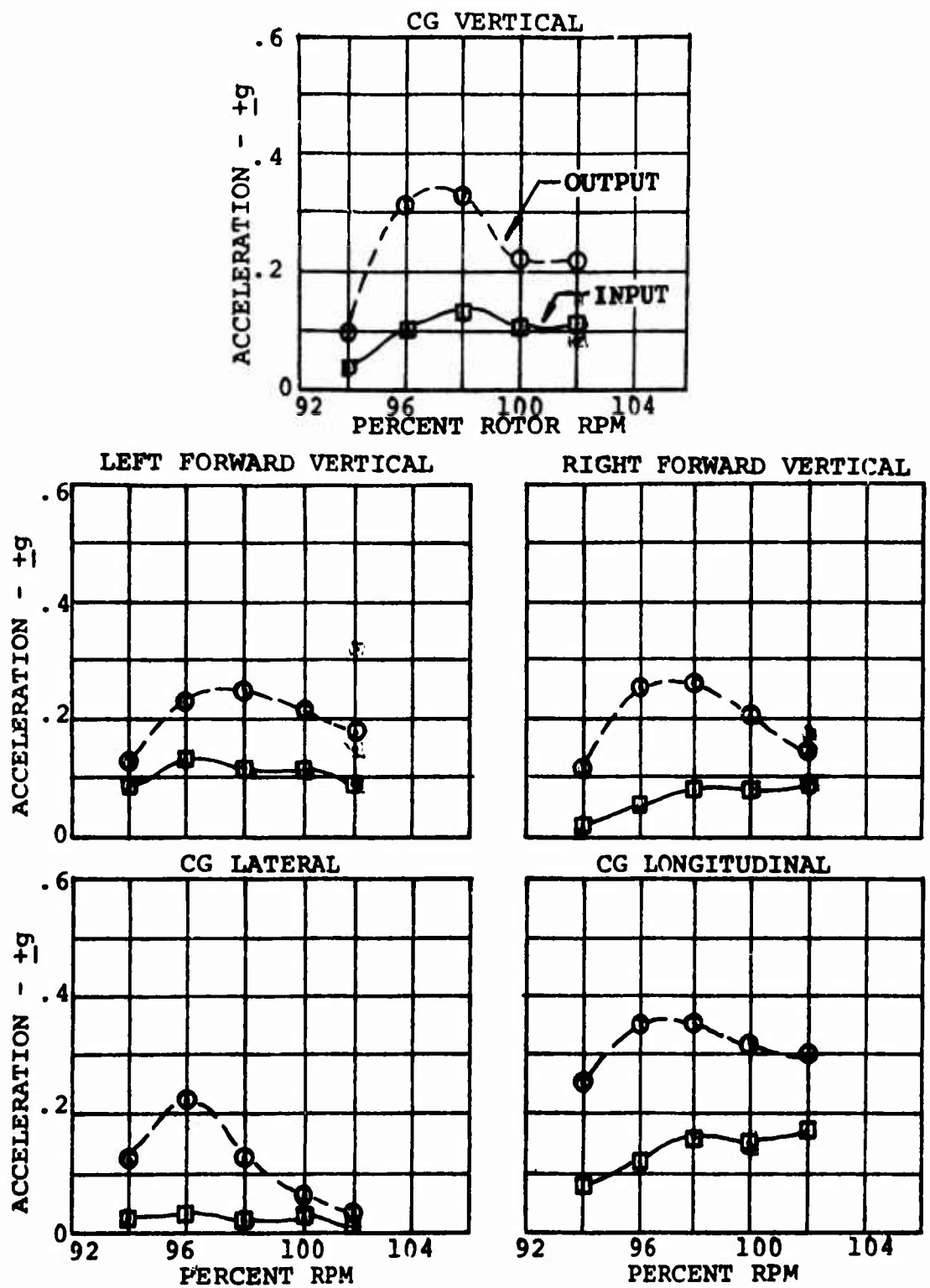
Figure 55. 120-Knot Four-Per-Rev Results of the 50-Pound Conventional Platform.
