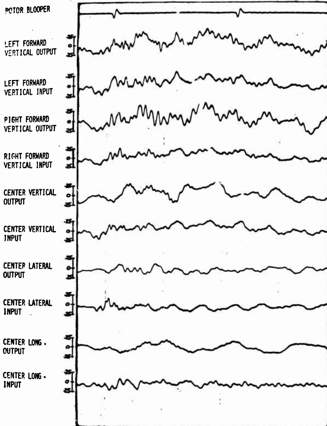
Figure 96. Oscillograph Traces of the Landing Conditions for the 150-Pound Two-Dimensional DAVI Platform With Longitudinally Offset Pivots.
