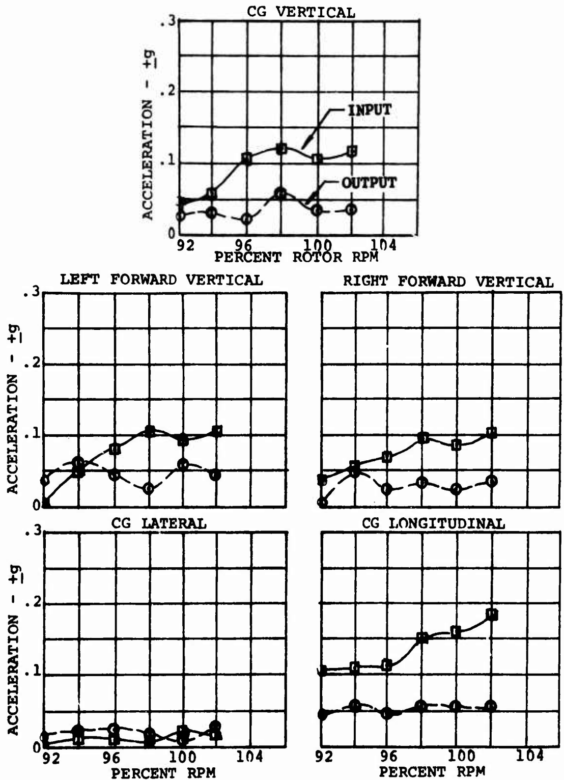
Figure 57. 120-Knot Four-Per-Rev Results of the 150-Pound Conventional Platform.
