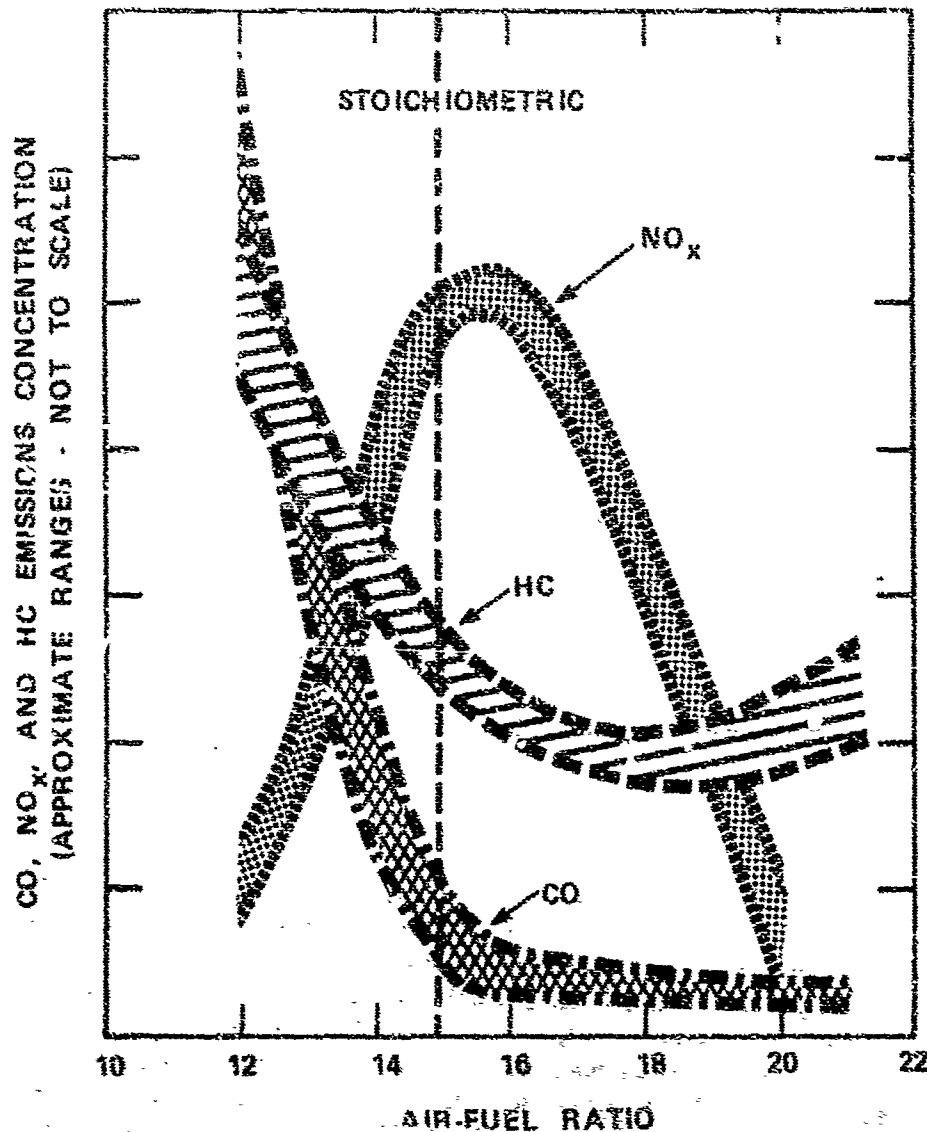
Figure 1. Effects of air-fuel ratio on exhaust composition. 1
