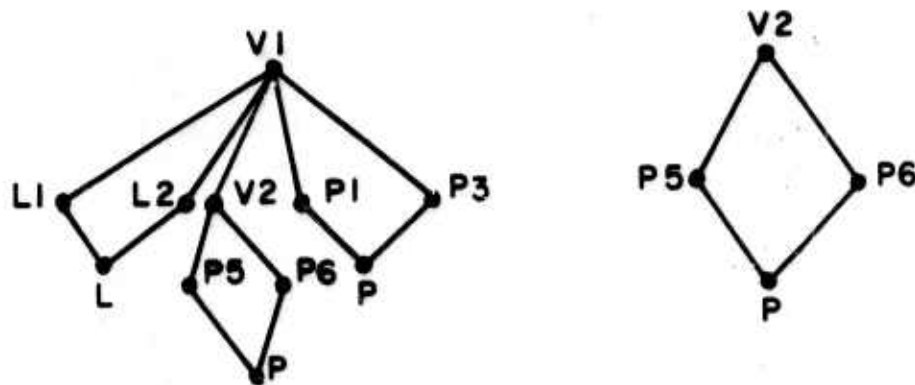
Figure C-7. Path of display file generator through a semilattice data structure.
