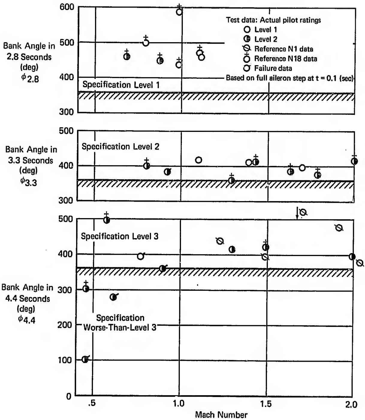
Figure 2 (3.3.4.1.1) Roll Control Effectiveness C0 Configuration
