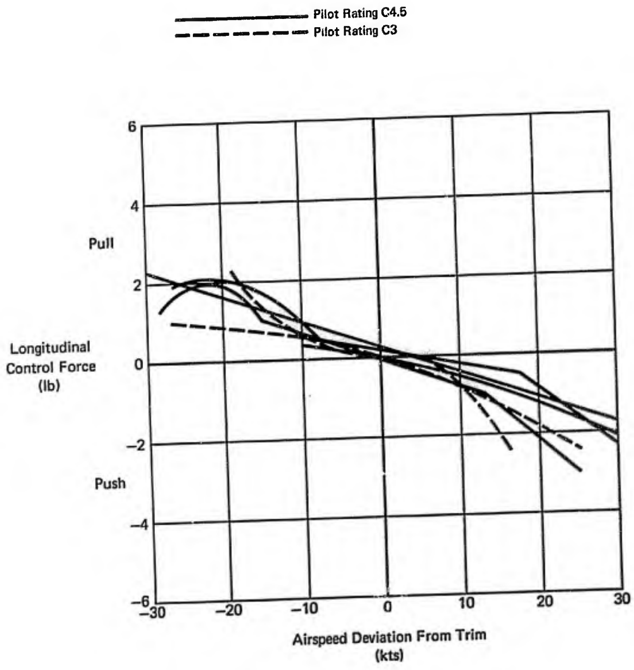
Figure 9 (3.2.1.1) Longitudinal Static Stability Feel/Trim System S3 High Lift Configurations Summary
