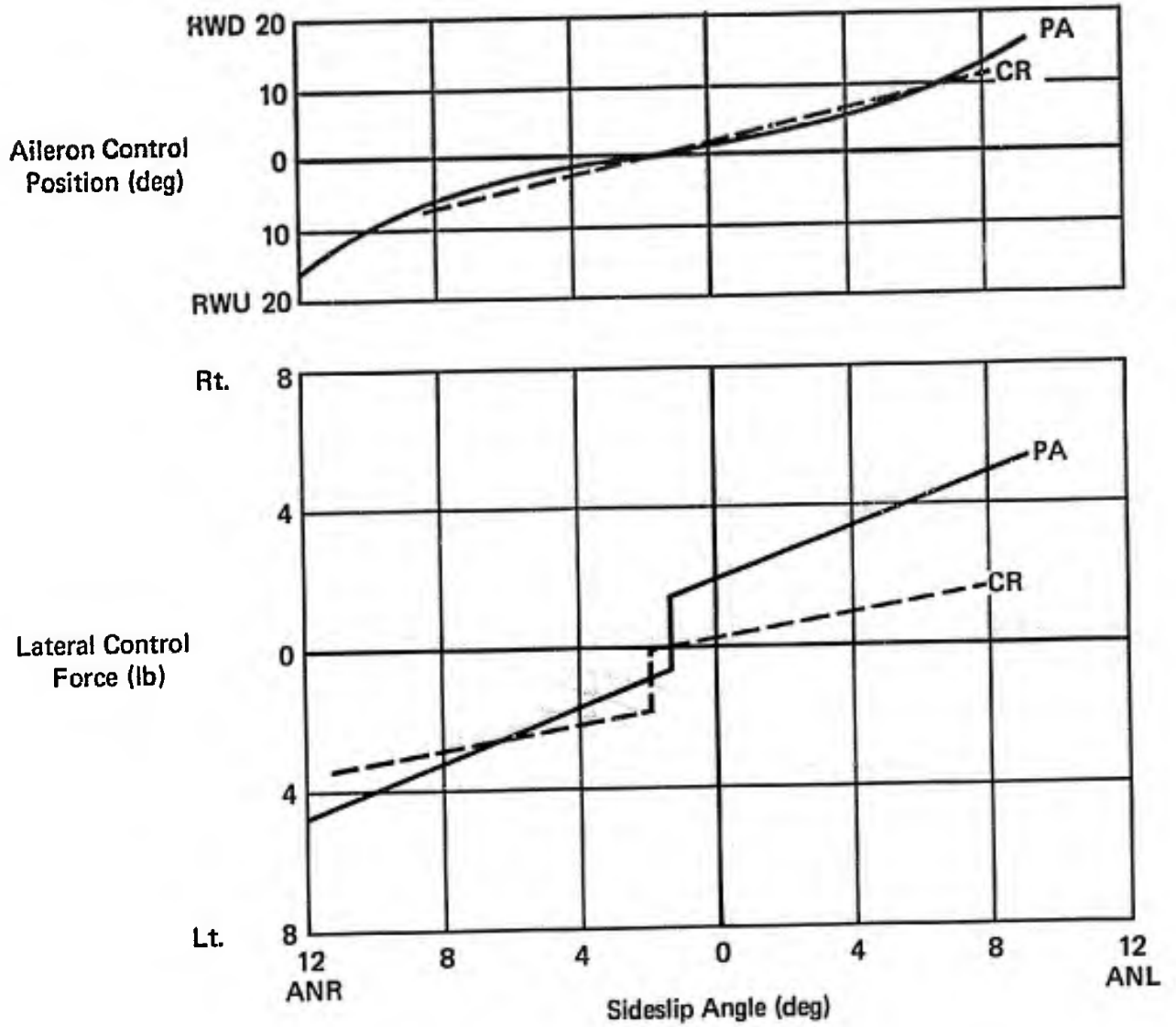
Figure 4 (3.3.6.3) Dihedral Effect Reference A1, F-4C Two 370-gal Wing Tanks + Eleven M117 Bombs
