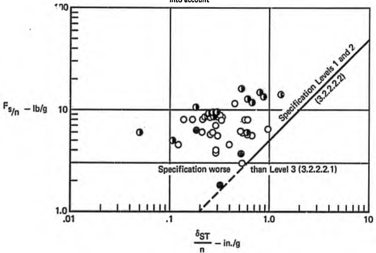
Figure 1 (3.2.2.2.2) Control Force Per Control Displacement
