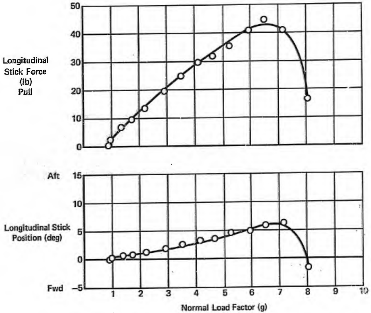
Figure 15 (3.2.2.2.1) Longitudinal Maneuvering Stability Cruise Configuration – Feel/Trim System S4 Reference A4, F-4C
