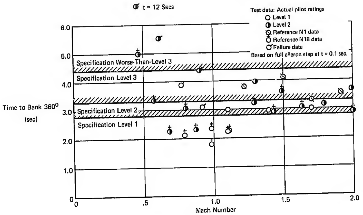
Figure 4 (3.3.4.1.1) Roll Control Effectiveness Time to Bank 360^\circ , CO Configuration
