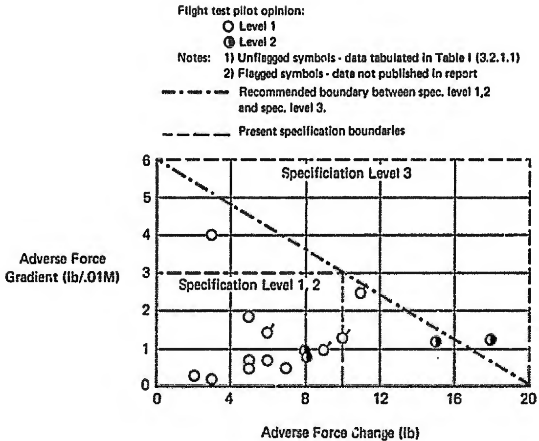
Figure 19 (3.2.1.1) Correlation of Pilot Rating Data With Transonic Static Instability Parameters CR/F/CO Configurations
