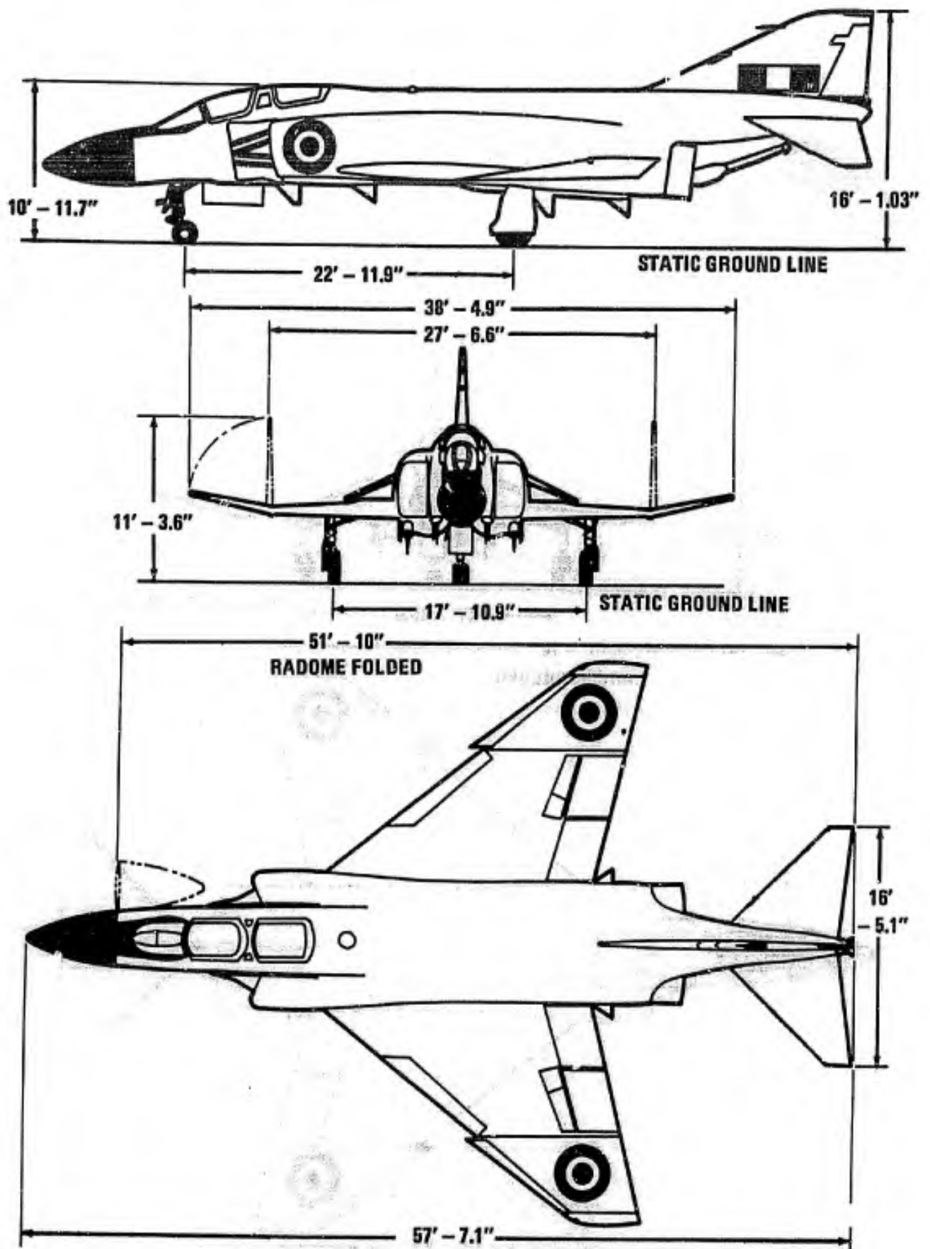
Figure 9 (II.I) Model F-4M
