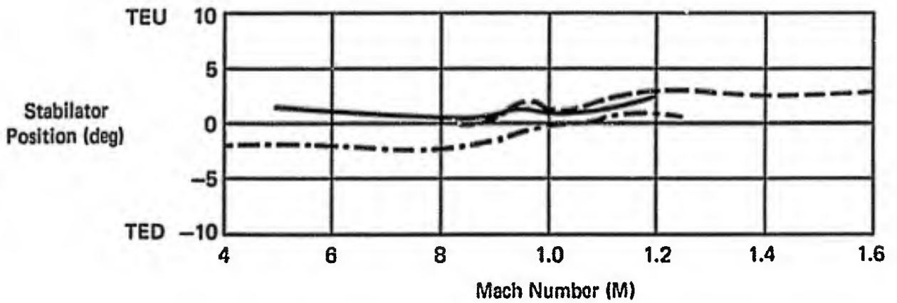
Figure 18 (3.2.1.1) Longitudinal Stability With Respect to Speed Longitudinal Static Stability S-4 Feel/Trim System CR/P/CO Configurations References N11 & A7
