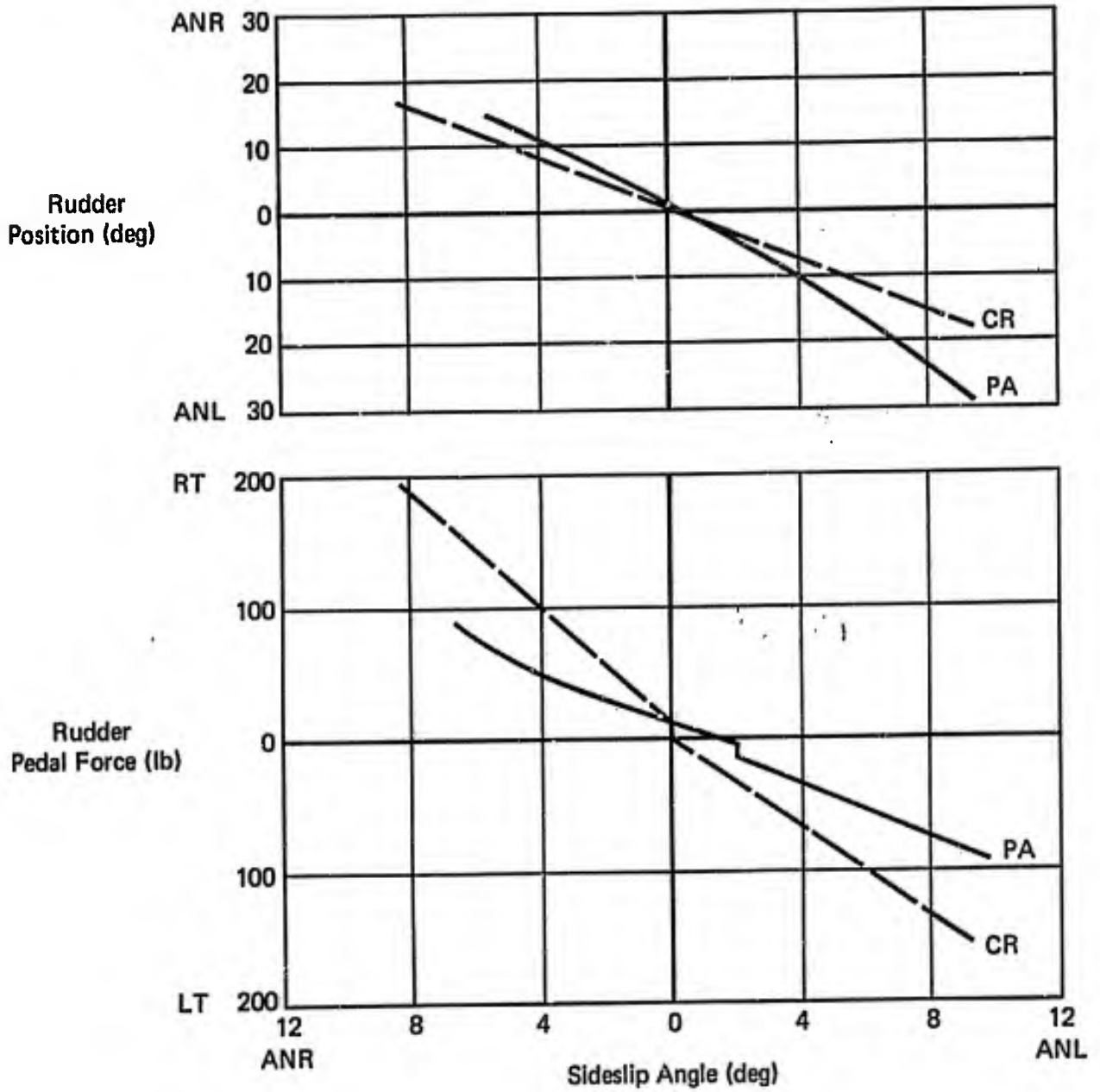
Figure 6 (3.3:6.1) Static Directional Stability Reference AB, F-4E Two 370-Gal. Wing Tanks + Six M117 Bombs
