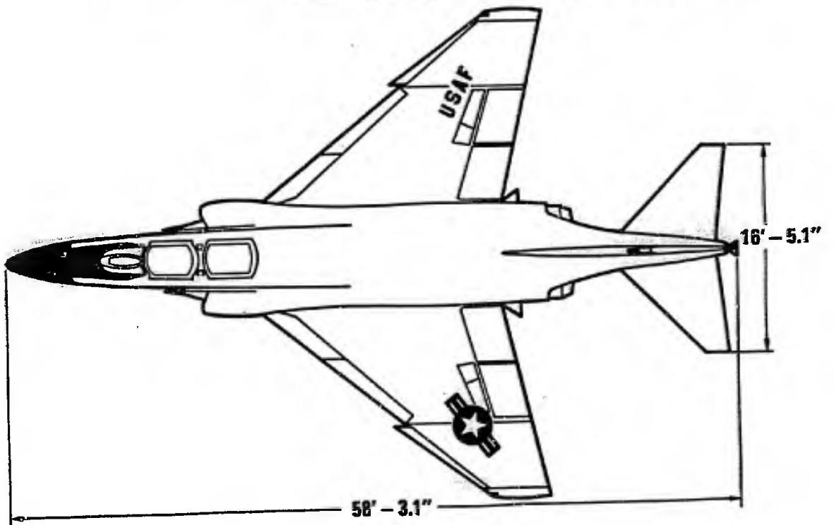
Figure 5 (II.1) Model F-4D
