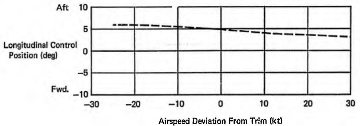
Figure 17 (3.2.1.1) Longitudinal Stability With Respect to Speed Longitudinal Static Stability Feel/Trim System S-4 PA Configuration References N11 & A7
