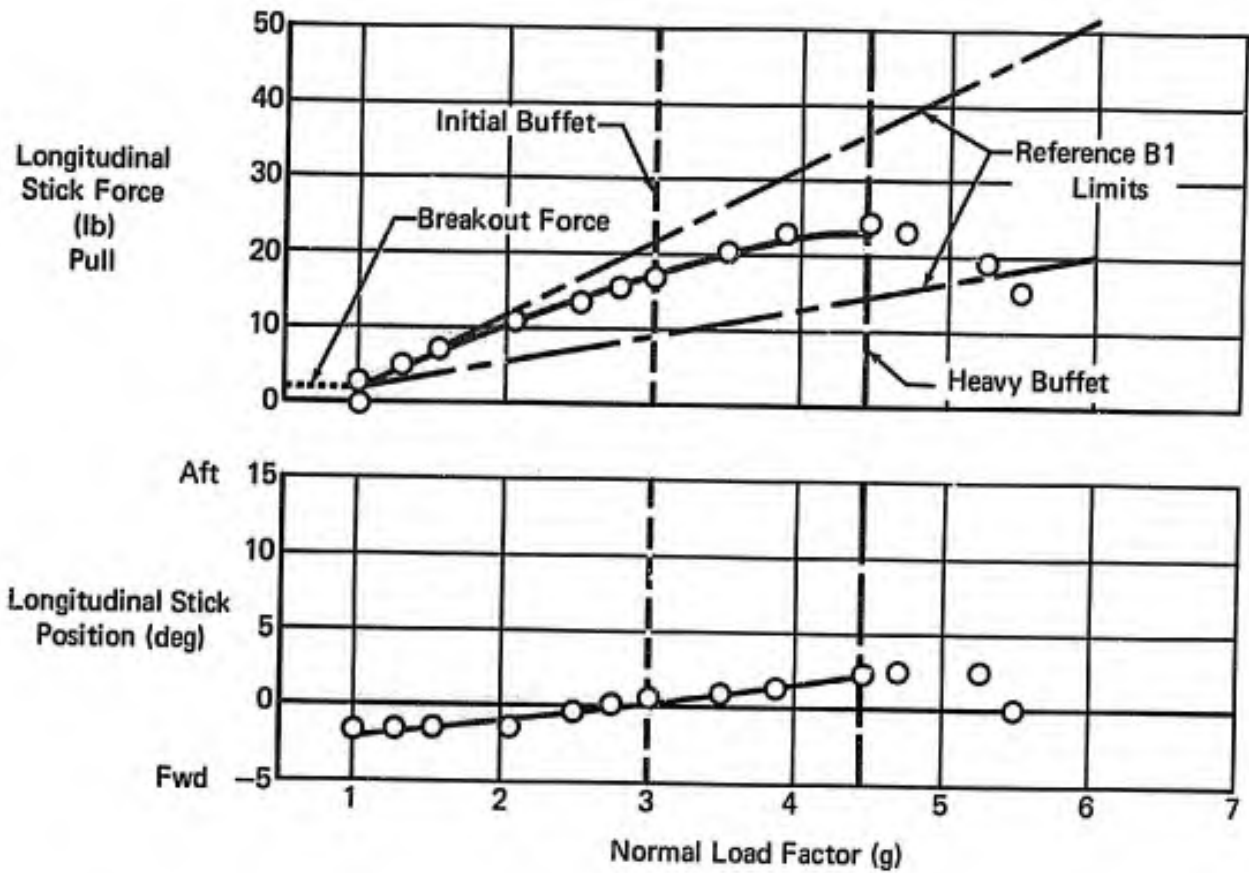
Figure 11 (3.2.2.2.1) Longitudinal Maneuvering Stability Cruise Configuration – Feel/Trim System S3 Reference A5, F-4C
