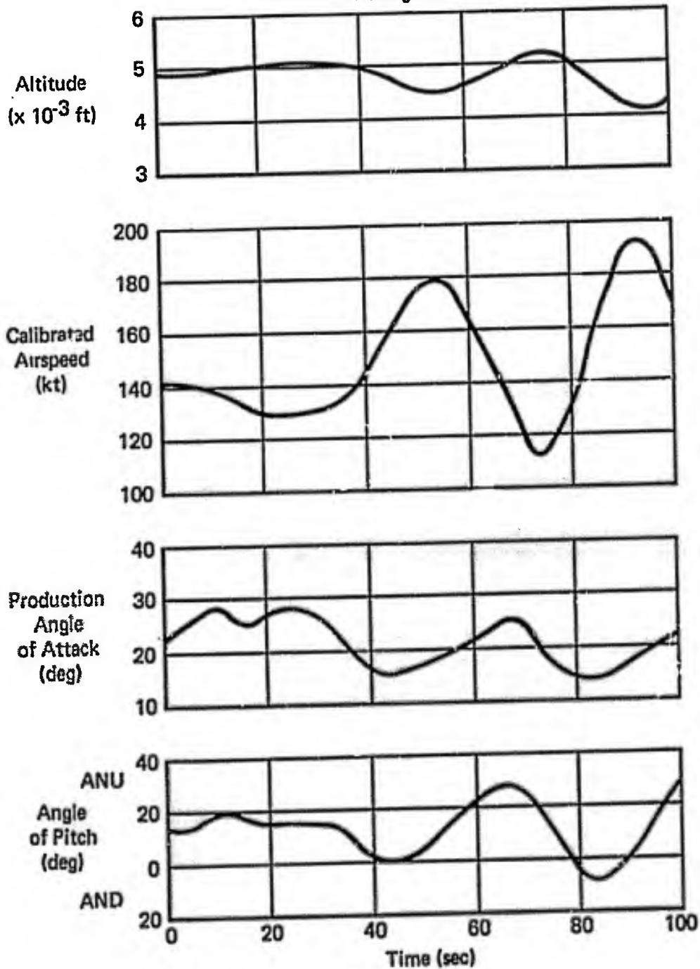
Figure 2 (3.2.1.2) Phugoid Stability Feel/Trim System S3, Stick Free Reference N13, F-4M
