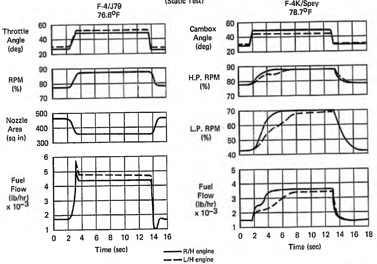
Figure 3 (3.6.2) Engine Response Comparison, 78% to 88% (H.P.) RPM GE-J79/Spay MK 201 Full Flap
