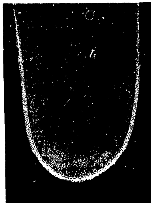
Magnification: 40X
