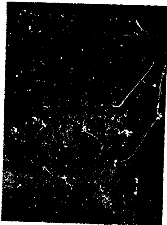
Magnification: 1000X
