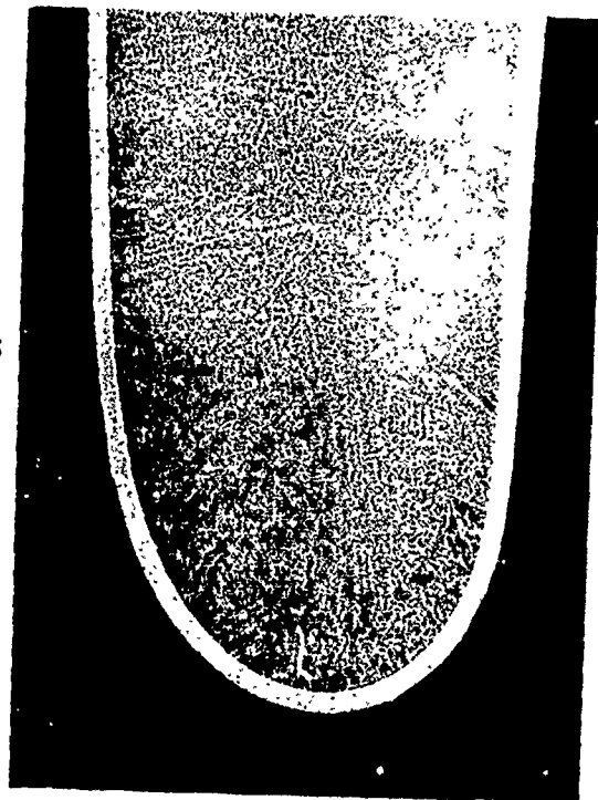
Magnification: 40X
