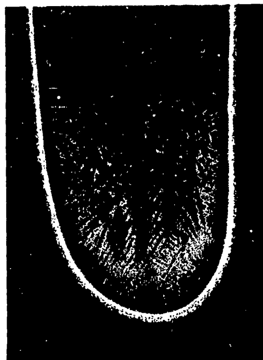
Magnification: 40X
