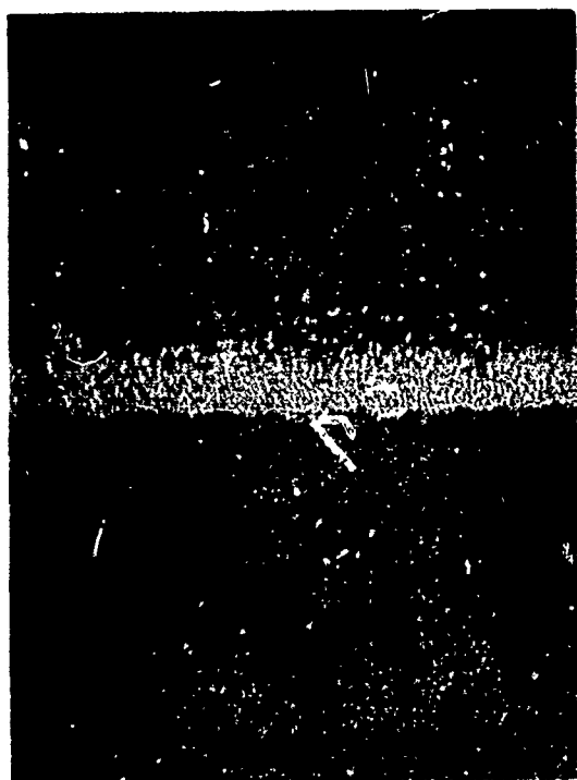
Magnification: 1000X
