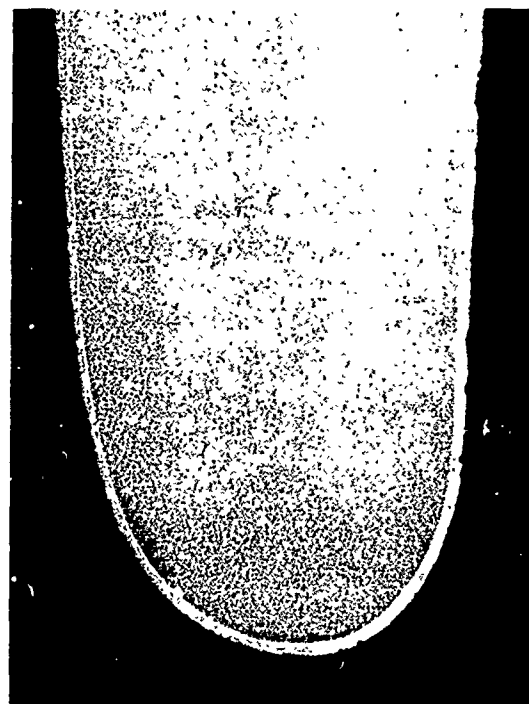
Magnification: 40X
