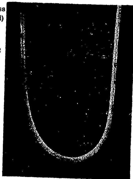
Magnification: 40X
