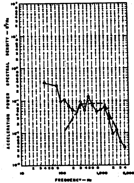
ACCELEROMETER - XI
