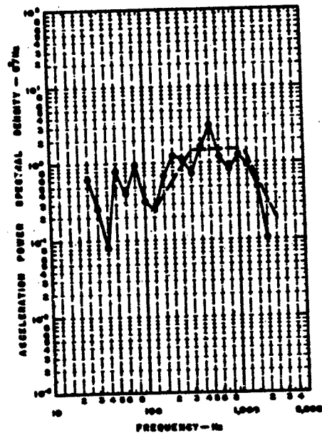
ACCELEROMETER 8-2
