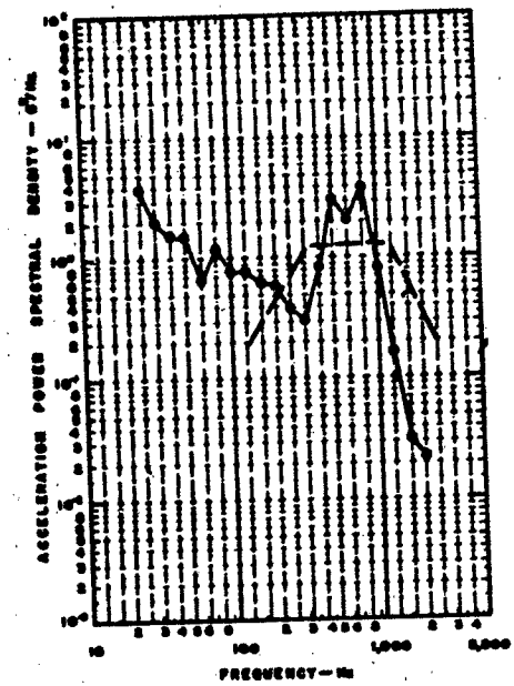
ACCELEROMETER 8-7
