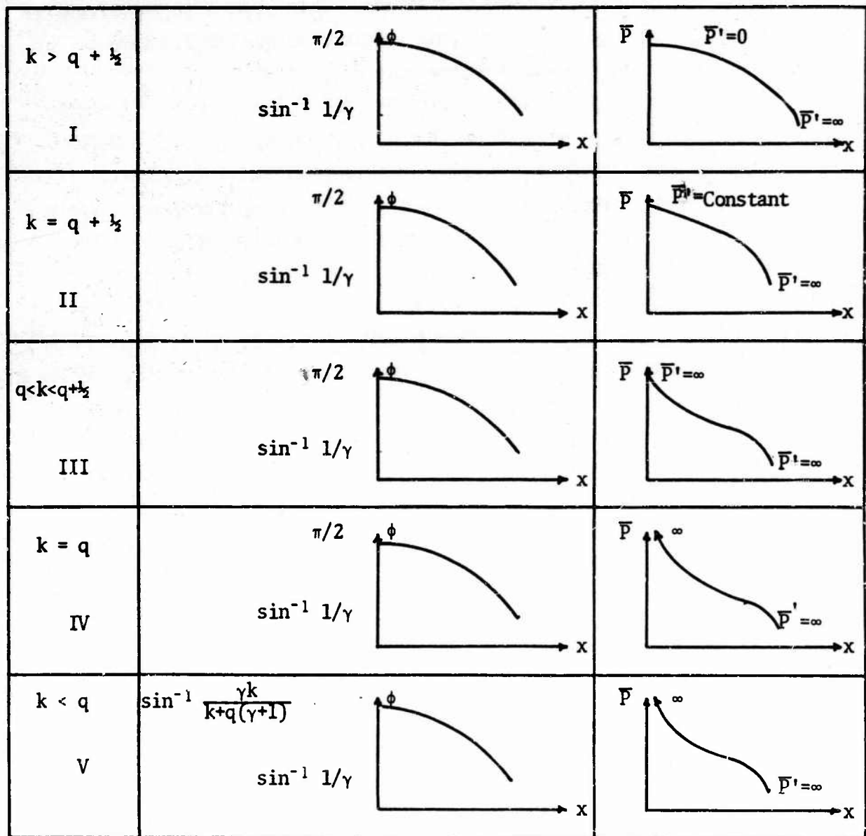
Figure 5. \phi versus x and \bar{P} versus x for various k and q relations
