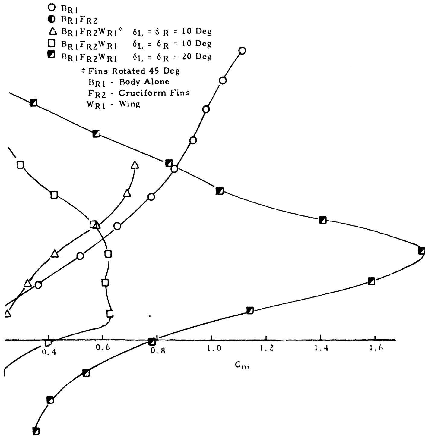
Figure 65. Pitching Moment Characteristics of RT0 Bomblet Model as Determined from AEDC Static Wind Tunnel Tests
