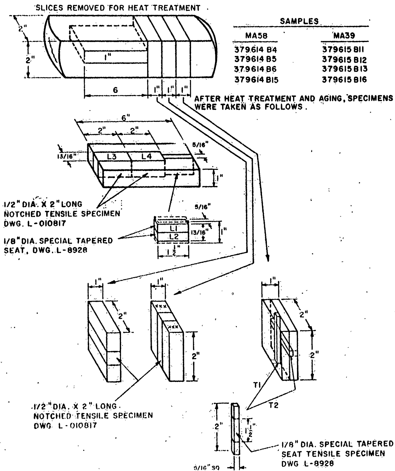
SAMPLING OF 2" SQUARE FORGED BAR
