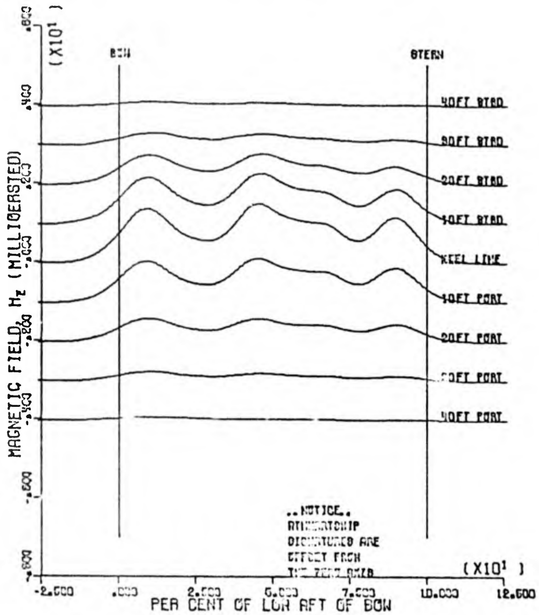
FIG. 14 EXAMPLE OF A DATA MATRIX PLOTTED AS LONGITUDINAL CURVES
