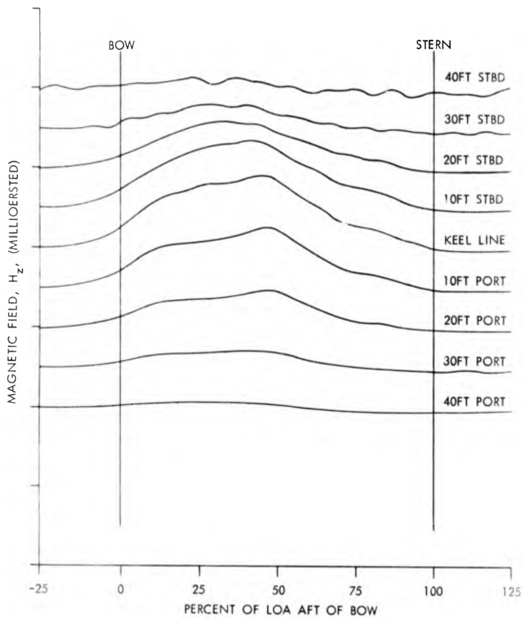
FIG. 16 ORIGINAL DATA PRIOR TO SMOOTHING
