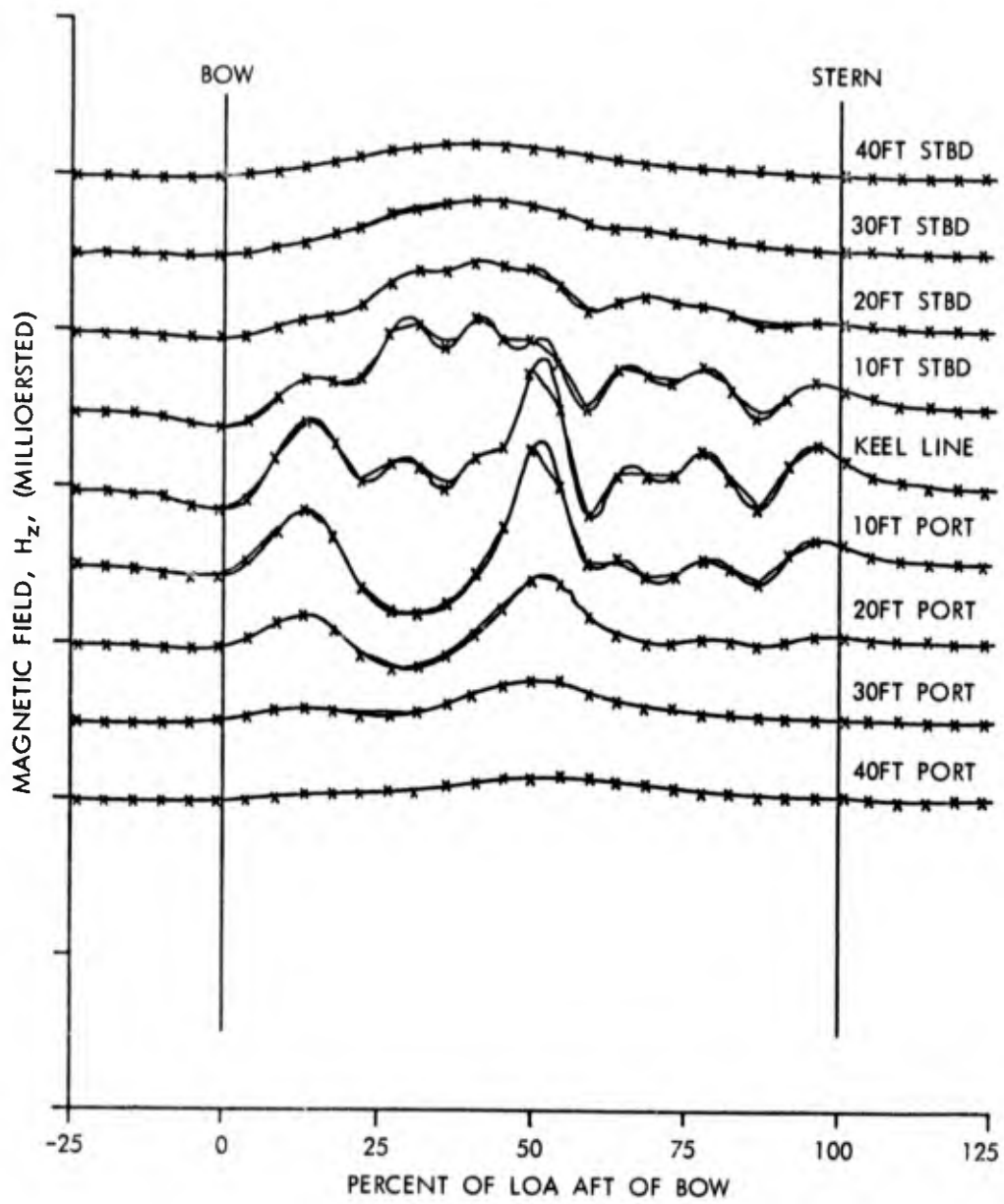
FIG. 18 EXAMPLE OF NUMERICAL INTERPOLATION
