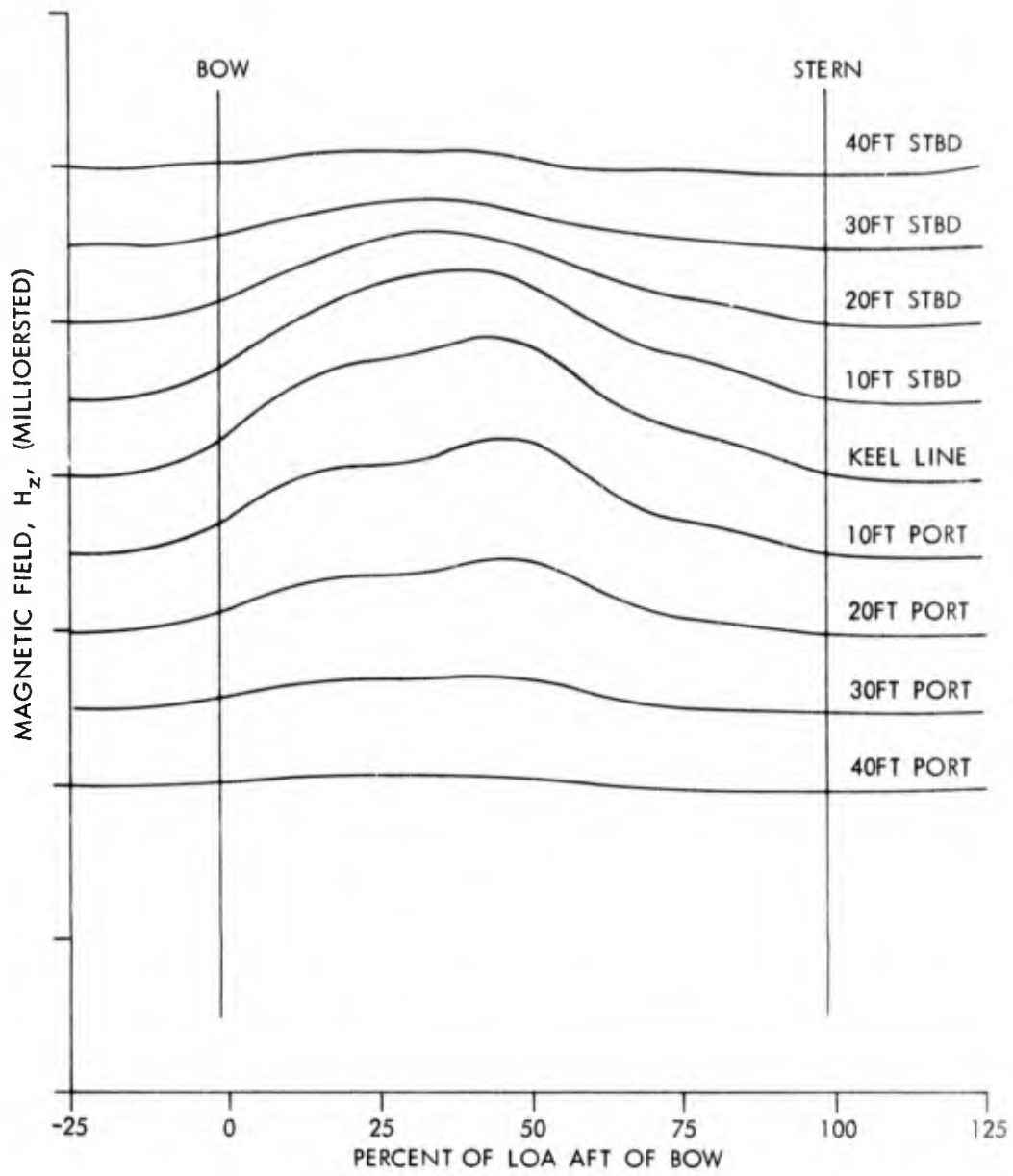
FIG. 17 DATA AFTER SMOOTHING
