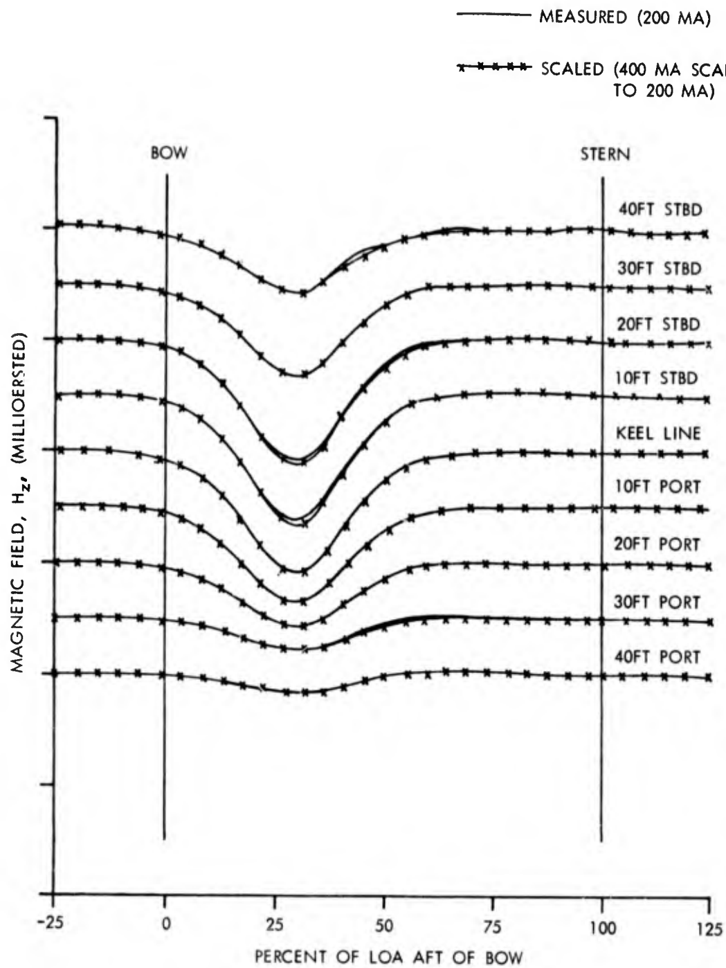
FIG. 20 SCALED COIL EFFECTS
