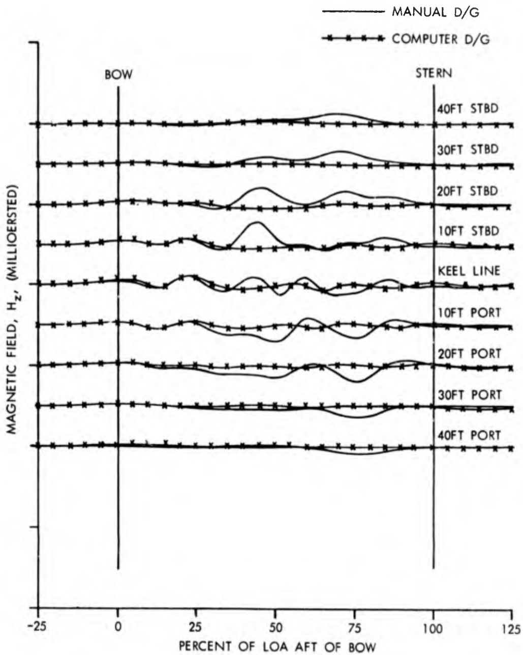
FIG. 19 COMPARISON OF MANUAL AND COMPUTER DEGAUSSING
