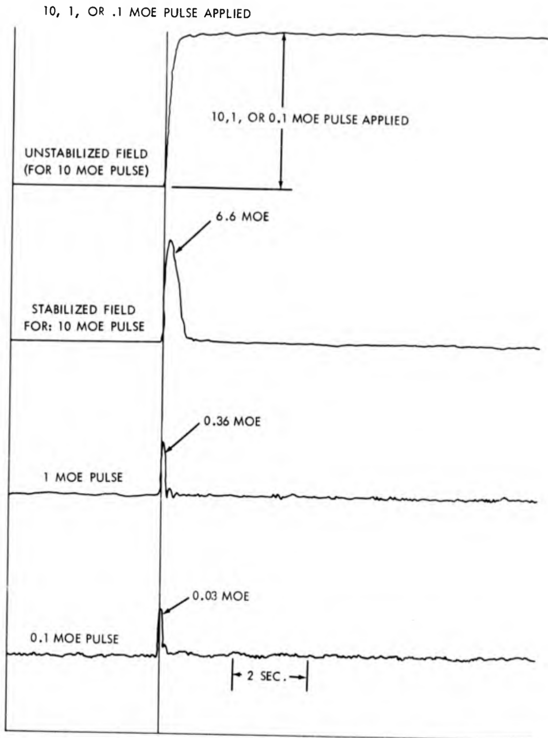
FIG. 11 RESPONSE CURVES FOR Z-CHANNEL OF FEEDBACK STABILIZATION SYSTEM
