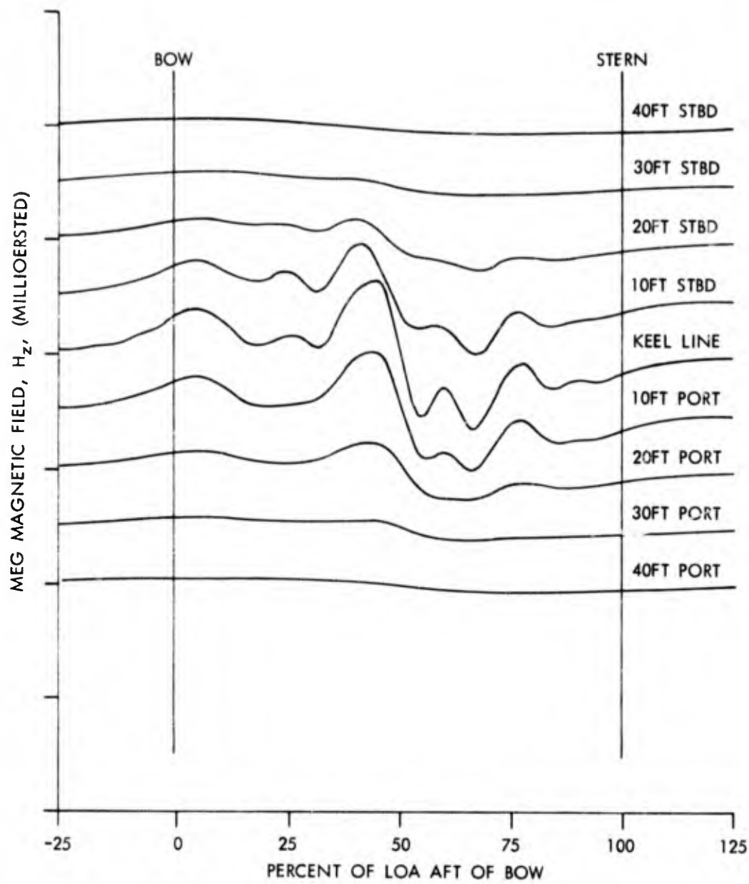
FIG. 22 ORIGINAL DATA PRIOR TO EXTRAPOLATION
