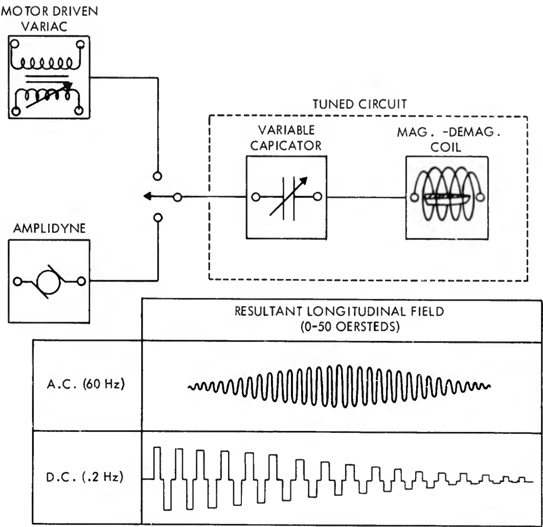
FIG. 7 BLOCK DIAGRAM OF MAGNETIZING AND DEMAGNETIZING SYSTEM
