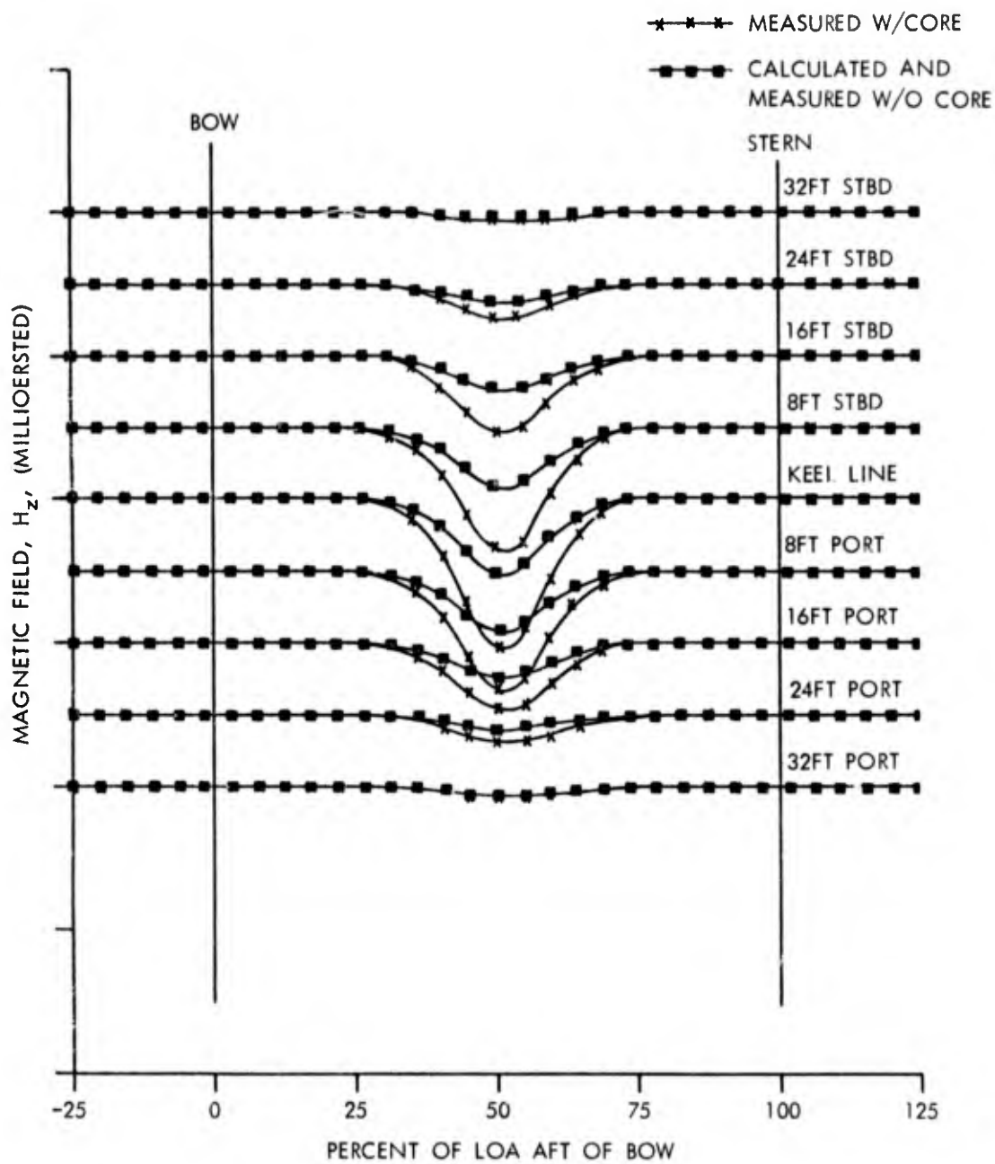
FIG. 21 CALCULATED COIL EFFECTS
