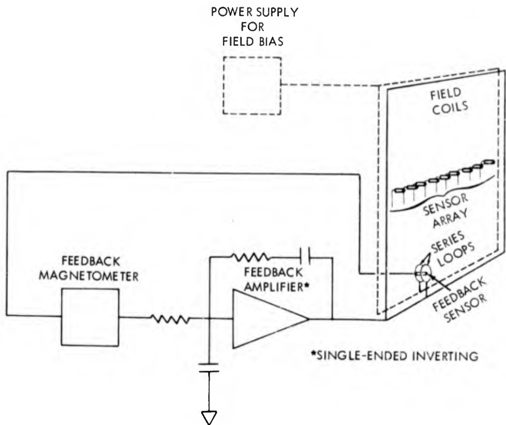
FIG. 9 BLOCK DIAGRAM OF SINGLE CHANNEL OF THE FEEDBACK STABILIZATION SYSTEM
