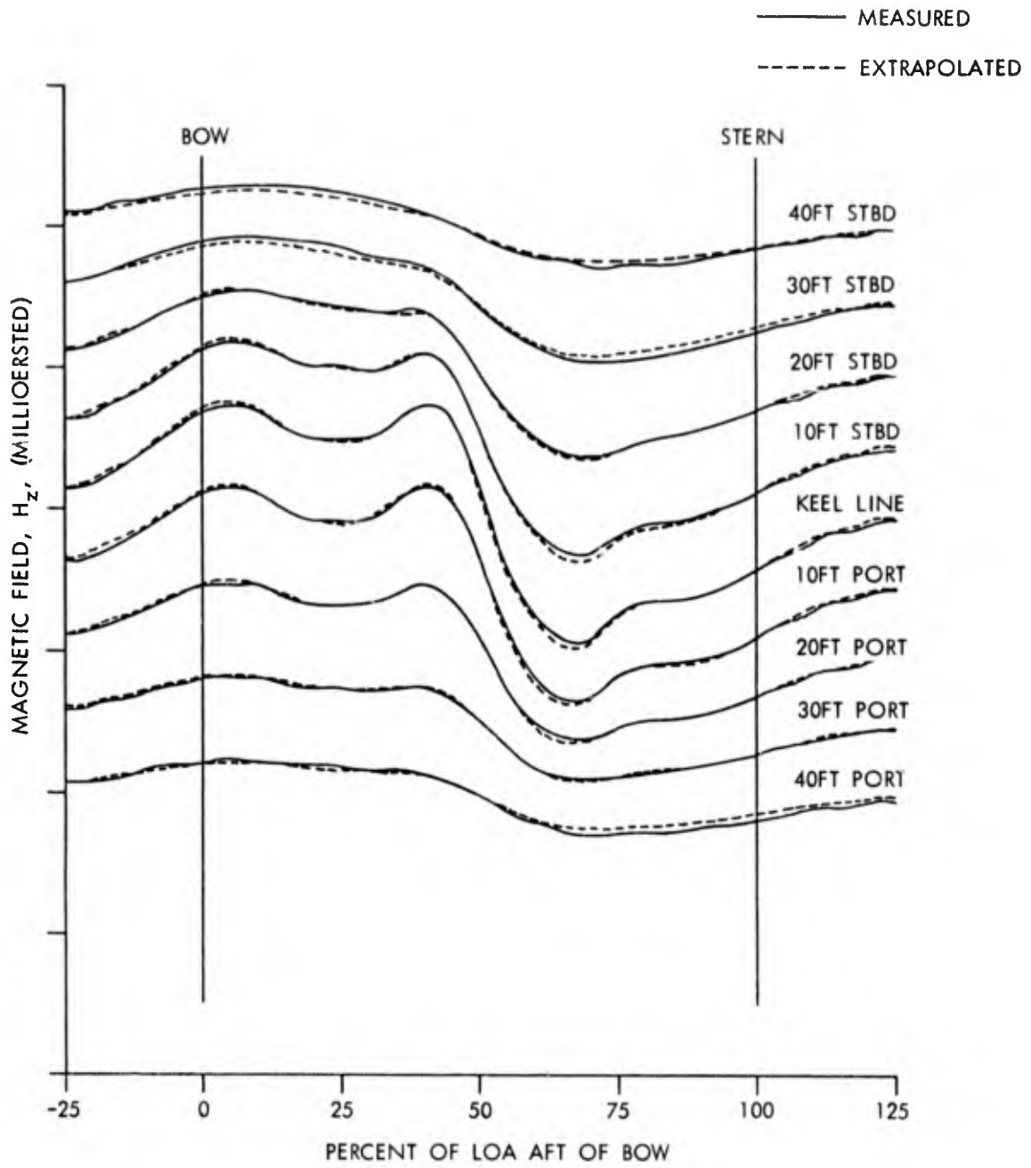
FIG. 23 COMPARISON OF MEASURED DATA WITH EXTRAPOLATED DATA
