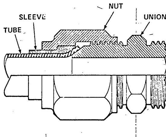
Figure 1. AN Flared Connector
