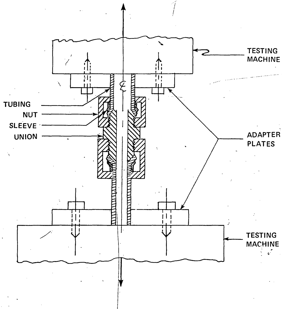
Figure 3. Axial Load Versus Torque Test Setup
