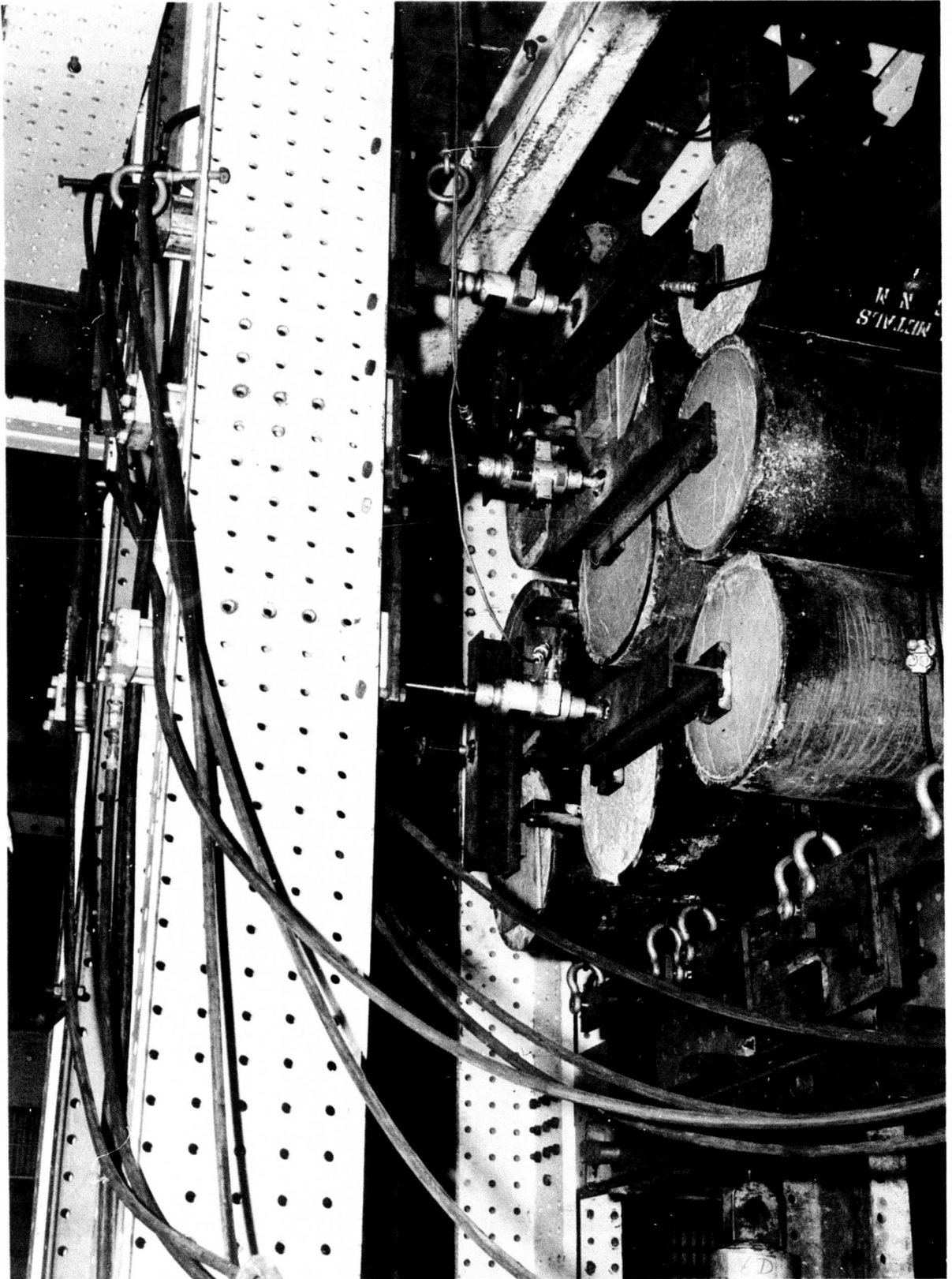
Figure 9. Forward Loads
