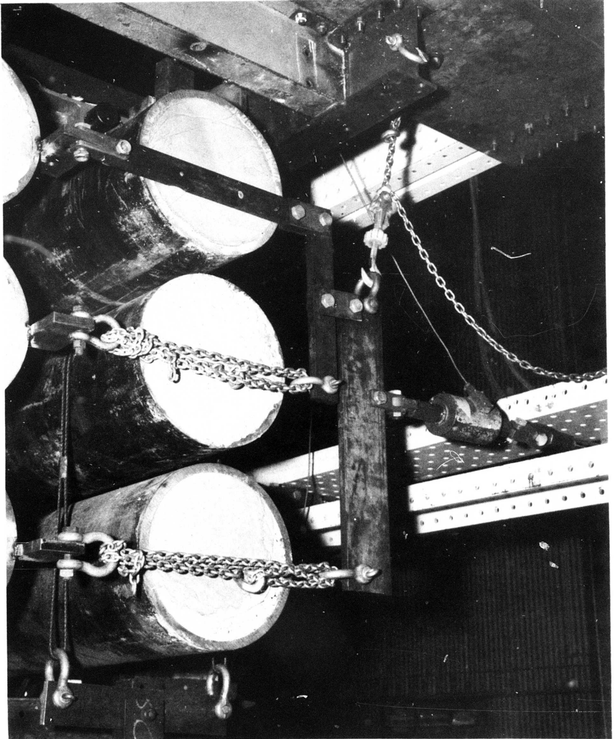
Figure 8. Whiffletree
