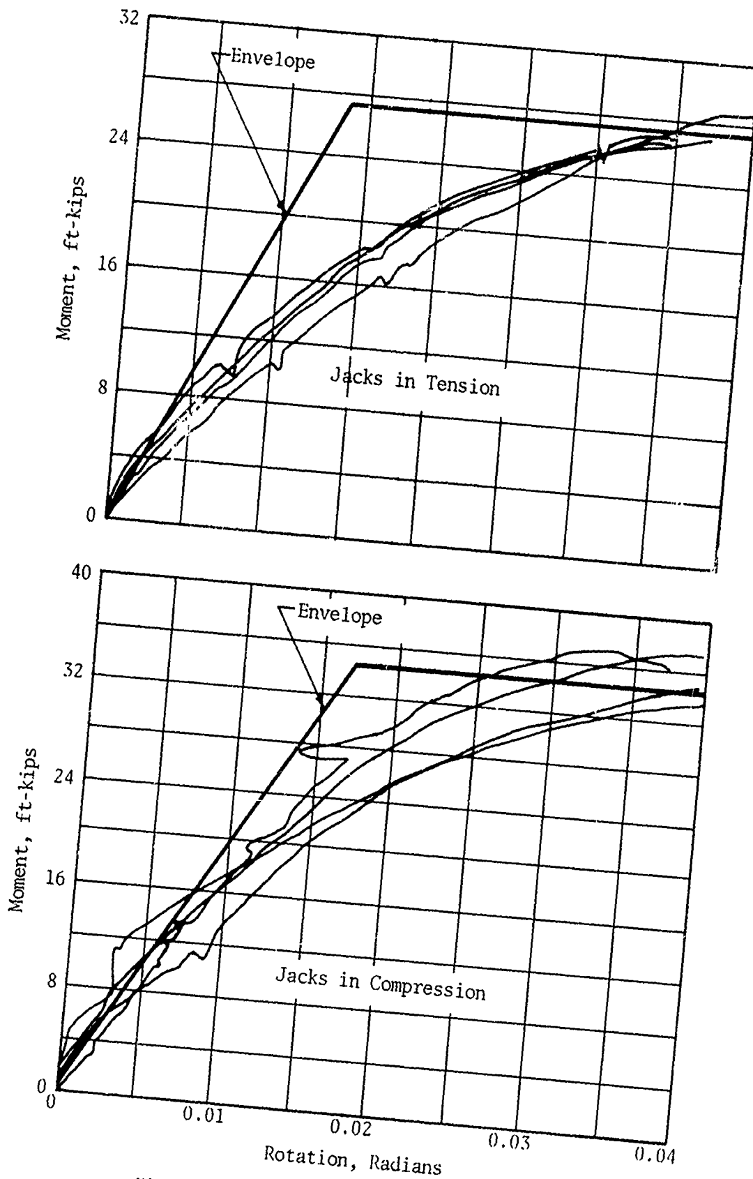
Figure 8. Moment-Rotation Curves
