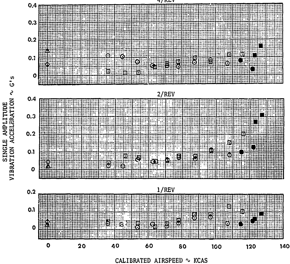
BULKHEAD F.S. 23.00 VERTICAL 4/REV
