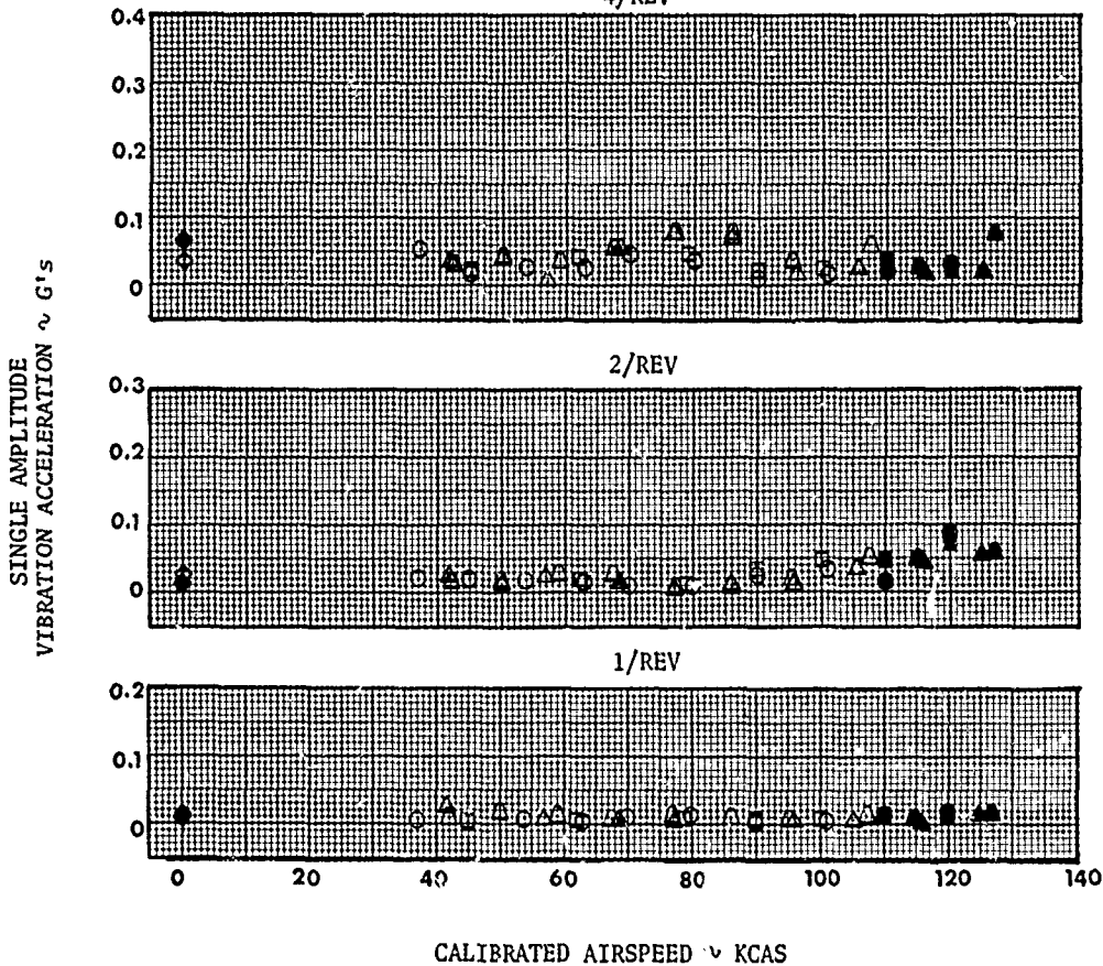
BULKHEAD F.S. 23.00 LONGITUDINAL 4/REV
