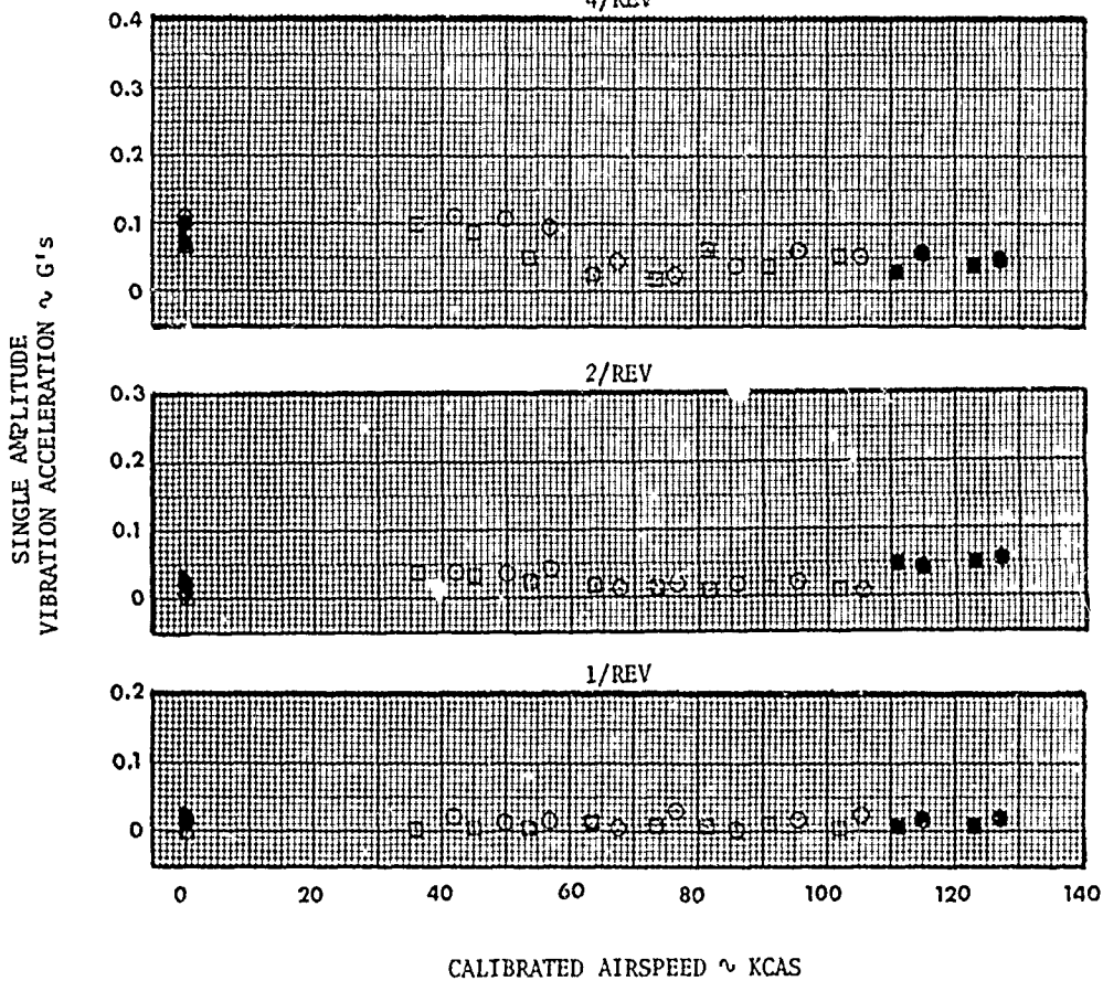
BULKHEAD F.S. 123.00 LATERAL 4/REV
