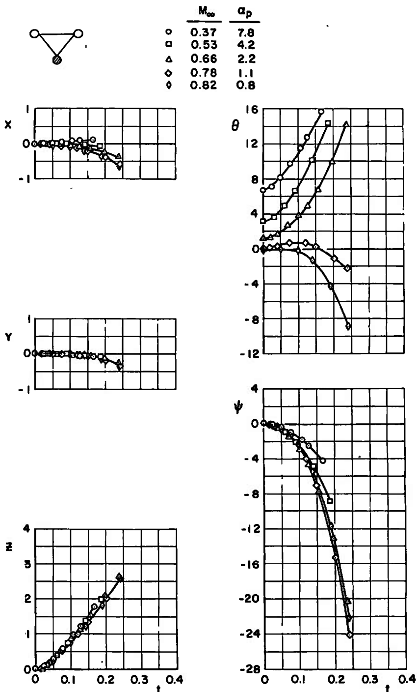
a. Right and Left Wing, Configuration 1C Fig. 13 Effect of Mach Number on the Separation Characteristics of the LAU-68A/A (Full) from the Inboard TER of the F-4C Aircraft, H = 5000 ft
