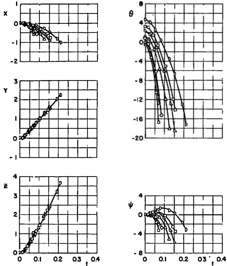
d. Right Wing, Configuration 10E Fig. 16 Continued
