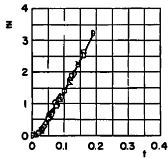
d. Right Wing, Configuration 10C Fig. 14 Continued
