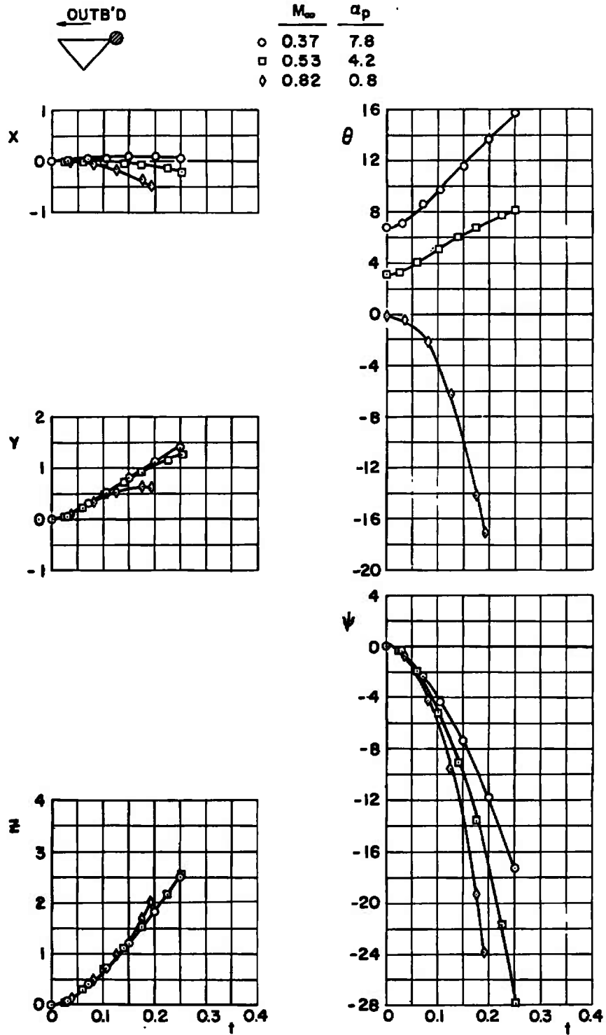
c. Left Wing, Configuration 4E Fig. 15 Continued
