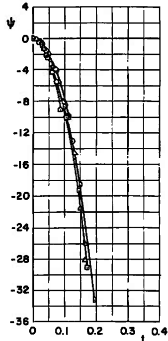
b. Left Wing, Configuration 7E Fig. 16 Continued
