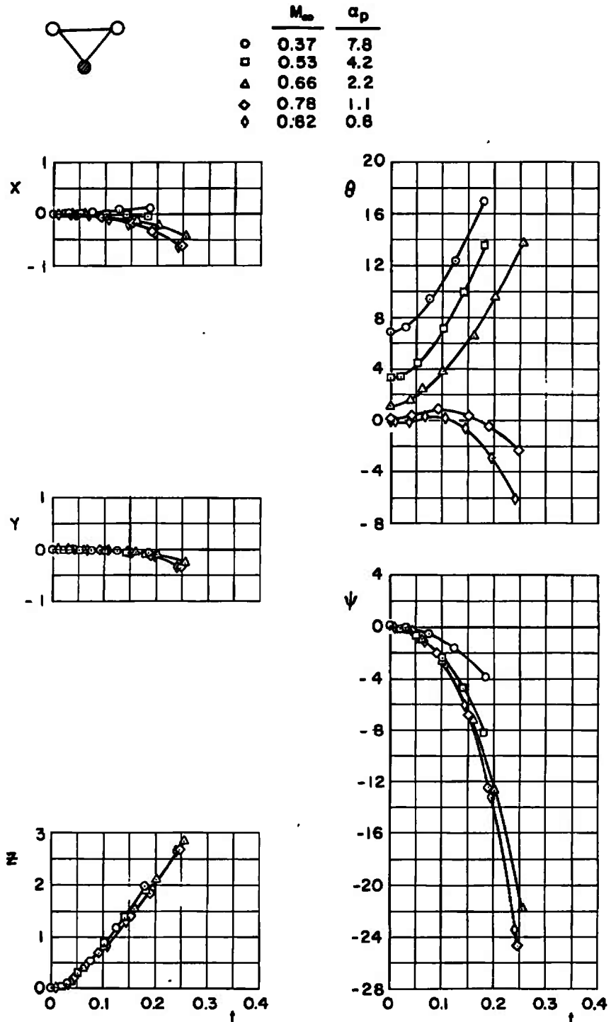
a. Right and Left Wing, Configuration 1E Fig. 15 Effect of Mach Number on the Separation Characteristics of the LAU-68A/A (Full) from the Inboard TER of the F-4E Aircraft, H = 5000 ft
