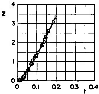
c. Left Wing, Configuration 9E Fig. 16 Continued
