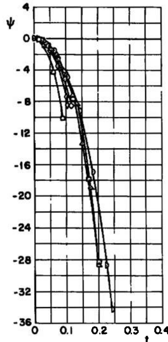
a. Right and Left Wing, Configuration 6C
