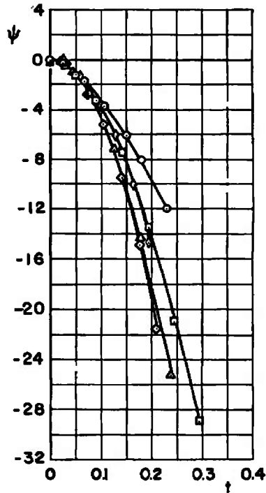
d. Right Wing, Configuration 5C Fig. 13 Continued
