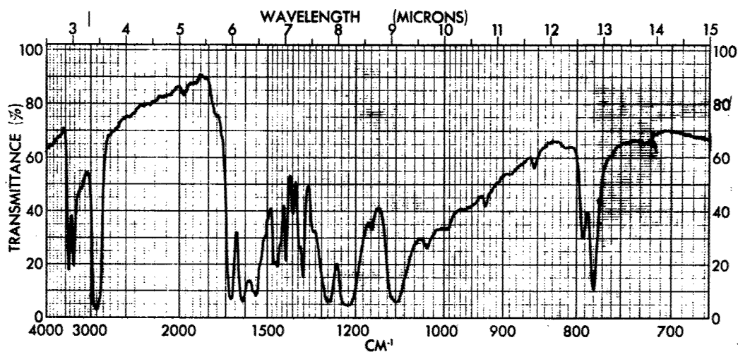
Figure 9 - Infrared Spectrum of Diethyl 2,5-Diimino-1,4-cyclohexanedicarboxylate (Nujol)
