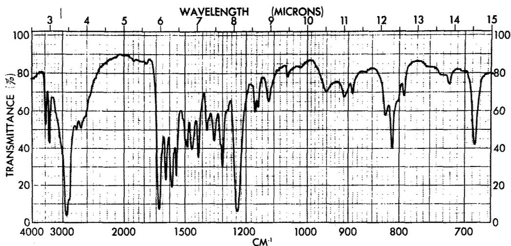
Figure 1 - Infrared Spectrum of the Benzidine 3,3'-Dicarboxylic Acid Sample (Nujol)
