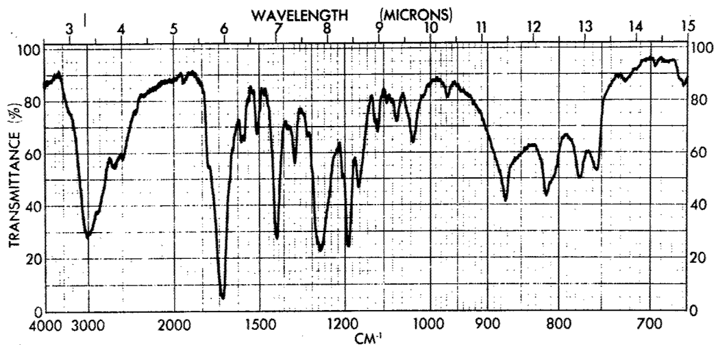
Figure 55 - Infrared Spectrum of NTCA No. 3 (Celanese via LNP 14 October 1970) (KBr)
