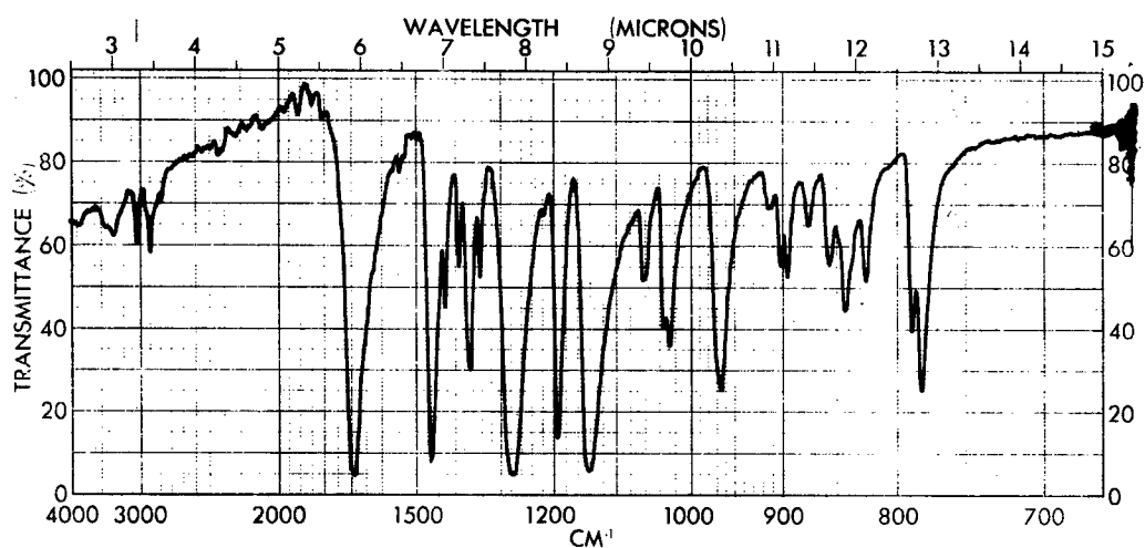
Figure 23 - Infrared Spectrum of 1,1'-Bis(methoxycarbonyl)ferrocene (KBr)
