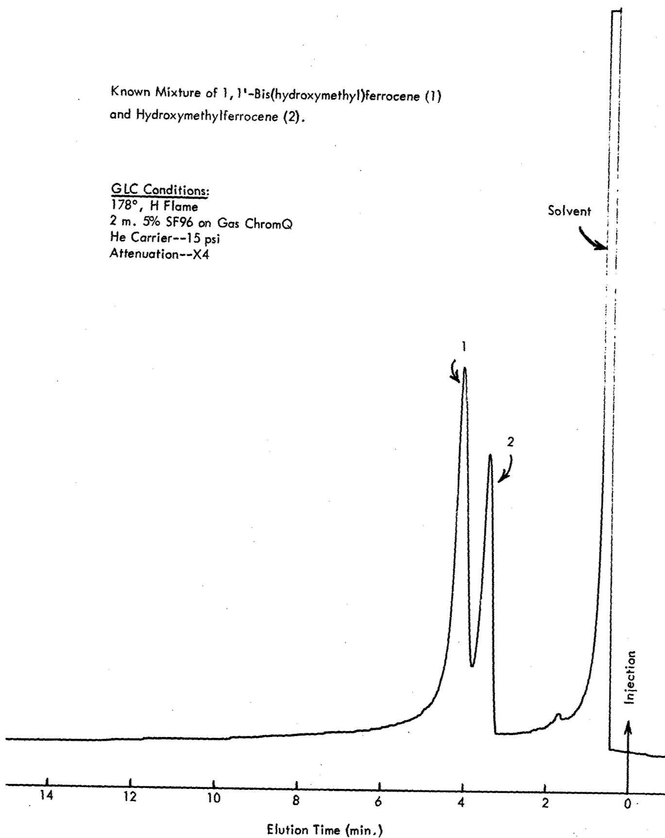
Figure 29 - Gas Liquid Chromatogram of a Mixture of Hydroxymethyl- ferrocene and 1,1'-Bis(hydroxymethyl)ferrocene
