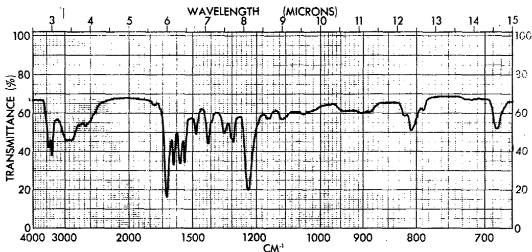
Figure 2 - Infrared Spectrum of Benzidine 3,3'-Dicarboxylic Acid Derived from the Commercial Material (KBr)
