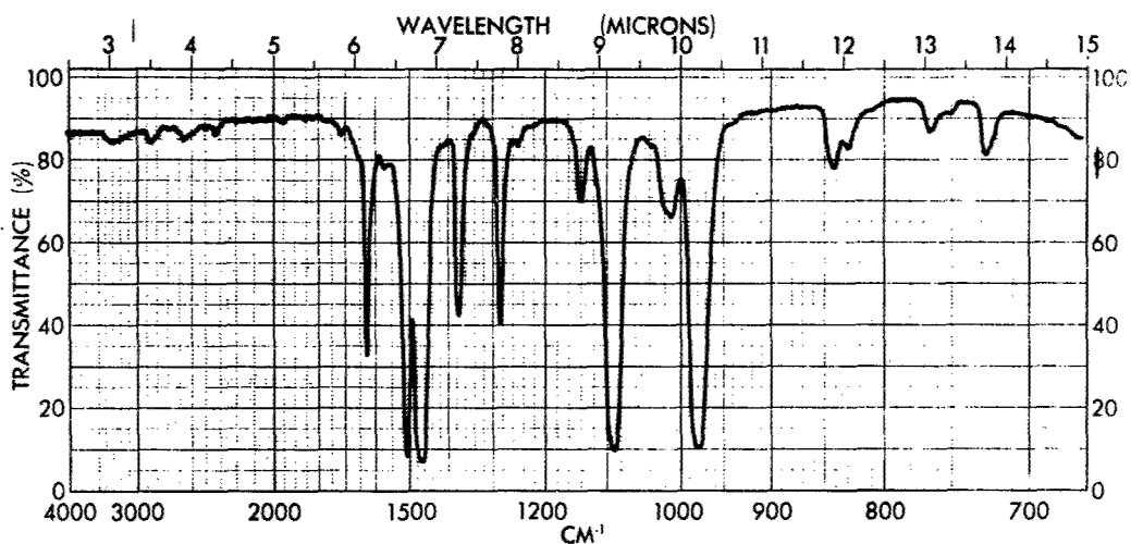
Figure 13 - Infrared Spectrum of Bis(pentafluorophenyl)phosphinous Bromide--Twice Distilled (Liquid)
