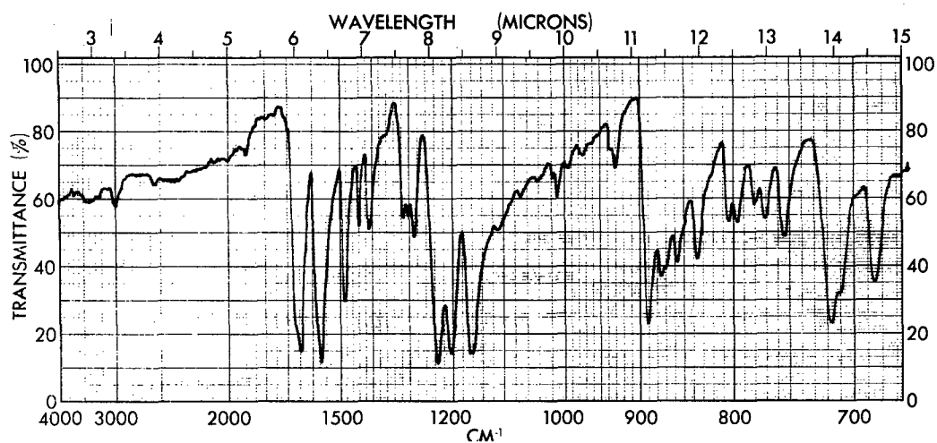
Figure 81 - Infrared Spectrum of p,p' -Oxydibenzil (KBr)
