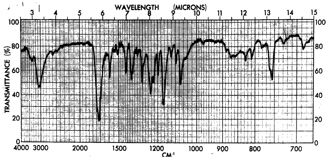
Figure 52 - Infrared Spectrum of NTCA No. 1 (Beaufort Chemical Company) (KBr)
