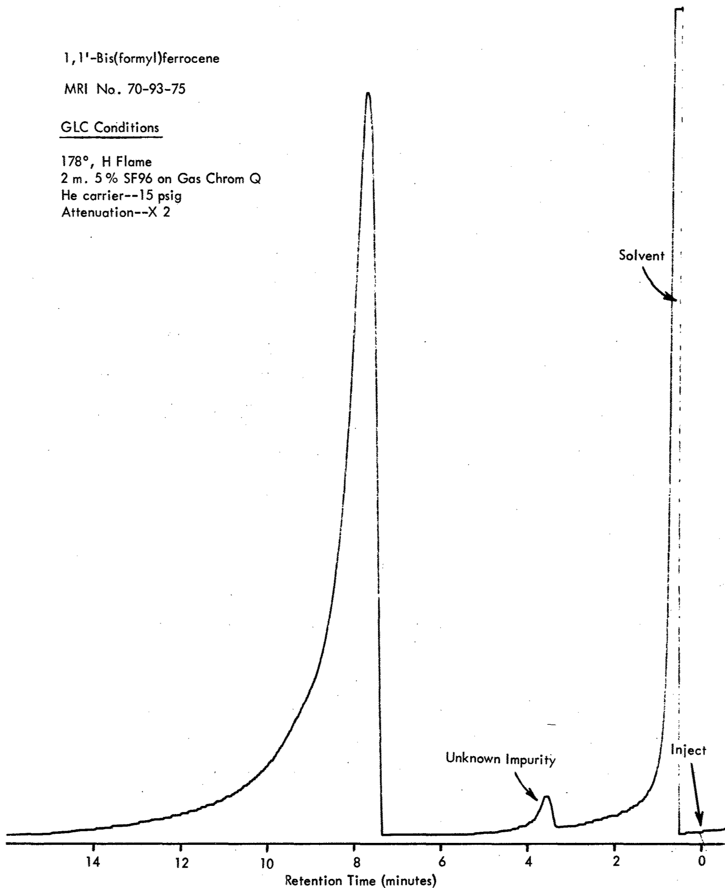
Figure 51 - GLC Chromatogram of 1,1'-Bis(formyl)ferrocene (Sample No. 3)
