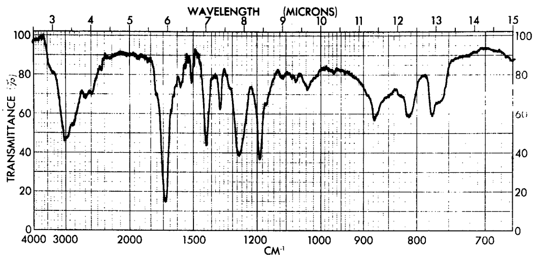
Figure 66 - Infrared Spectrum of NTCA No. 11 (Used in Polymerization No. 70-6) (KBr)
