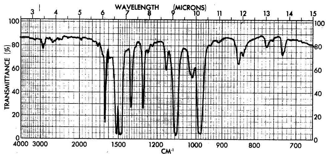
Figure 12 - Infrared Spectrum of Bis(pentafluorophenyl)phosphinous Bromide (Liquid)
