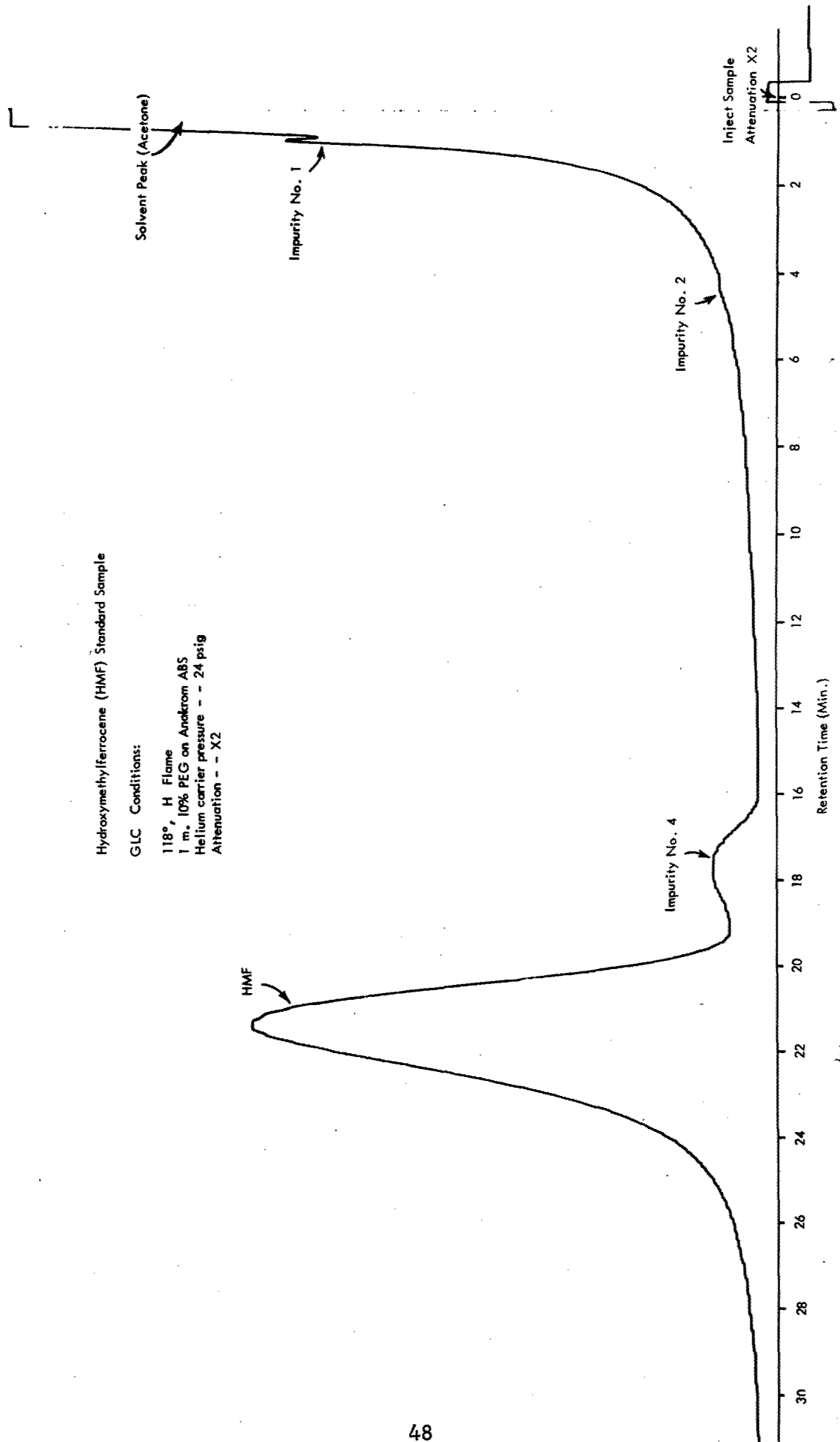
Figure 19 - GLC Chromatogram of Hydroxymethylferrocene (Standard Sample)
