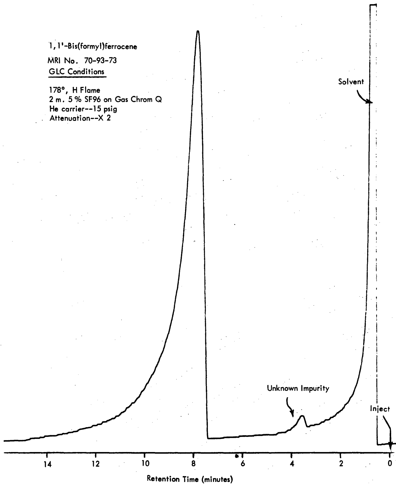
Figure 50 - GLC Chromatogram of 1,1'-Bis(formyl)ferrocene (Sample No. 2)
