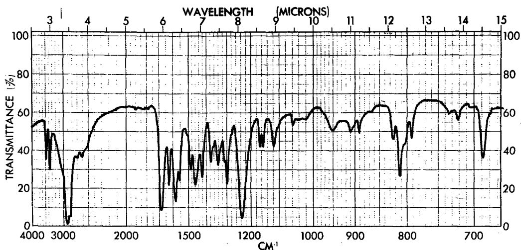
Figure 4 - Infrared Spectrum of the Second Benzidine 3,3'-Dicarboxylic Acid Sample (Nujol)
