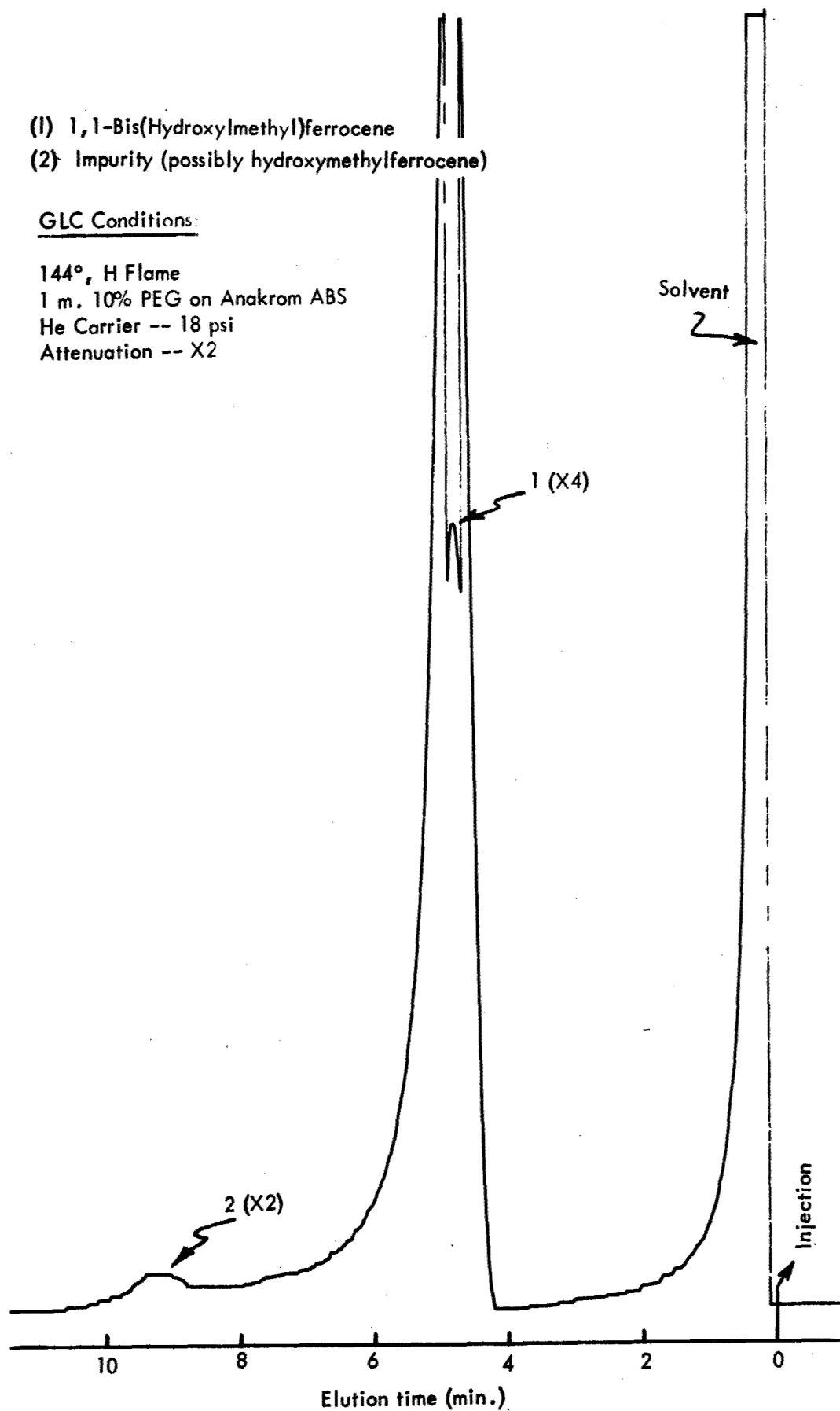
Figure 27 - Gas Liquid Chromatogram of 1,1'-Bis(hydroxymethyl)ferrocene
