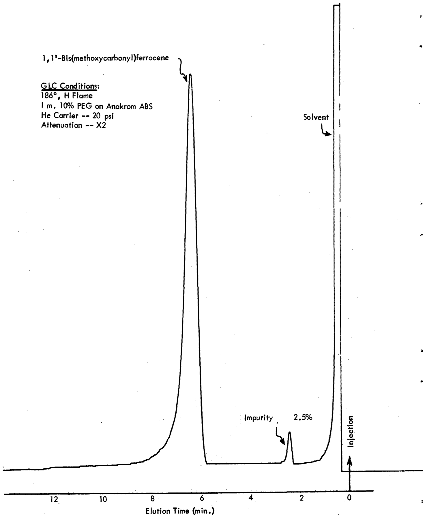
Figure 31 - Gas Liquid Chromatogram of 1,1'-Bis(methoxycarbonyl)ferrocene
