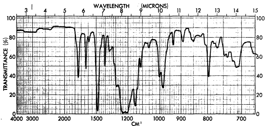
Figure 14 - Infrared Spectrum of 4-Bromoperfluorooctanophenone (Liquid)
