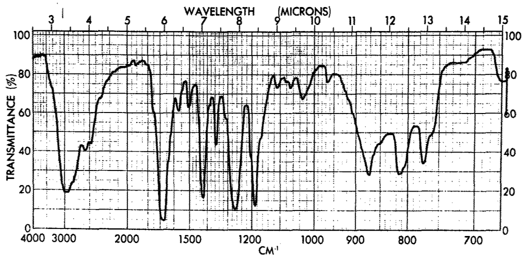
Figure 64 - Infrared Spectrum of NTCA No. 9 (Used in Polymerization 70-4) (KBr)
