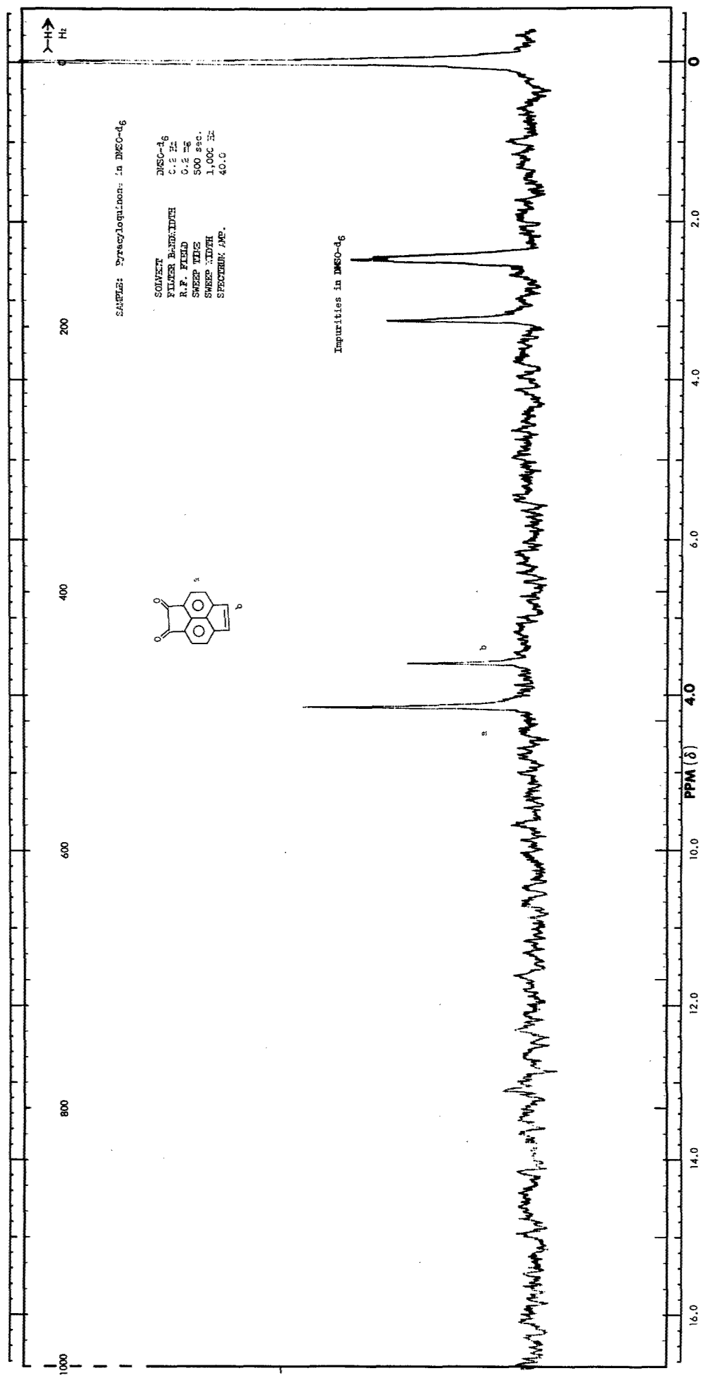
Figure 79 - NMR Spectrum of Piryloquinone
