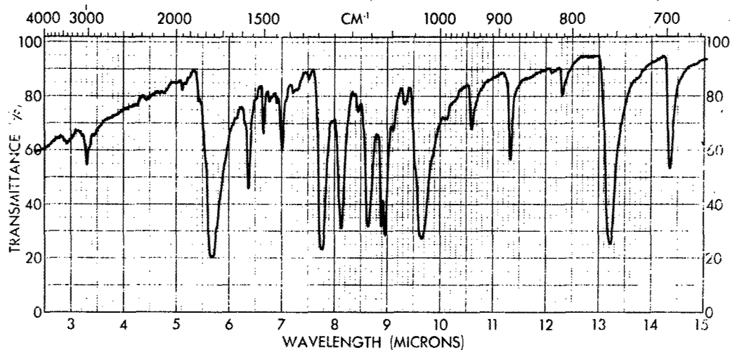
Figure 69 - Infrared Spectrum of Commercial NTDA (Source: Chemical Procurement Labs) (KBr)
