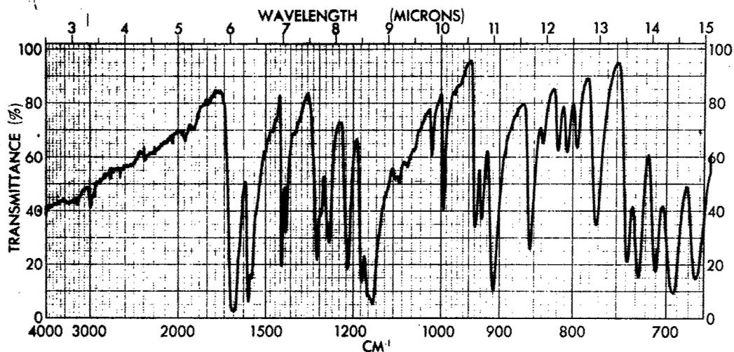
Figure 75 - Infrared Spectrum of 1,3-Bis(phenylglyoxaloyl)benzene (KBr)
