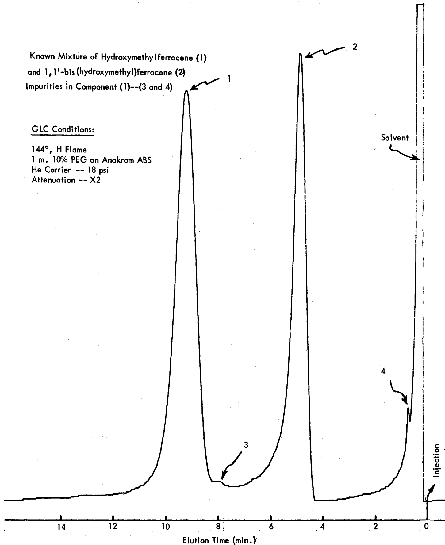
Figure 30 - Gas Liquid Chromatogram of a Mixture of Hydroxymethylferrocene and 1,1'-Bis(hydroxymethyl)ferrocene
