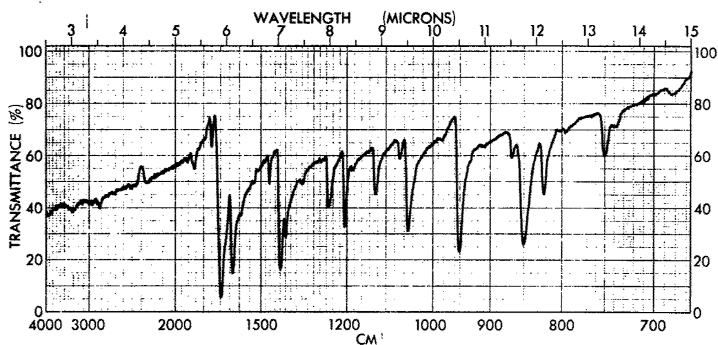
Figure 76 - Infrared Spectrum of Pyracen-1,2-dione (KBr)
