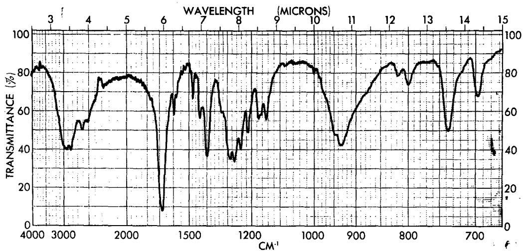
Figure 72 - Infrared Spectrum of m -Phenylenediacetic Acid (KBr)
