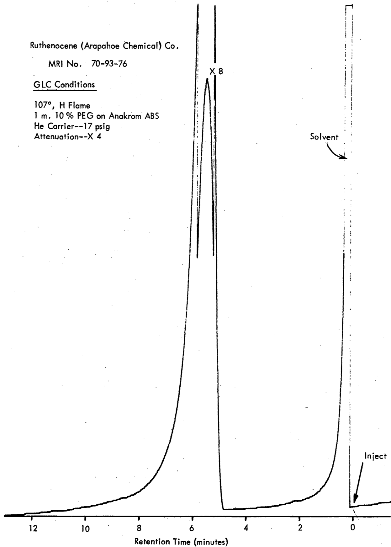
Figure 17 - GLC Chromatogram of Ruthenocene (Arapahoe Chemical Company)
