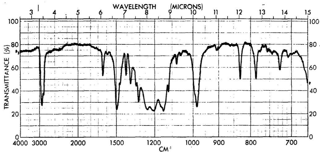
Figure 15 - Infrared Spectrum of Perfluoro-1-bromo-4- n -octylbenzene (Nujol)
