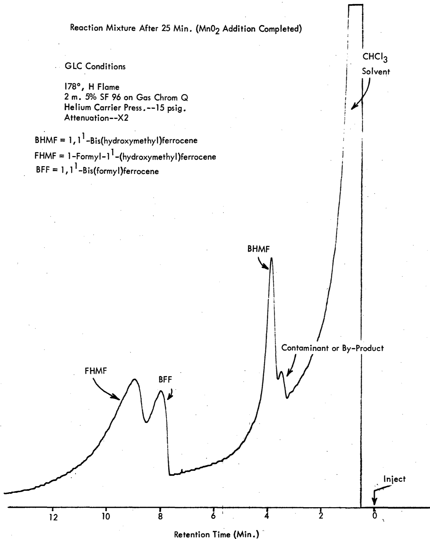
Figure 43 - GLC Chromatogram of 1,1'-Bis(hydroxymethyl)ferrocene Oxidation Mixture After 25 Min. ( \text{MnO}_2 Addition Completed)
