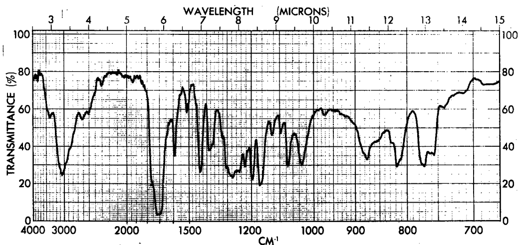
Figure 54 - Infrared Spectrum of NTCA No. 2 (Celanese via LNP 23 September 1969) (KBr)
