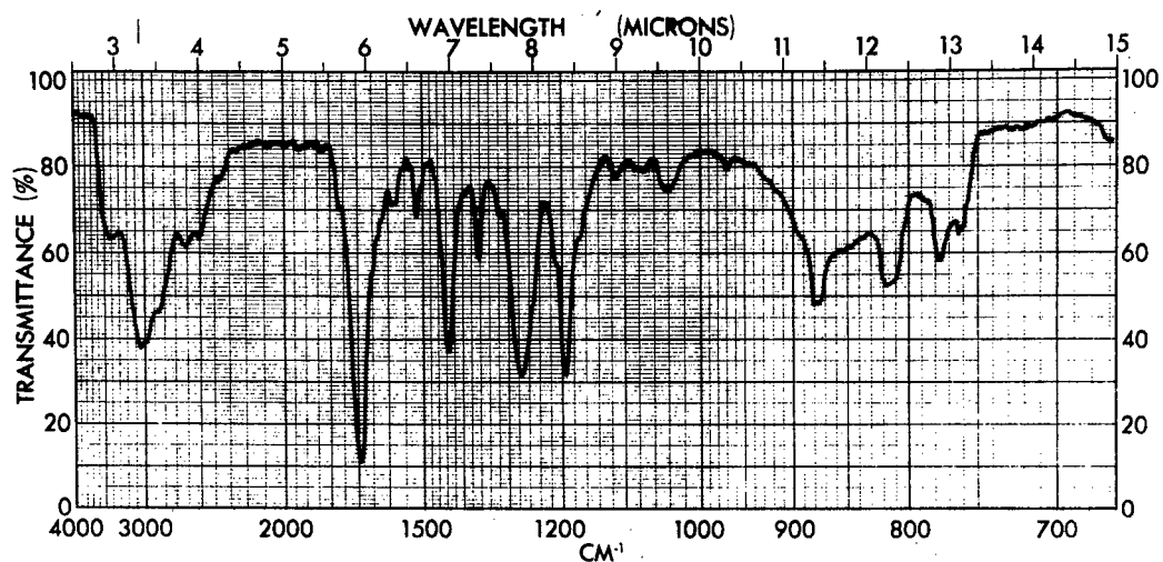
Figure 57 - Infrared Spectrum of NTCA No. 5 (Used in Polymerization 70-1) (KBr)
