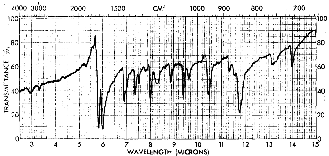
Figure 78 - Infrared Spectrum of Pyracyloquinone (KBr)
