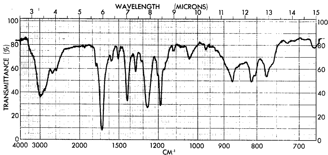
Figure 67 - Infrared Spectrum of NTCA No. 12 (Used in Polymerization No. 70-7) (KBr)
