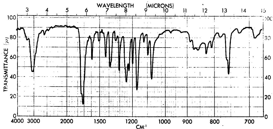
Figure 63 - Infrared Spectrum of NTCA No. 8 (5 g. of NTCA No. 5 After 66 Hr. Treatment with 6N HCl) (Used in Polymerization 70-3) (KBr)
