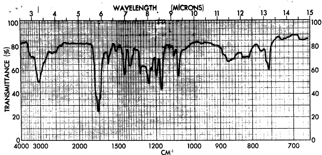
Figure 62 - Infrared Spectrum of NTCA No. 7 (5 g. of NTCA No. 5 Treated 20 Hr. with 6N HCl) (Used in Polymerization 70-2) (KBr)
