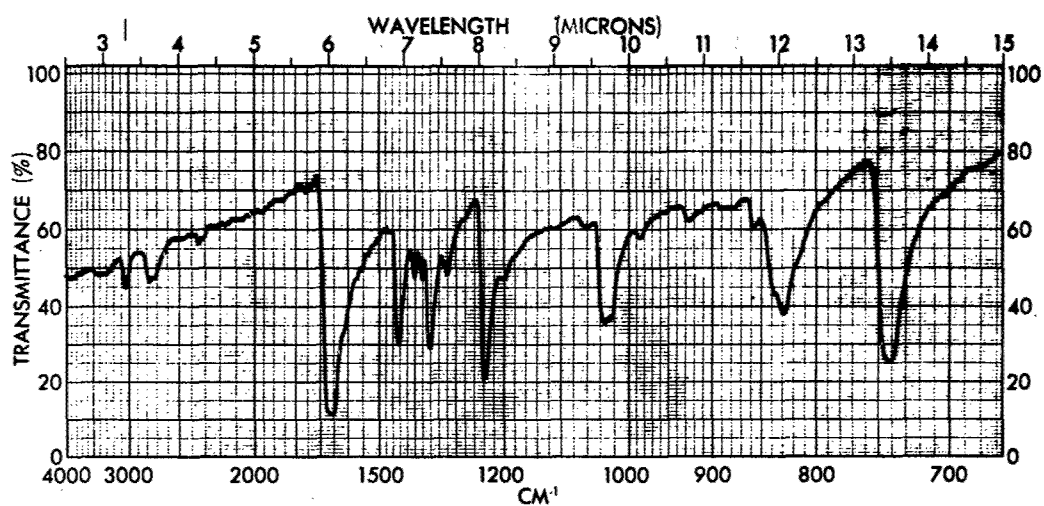
Figure 25 - Infrared Spectrum of 1,1'-Bis(formyl)ferrocene (KBr)
