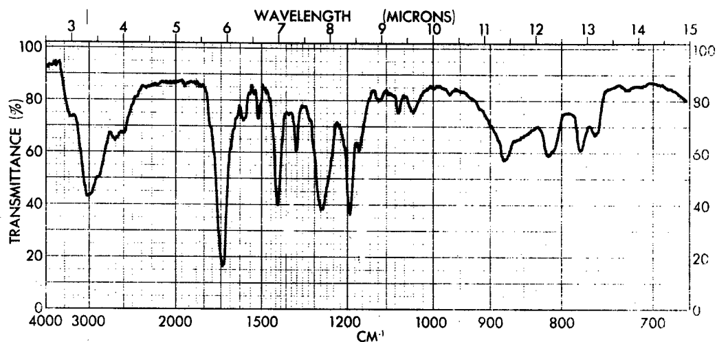
Figure 61 - Infrared Spectrum of NTCA No. 6 (1 g. of NTCA No. 5 Treated 15 Min. with 100 Ml. 12N HCl) (KBr)
