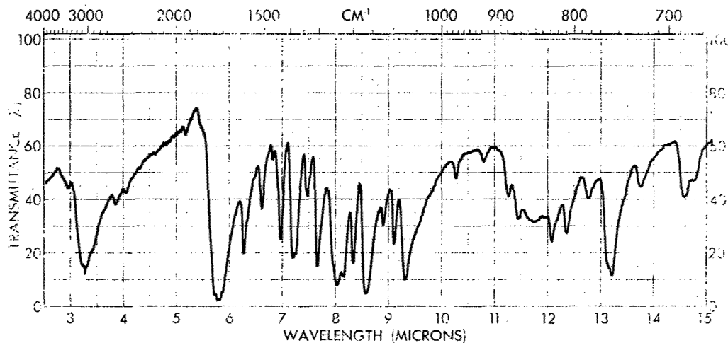
Figure 70 - Infrared Spectrum of Commercial NTDA (Source: K and K Laboratories) (KBr)
