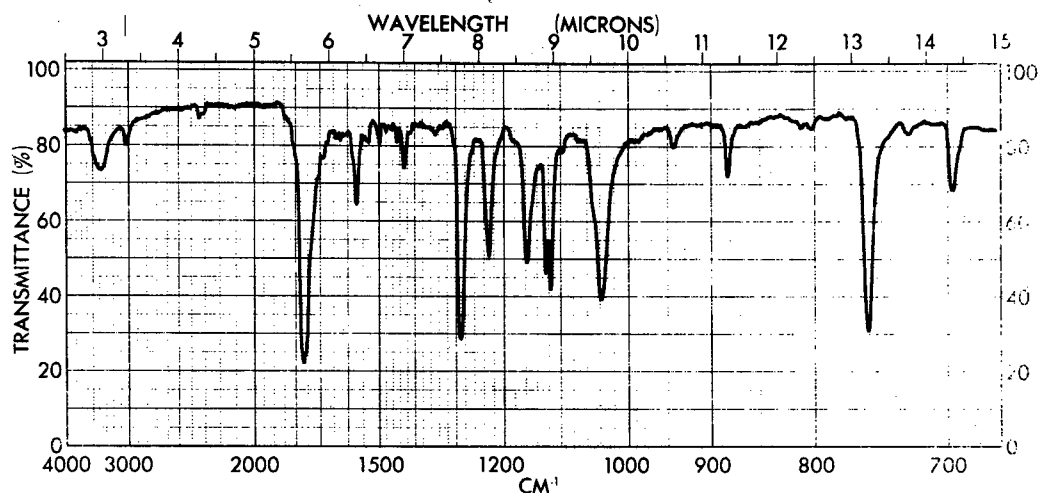
Figure 53 - Infrared Spectrum of NTCA Dianhydride (Produced by Heating NTCA No. 1 on DTA to 300°C) (KBr)
