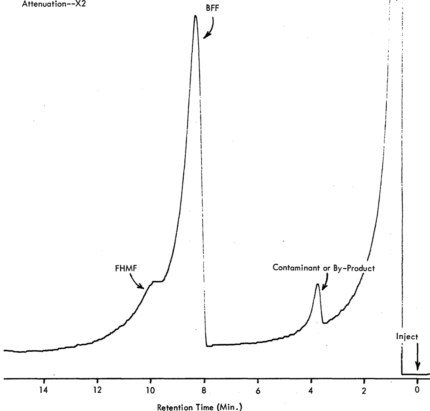
Figure 45 - GLC Chromatogram of 1,1'-Bis(hydroxymethyl)ferrocene Oxidation Mixture After 2 Hr. ( \text{MnO}_2 Added, Heated to Reflux and Refluxed 1 Hr.)
