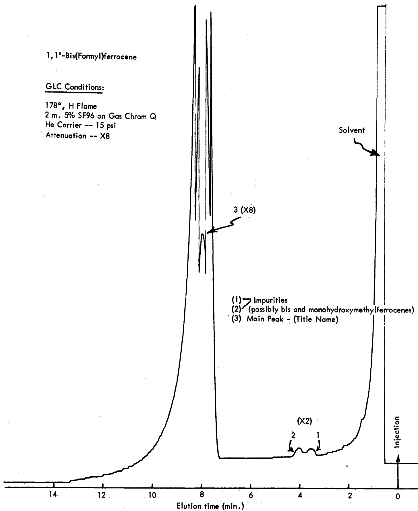
Figure 28 - Gas Liquid Chromatogram of 1,1'-Bis(formyl)ferrocene
