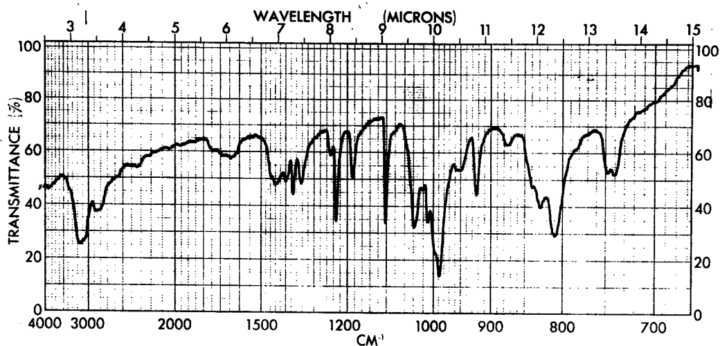
Figure 22 - Infrared Spectrum of Hydroxymethylferrocene (KBr)
