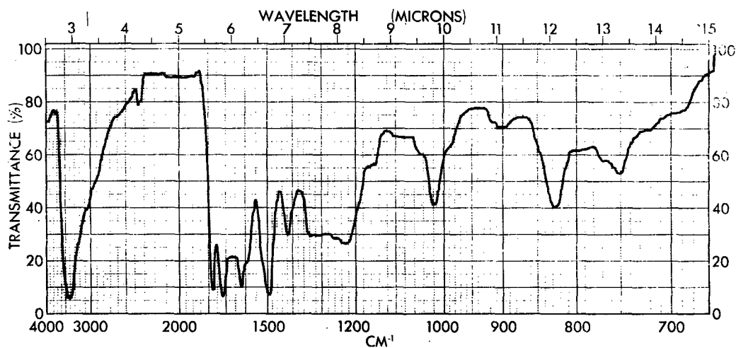
Figure 6 - Infrared Spectrum of Substance Obtained Directly in the "Bisdione" Preparation (KBr)
