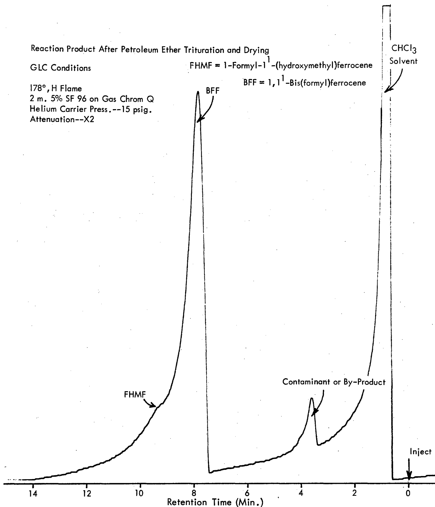
Figure 46 - GLC Chromatogram of 1,1'-Bis(hydroxymethyl)ferrocene Oxidation Product After Petroleum Ether Trituration and Drying
