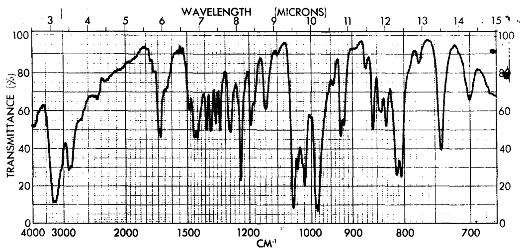
Figure 20 - Infrared Spectrum of 1,1'-Bis(hydroxymethyl)ferrocene (KBr)
