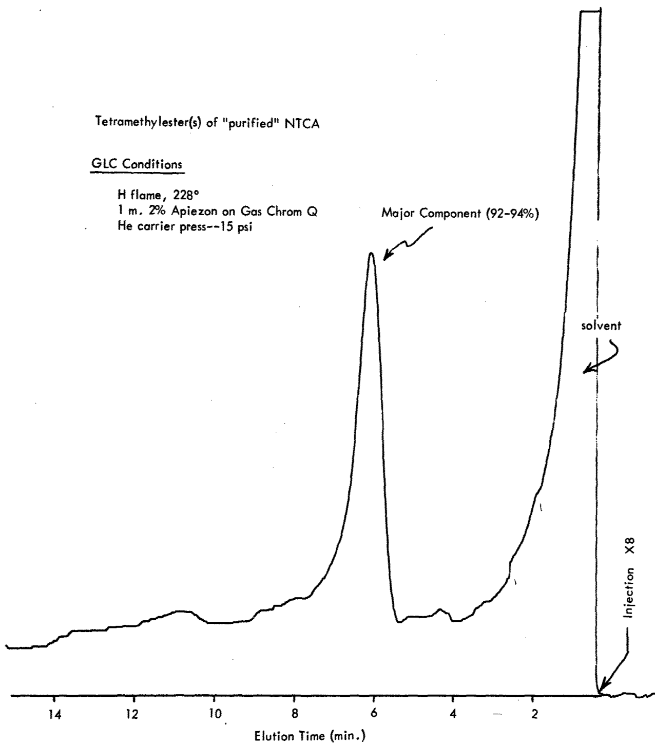
Figure 60 - Gas Liquid Chromatogram of Tetramethyl Ester(s) of NTCA No. 5
