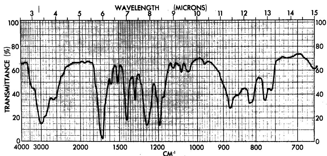
Figure 59 - Infrared Spectrum of NTCA (Produced by Three Successive Oxidation-Decolorization Treatments of the NTCA No. 1) (KBr)
