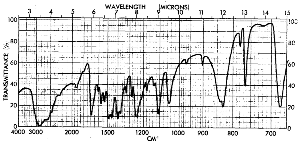
Figure 3 - Infrared Spectrum of Benzidine 3,3'-Dicarboxylic Acid Dihydrochloride Derived from the Commercial Material (Nujol)
