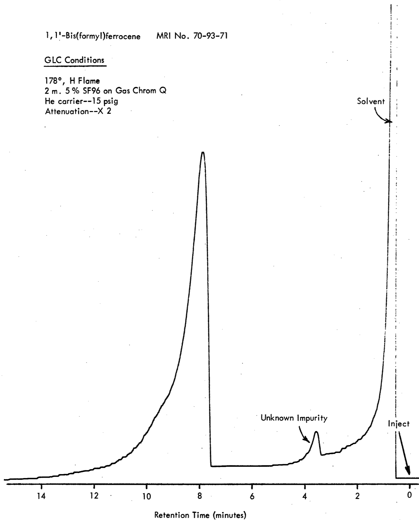
Figure 49 - GLC Chromatogram of 1,1'-Bis(formyl)ferrocene (Sample No. 1)
