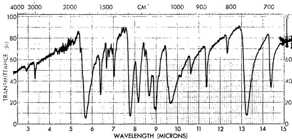
Figure 71 - Infrared Spectrum of NTDA No. 1 (Used in Polymerization No. 71-1) (KBr)
