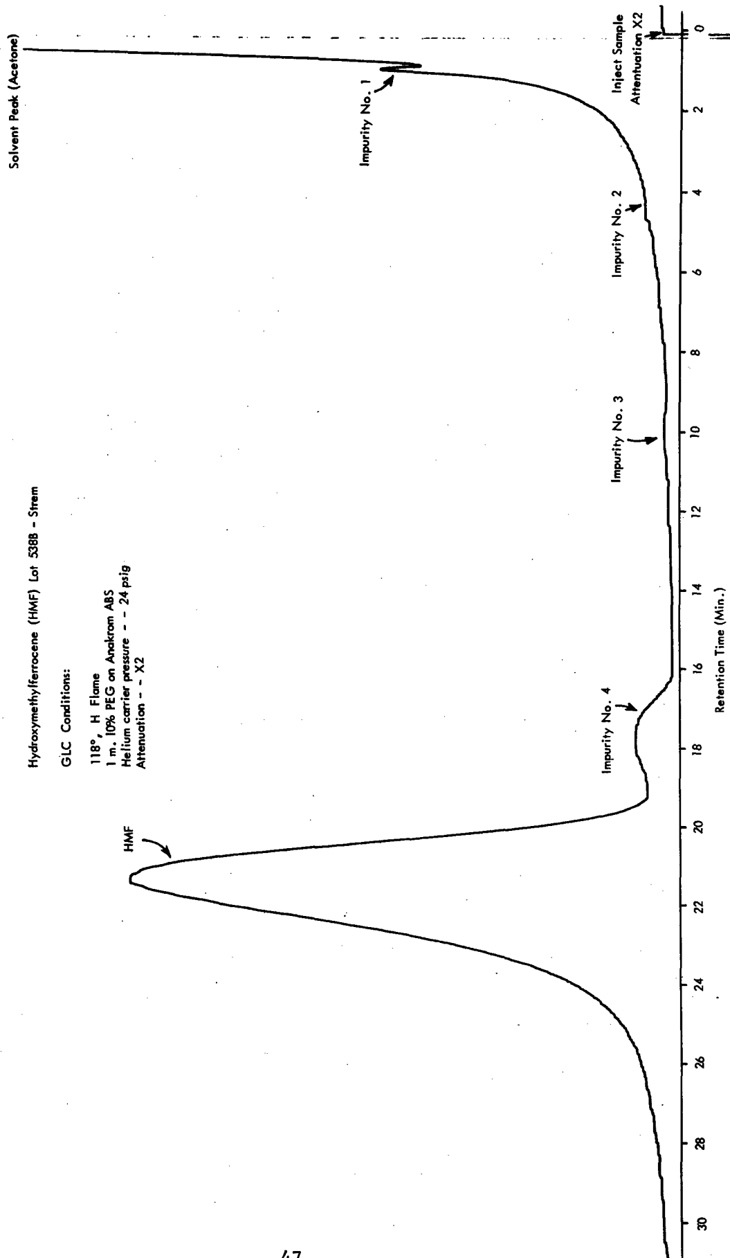
Figure 18 - GLC Chromatogram of Hydroxymethylferrocene (Strem Chemical Company)
