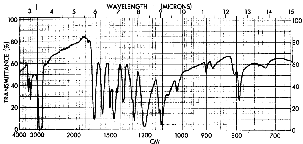
Figure 10 - Infrared Spectrum of the Sample of Diethyl 2,5-Diaminoterephthalate (Nujol)
