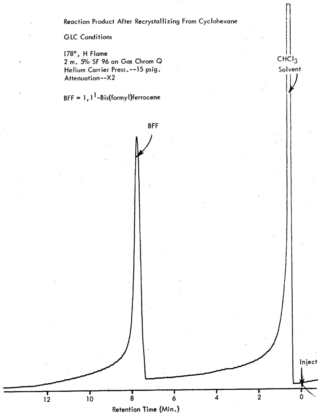
Figure 47 - GLC Chromatogram of 1,1'-Bis(hydroxymethyl)ferrocene Oxidation Product After Recrystallizing from Cyclohexane
