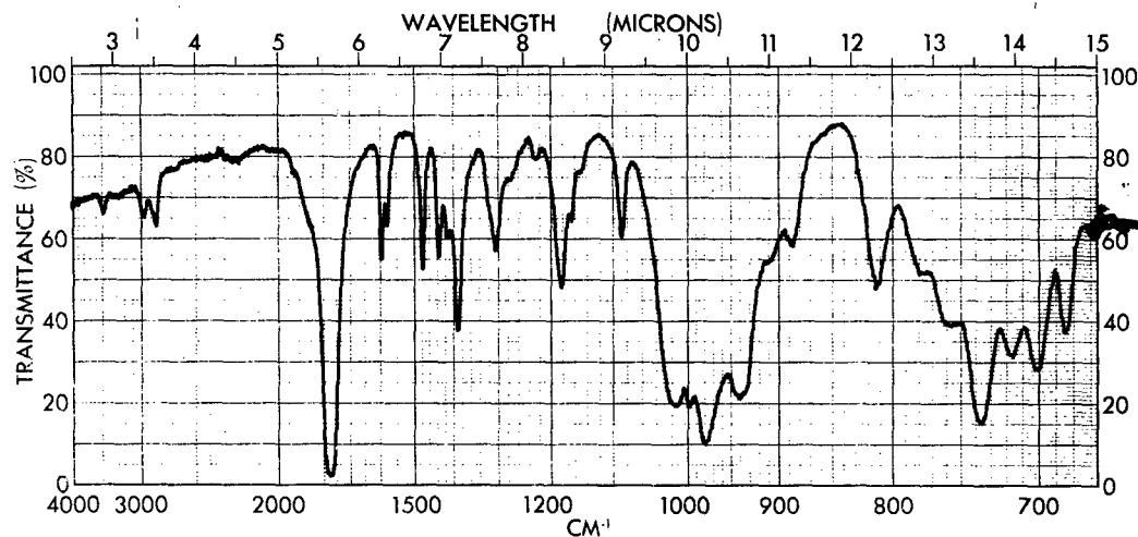
Figure 73 - Infrared Spectrum of m -Phenylenediacetyl Chloride (Liquid)
