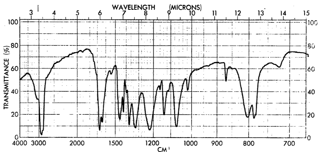
Figure 7 - Infrared Spectrum of the Substance Obtained Directly in the "Bisdione" Preparation from More Highly Purified Benzidine 3,3'-Dicarboxylic Acid (KBr)
