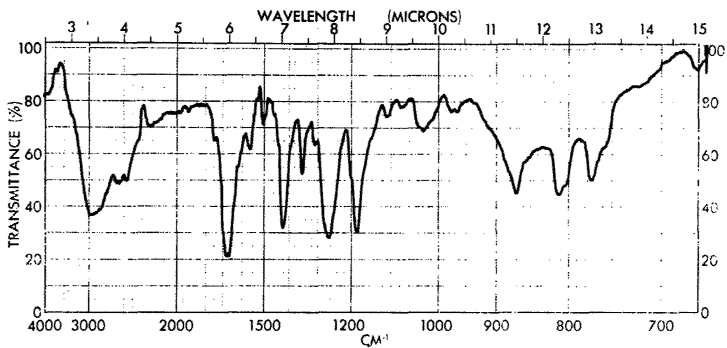
Figure 65 - Infrared Spectrum of NTCA No. 10 (Used in Polymerization 70-5) (KBr)
