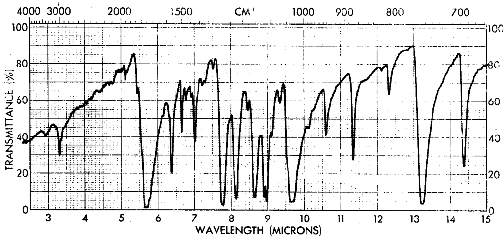
Figure 68 - Infrared Spectrum of Commercial NTDA (Source: Aldrich Chemical Company) (KBr)
