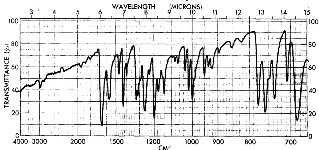
Figure 74 - Infrared Spectrum of 1,3-Bis(phenylacetyl)benzene (KBr)
