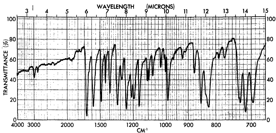
Figure 80 - Infrared Spectrum of p,p' -Di(phenylacetylphenyl)ether (KBr)
