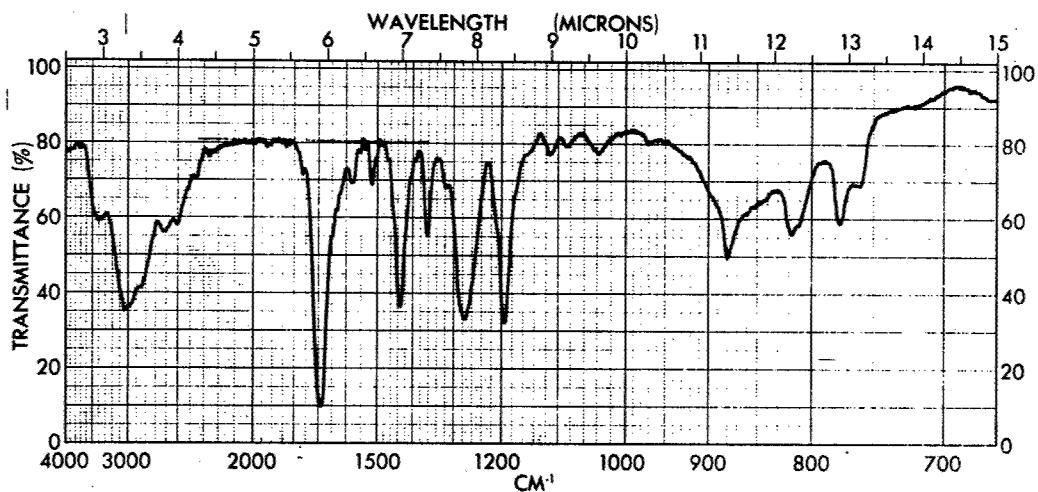
Figure 56 - Infrared Spectrum of NTCA No. 4 (Used in Polymeriza- tion 69-1) (KBr)
