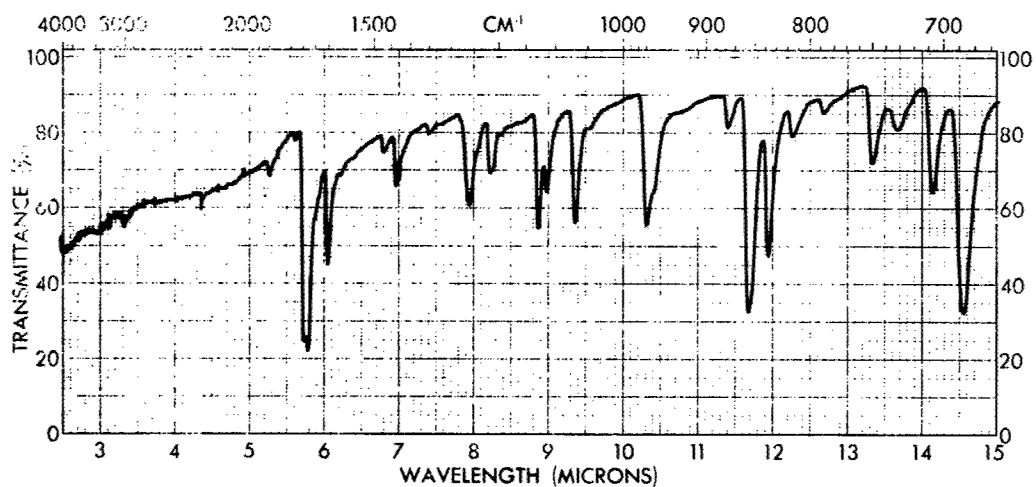
Figure 77 - Infrared Spectrum of 5,6-Dibromo-1,2-diketopyracene (KBr)
