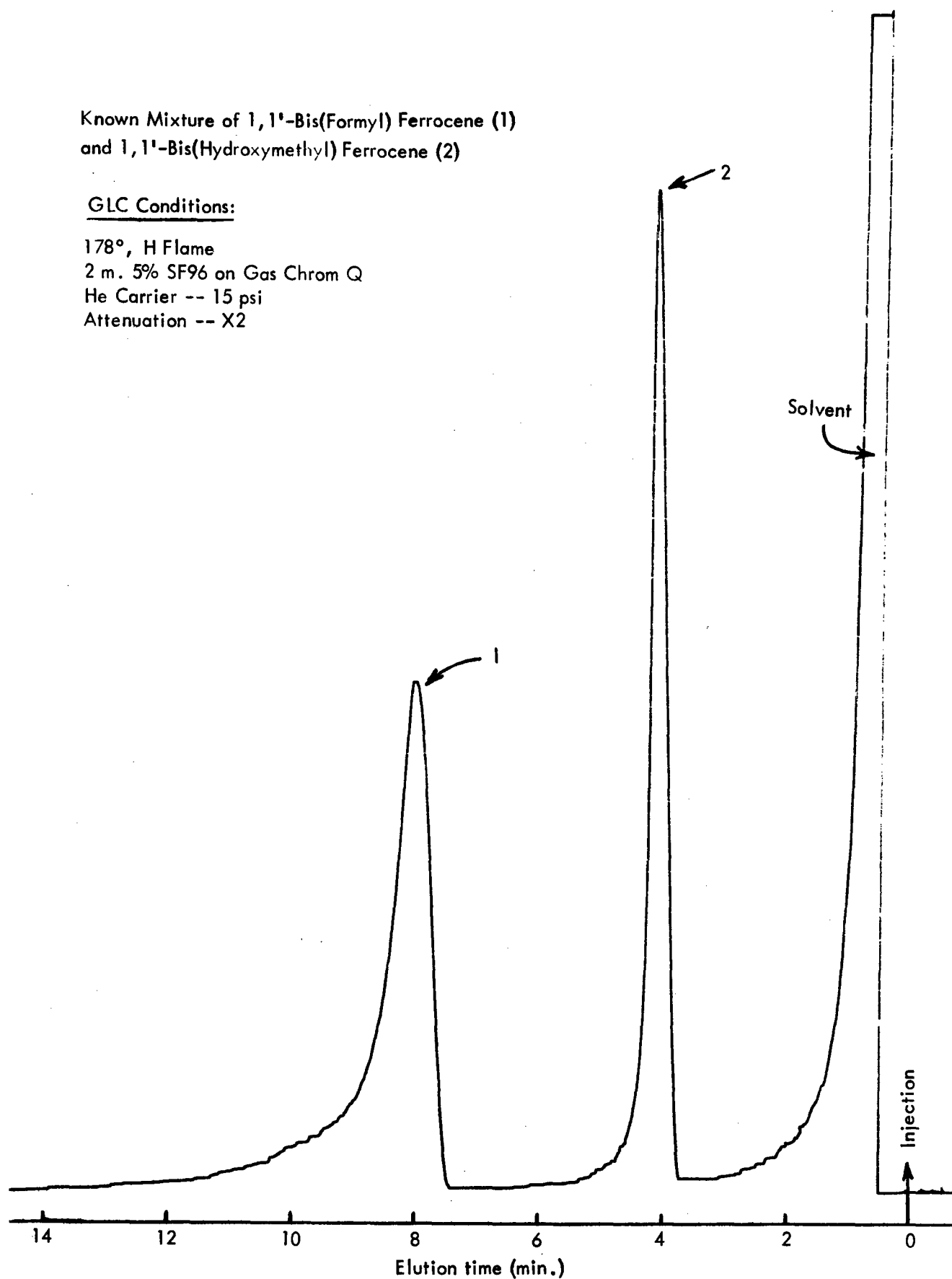
Figure 26 - Gas Liquid Chromatogram of a Mixture of 1,1'-Bis(hydroxymethyl)-ferrocene and 1,1'-Bis(formyl)ferrocene
