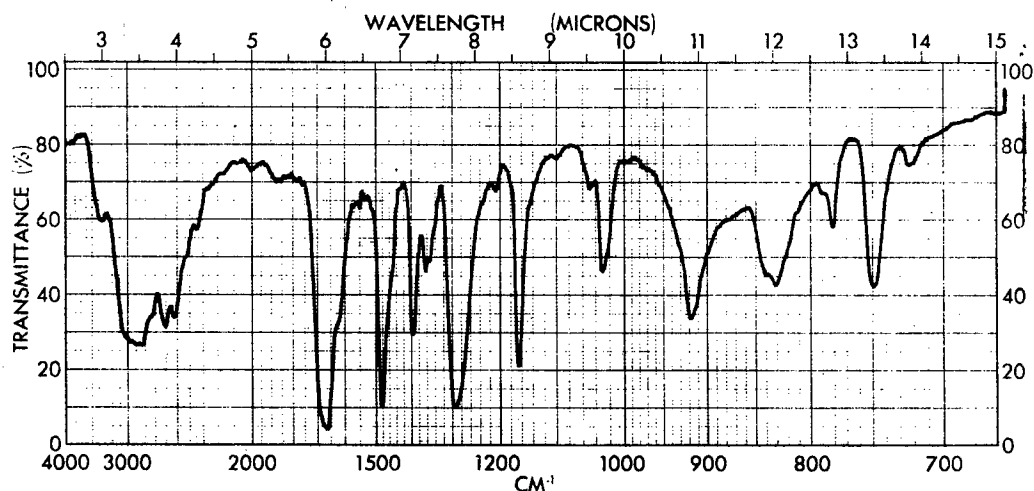
Figure 24 - Infrared Spectrum of 1,1'-Bis(carboxy)ferrocene (KBr)
