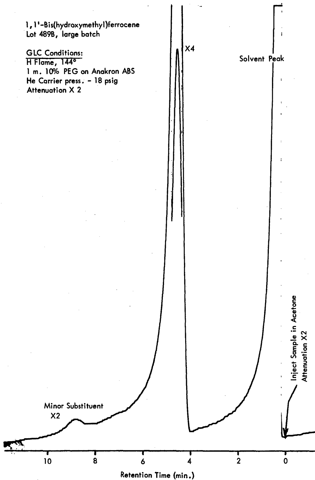
Figure 34 - Gas Liquid Chromatogram of 1,1'-Bis(hydroxymethyl)ferrocene (Lot 489B)
