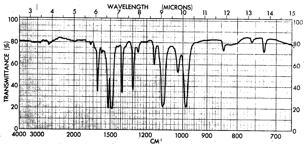
Figure 11 - Infrared Spectrum of Pentafluorophenylphosphonous Dibromide (Liquid)
