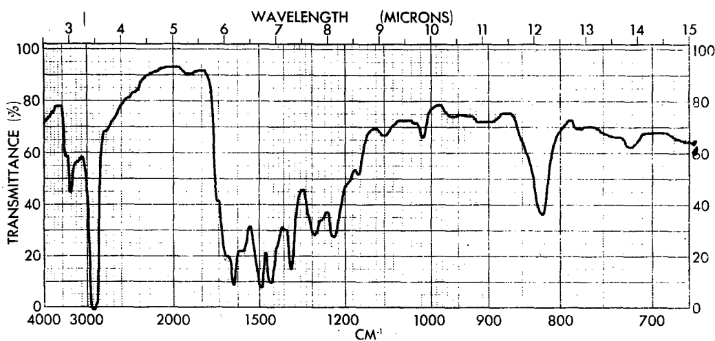
Figure 5 - Infrared Spectrum of the Substance Precipitated from Dimethylacetamide in the "Bisdione" Preparation (Nujol)
