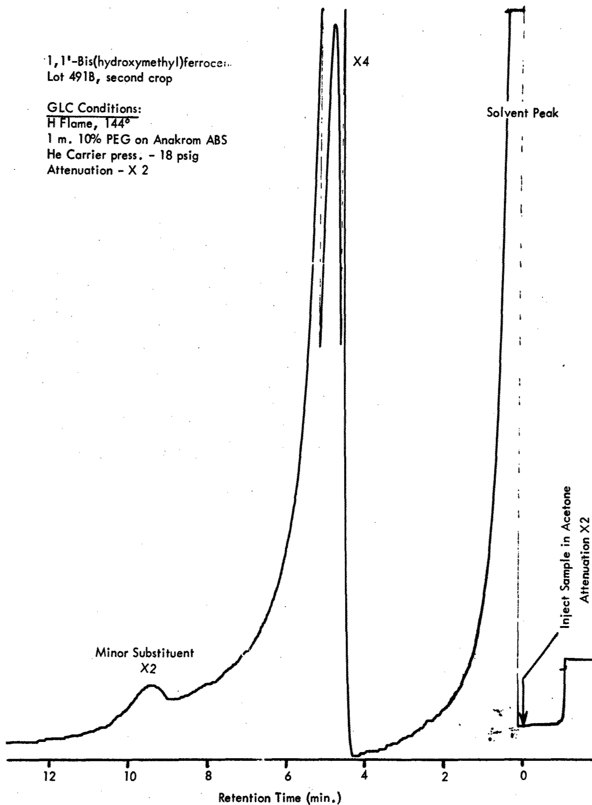
Figure 37 - Gas Liquid Chromatogram of 1,1'-Bis(hydroxymethyl)ferrocene (Lot 491B, Second Crop)
