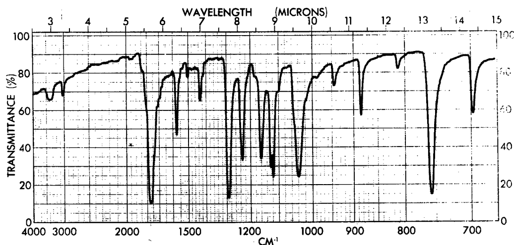
Figure 58 - Infrared Spectrum of NTCA Dianhydride (Produced by Heating NTCA No. 5 on DTA to 350°) (KBr)
