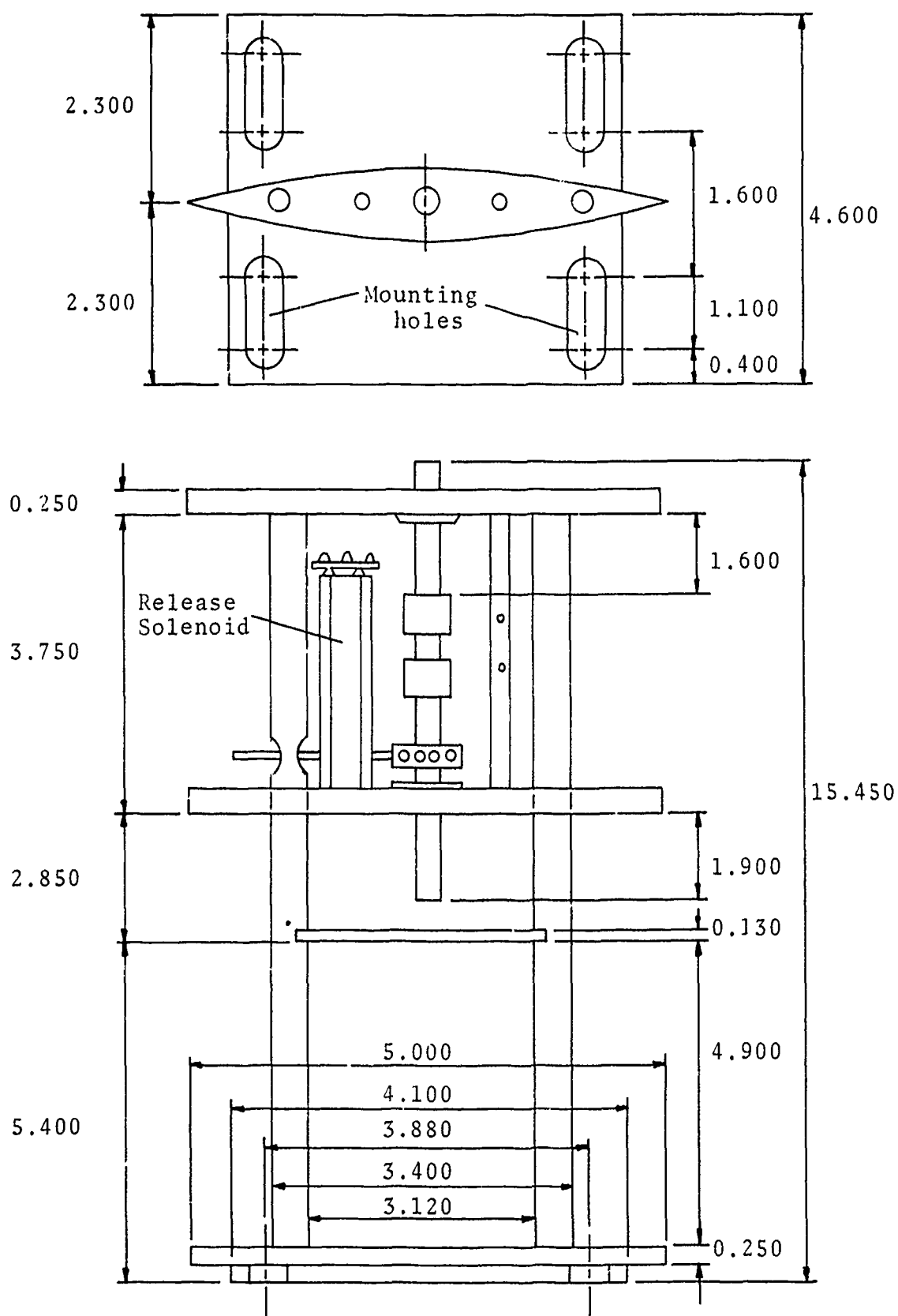
Figure II-13. Accelerometer Stand
