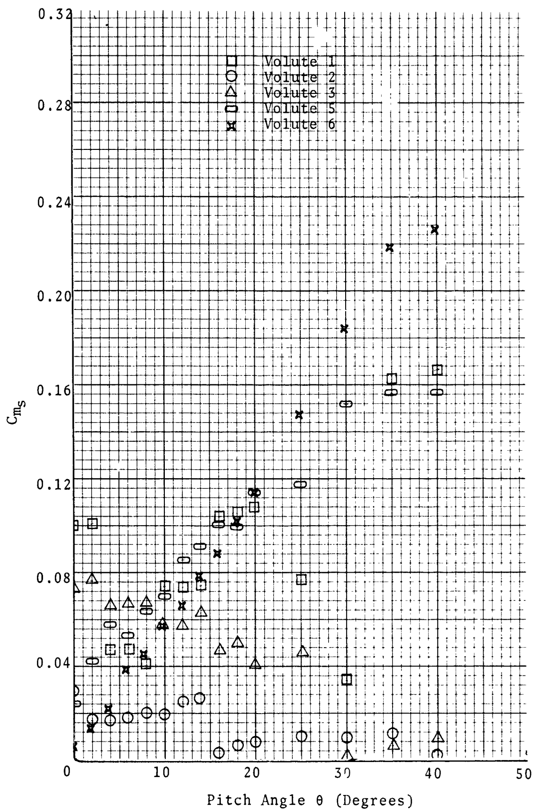
Figure II-7. \theta Versus C_{m_s} For Rigid Volutes
