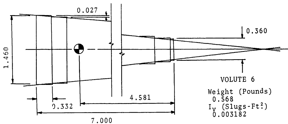
Figure II-2. Rigid Volute : 4, 5, and 6
