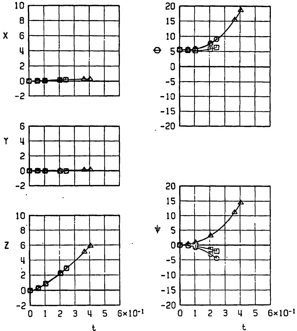
a. Configurations 8 through 10 Fig. 27 Effect of Aircraft-Loading Configuration on the Separation Trajectories of the Unfinned BLU-1C/B at Mach Number 0.42
