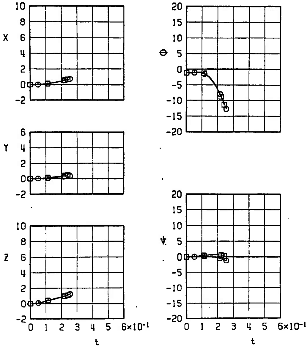
a. Configurations 32 and 40 Fig. 37 Effect on Wing-Loading Configuration on Separation Trajectories of the MK-82GP at Mach Number 0.95
