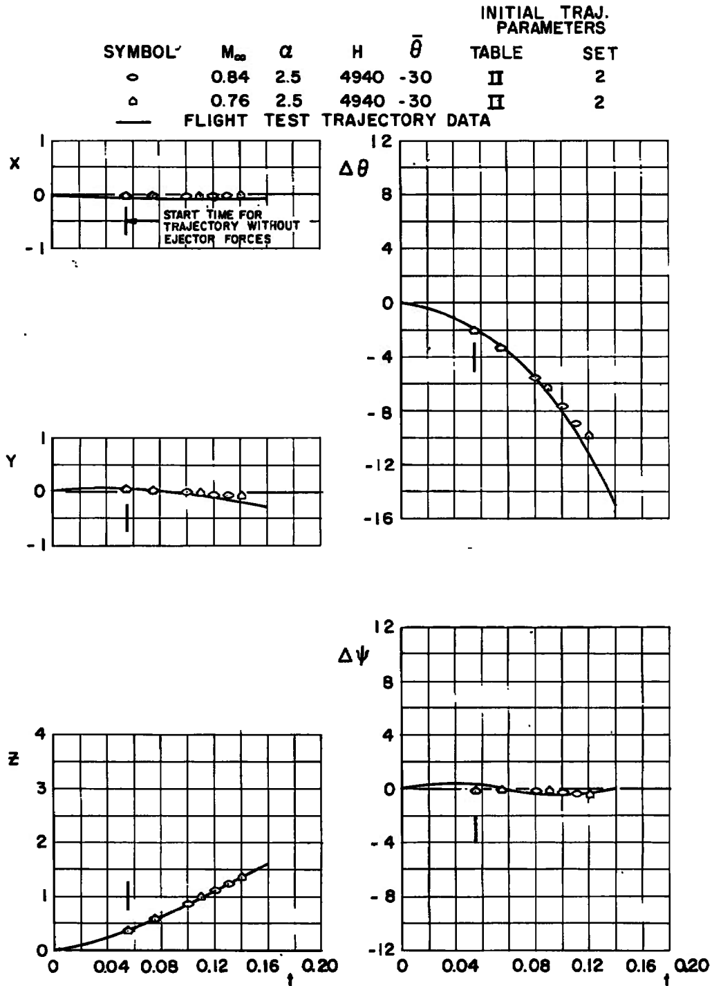
Fig. 24 Effect of Mach Number Variation on the Unfinned BLU-1C/B Trajectories; Configuration 5
