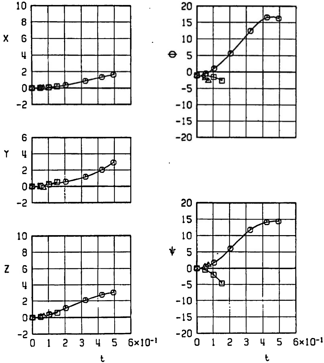
Fig. 39 Effect of Wing-Loading Configuration on Separation Trajectories of the MK-82SE at Mach Number 0.86
