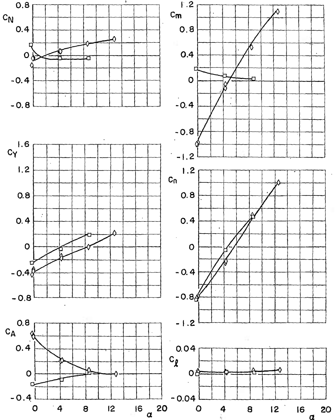
Fig. 17 Aerodynamic Coefficients of the Unfinned BLU-1C/B with Parent Angle of Attack at Mach Number 0.90
