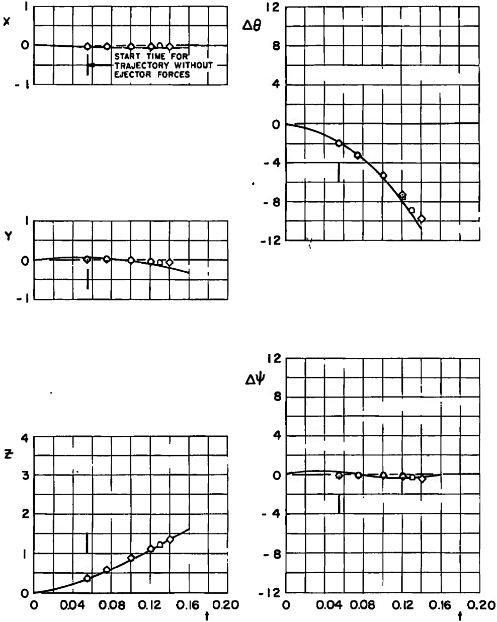
Fig. 22 Effect of Damping Derivative Variation on the Unfinned BLU-1C/B Trajectories; Configuration 5
