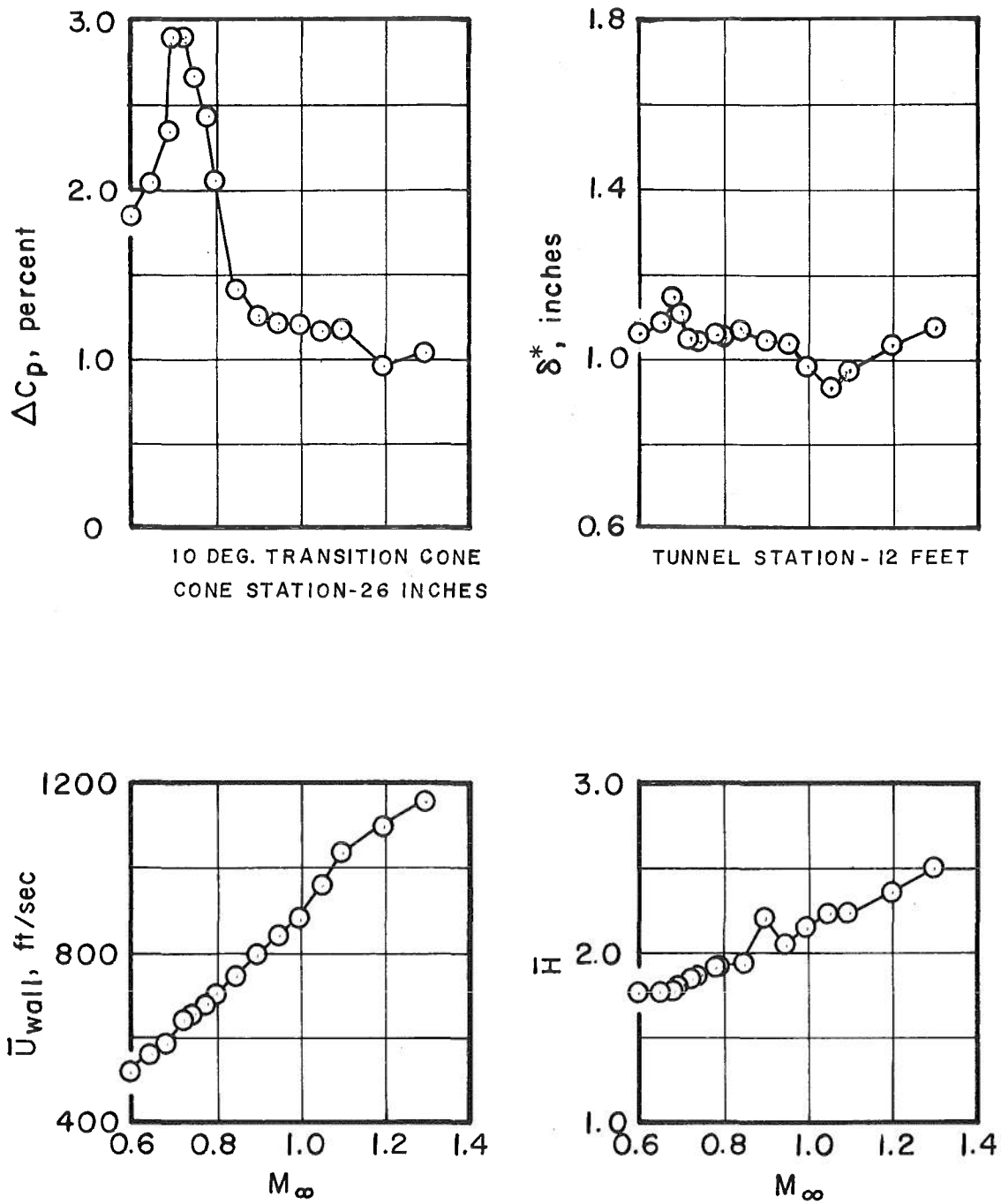
Fig. 12 Variation of Tunnel 16T Wall Boundary-Layer Characteristics and Test Section Noise Levels as a Function of Mach Number, p_t = 1185 psfa, \theta_w = 0 deg
