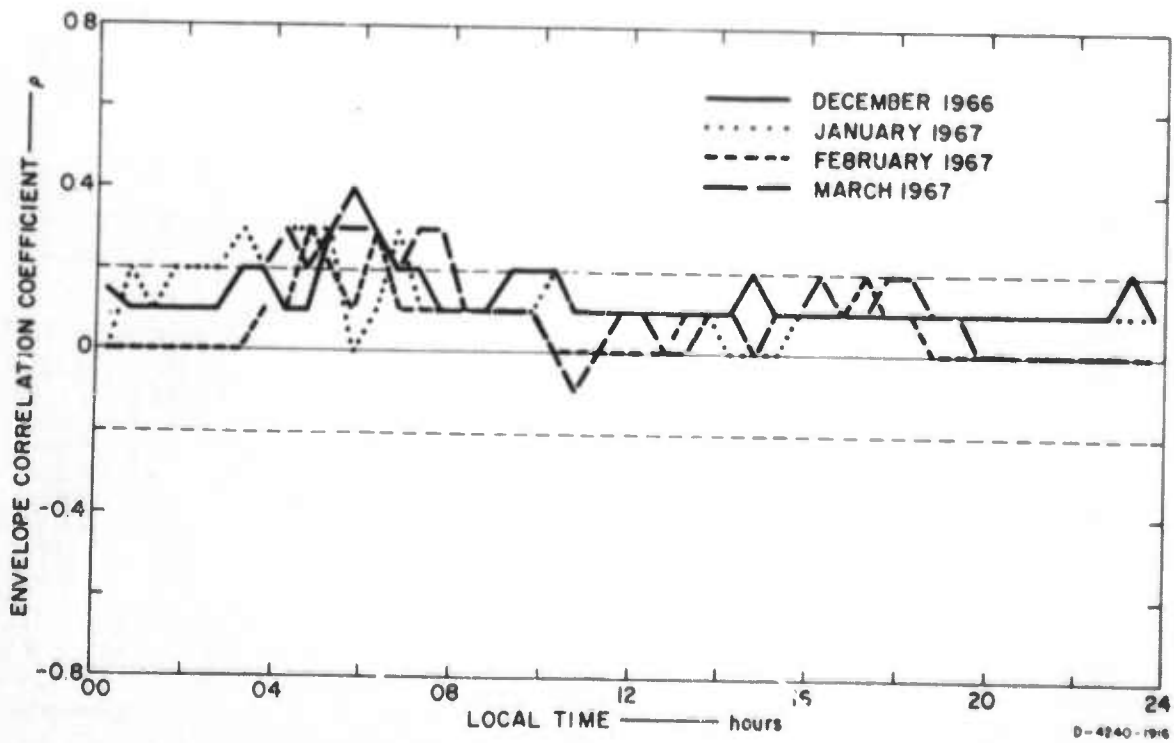
FIGURE IV-14 ENVELOPE CORRELATION COEFFICIENT OF SIGNALS RECEIVED AT CHIENGMAI
