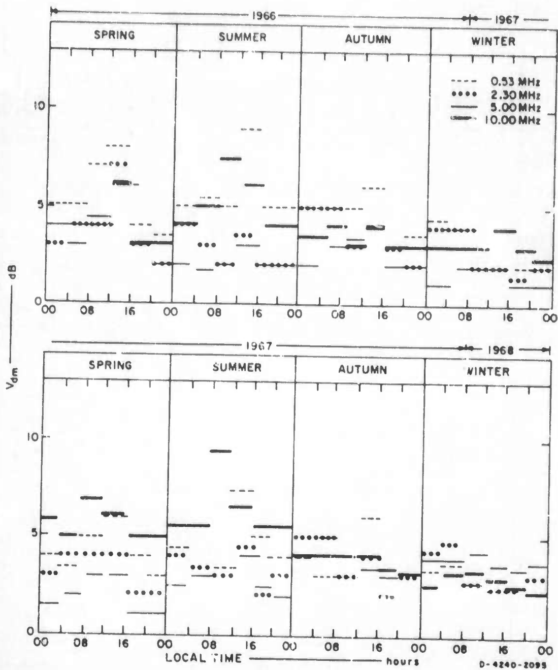
FIGURE IV-33 QUARTERLY TIME BLOCK MEDIAN OF NOISE VOLTAGE DEVIATION ( V_{dm} ) OBSERVED AT LAEM CHABANG DURING THE PERIOD MARCH 1966 THROUGH FEBRUARY 1968
