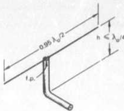
(b) DIPOLE—ALUMINUM INSTALLED AT FEEDPOINT (f.p.) FOR BALANCED DIPOLES
