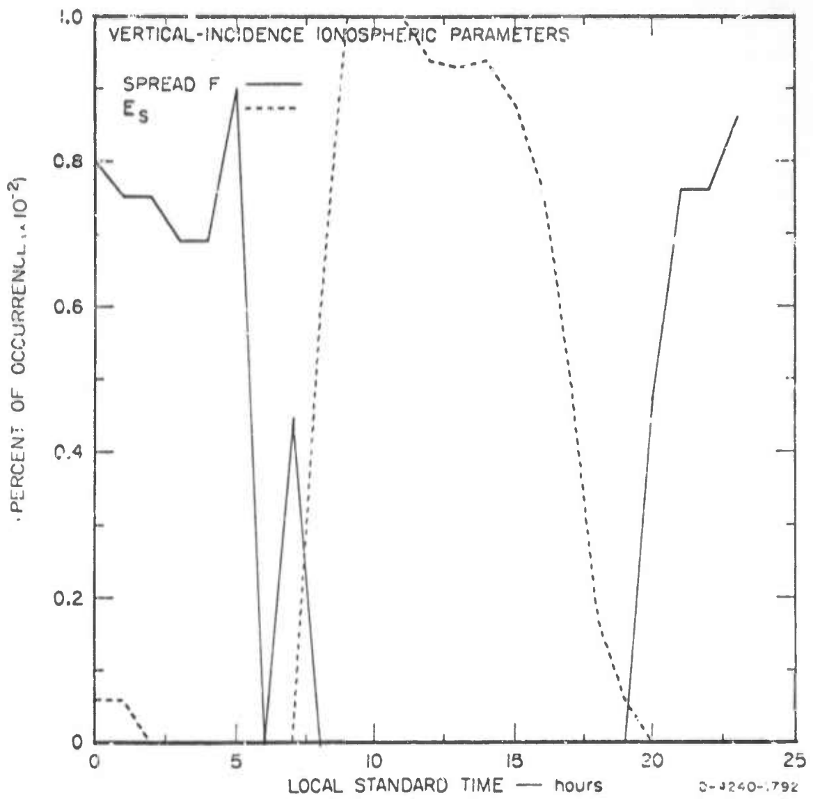
FIGURE IV-31 PERCENT OCCURRENCE OF SPREAD F AND SPORADIC E AT SONGKHLA, FEBRUARY 1967
