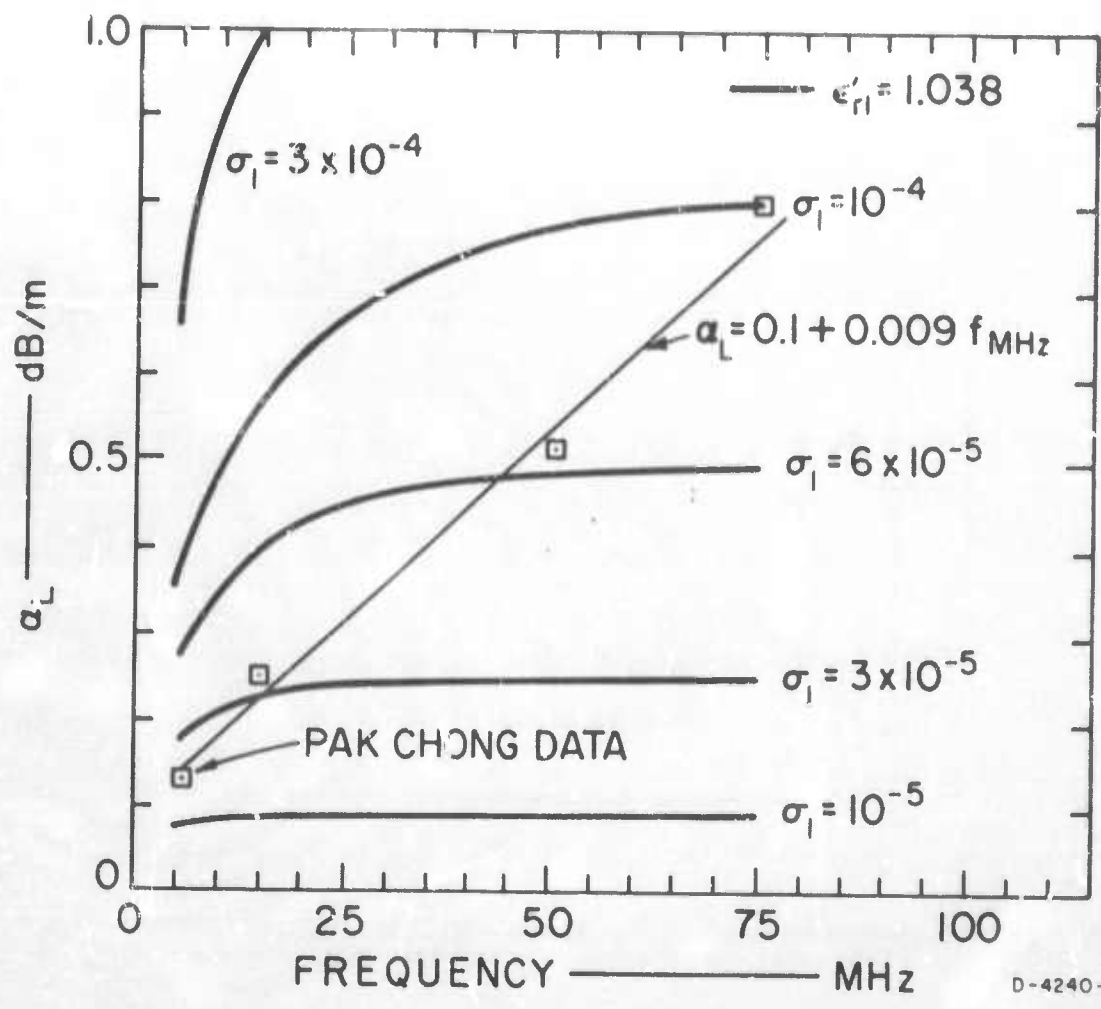
FIGURE III-11 LATERAL WAVE ATTENUATION CONSTANT COMPUTED AS A FUNCTION OF FREQUENCY, WITH CONSTANT CONDUCTIVITY
