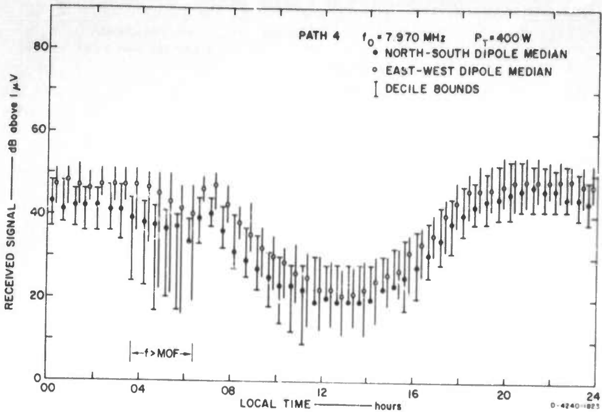
FIGURE IV-13 CW RECEIVED SIGNAL STRENGTH AT CHIENGMAI
