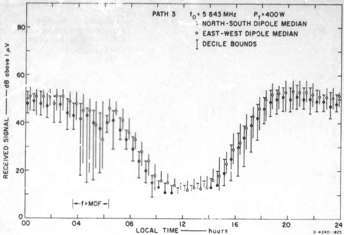
FIGURE IV-11 CW RECEIVED SIGNAL STRENGTH AT NAKON SAWAN
