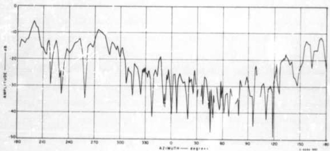
FIGURE III-27 MEASURED AMPLITUDE VERSUS AZIMUTH ANGLE OF 50-MHz VHF ANTENNAS IN A EUCALYPTUS GROVE—8° ELEVATION
