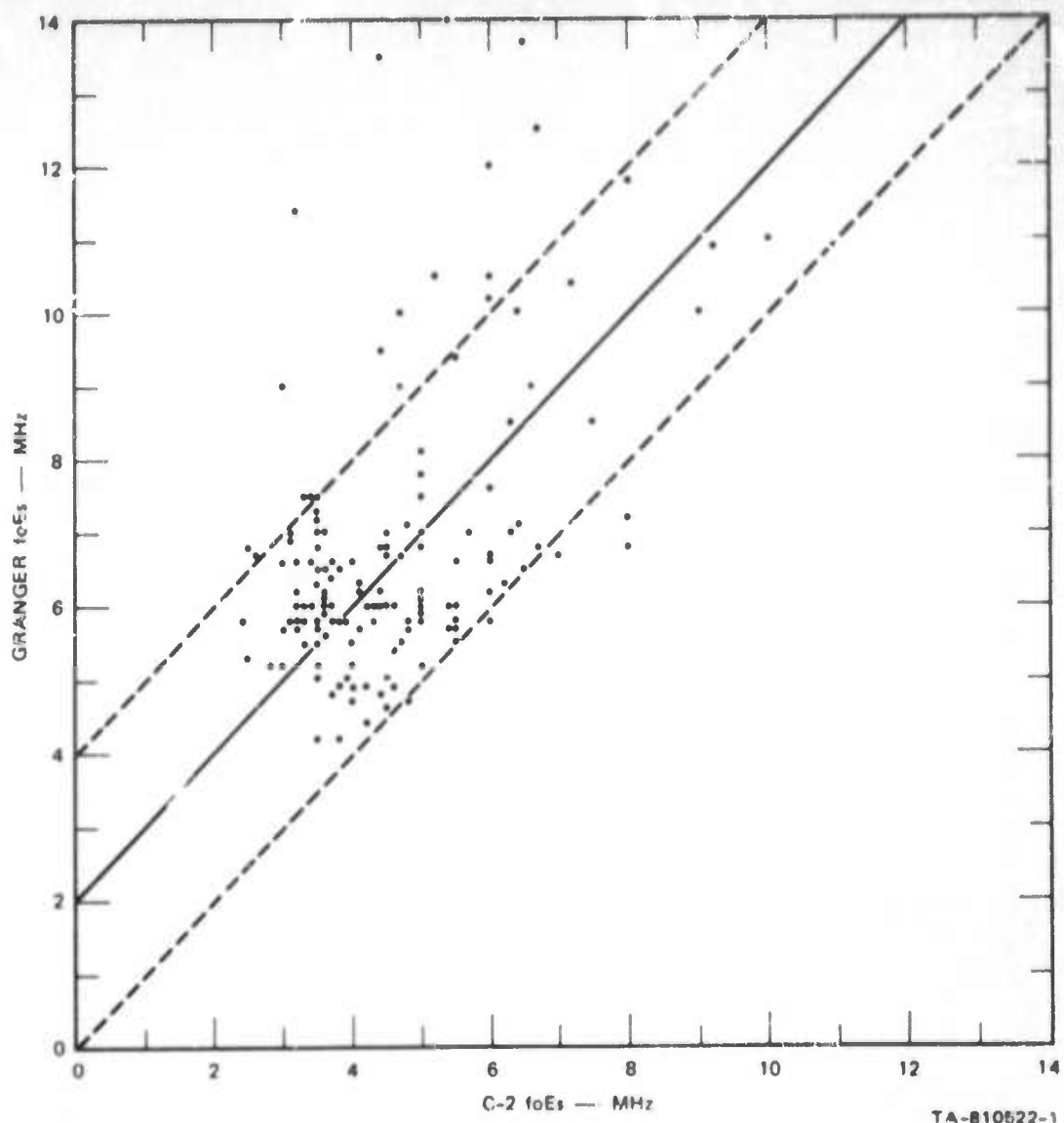
FIGURE IV-30 MASS PLOT OF f_oE_1 , AS A FUNCTION OF FREQUENCY OF THE C-2 AND GRANGER SOUNDERS AT BANGKOK
