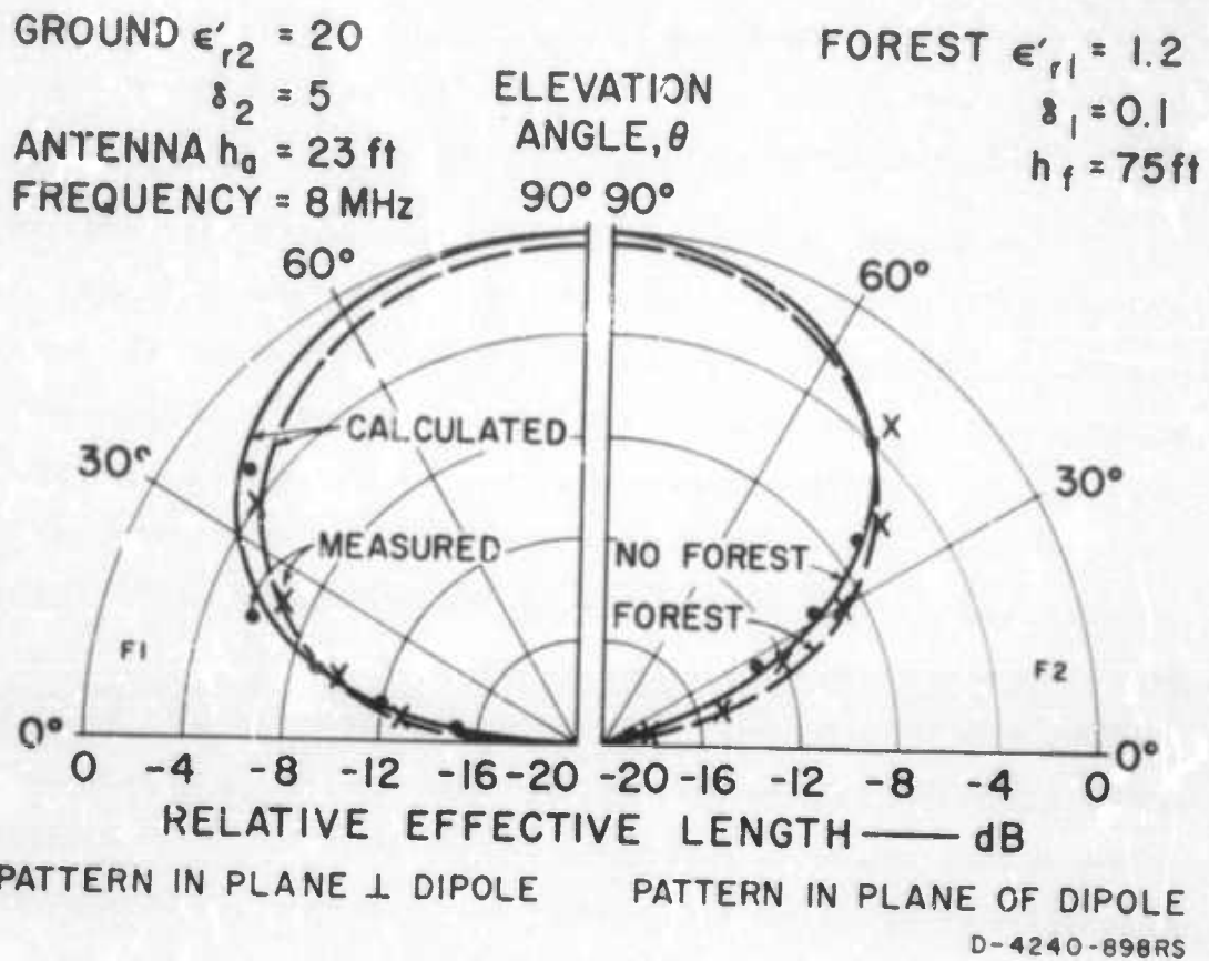
FIGURE III-29 COMPARISON OF MEASURED AND CALCULATED EFFECTIVE LENGTHS FOR DIPOLE IN FOREST AND IN OPEN
