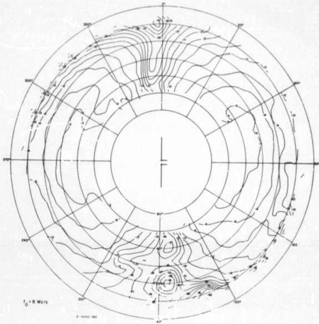
FIGURE III-19 MEASURED RADIATION PATTERN OF THE 8 MHz, 23-FOOT HIGH UNBALANCED DIPOLE AT ALMANOR— E_\phi AT 8 MHz
