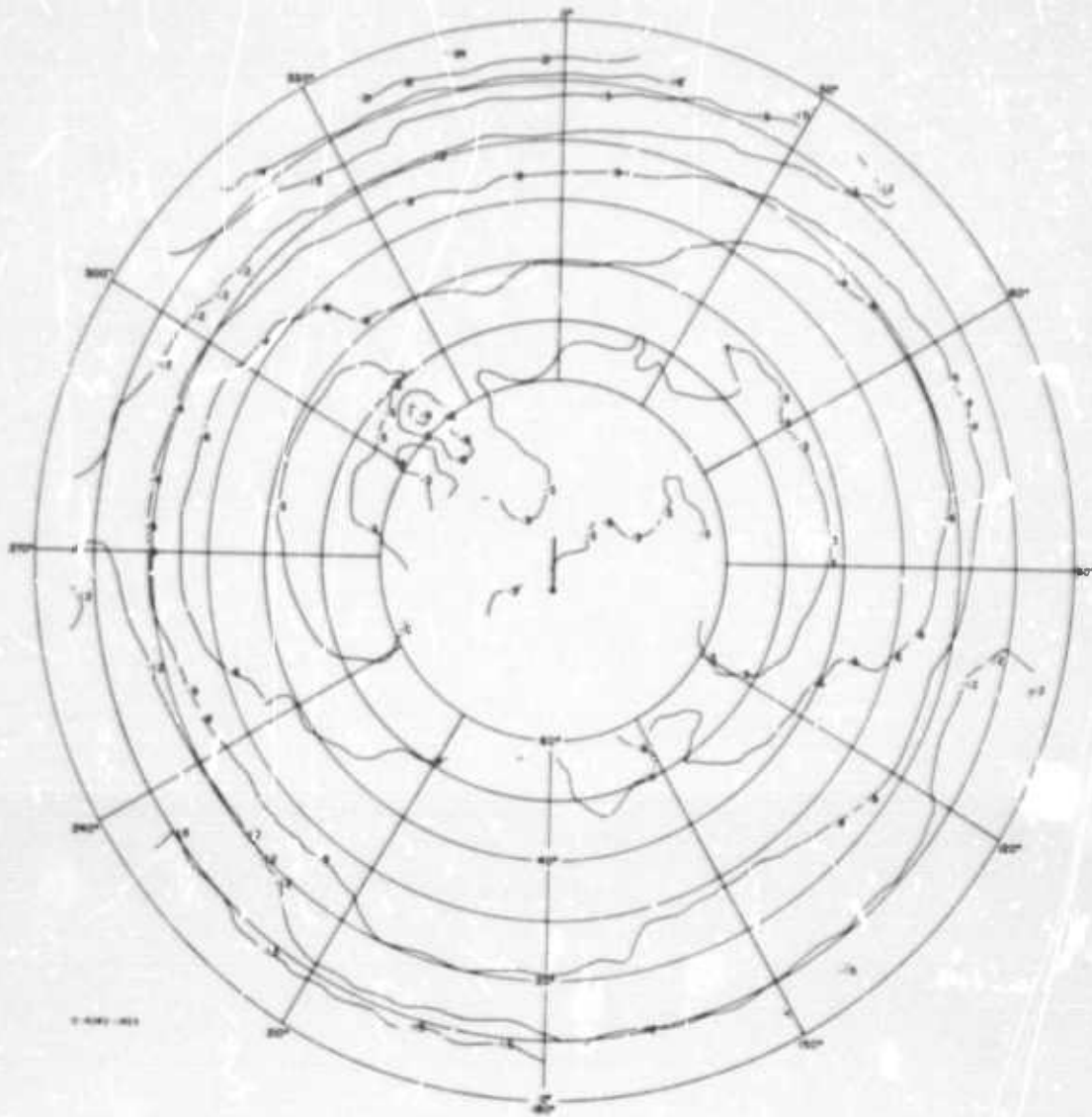
FIGURE III-25 MEASURED RADIATION PATTERN OF THE 6 MHz 5:1 INVERTED L ANTENNA AT BAN MUN CHIT—POWER AT 6 MHz
