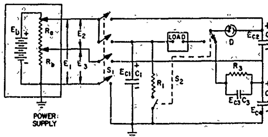
Figure 7-16. Single-diode Ruhlmann Circuit
