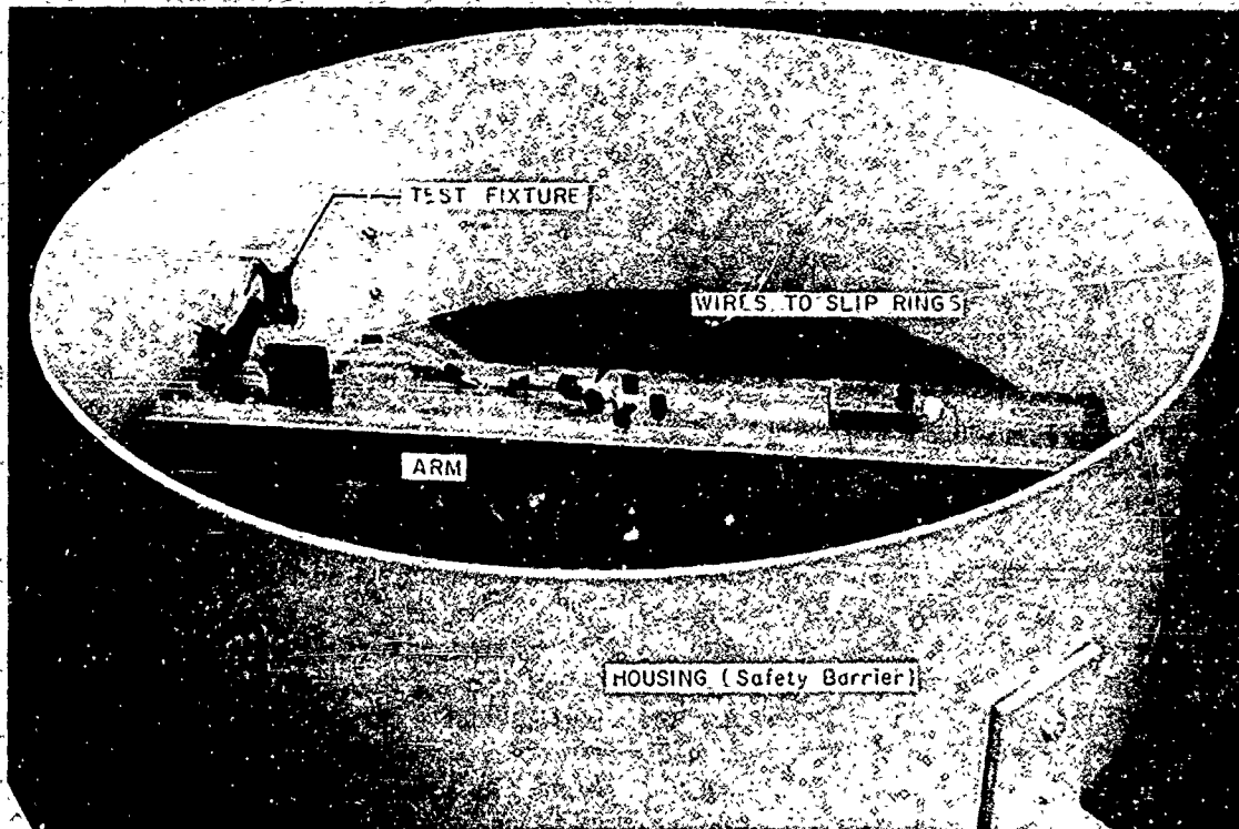
Figure 15-2. Low-g Centrifuge
