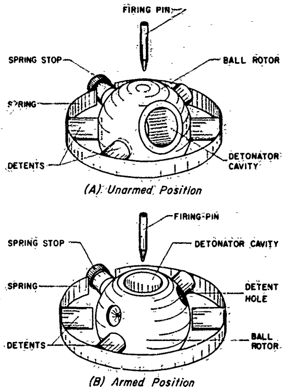
Figure 6-22. Ball Rotor
