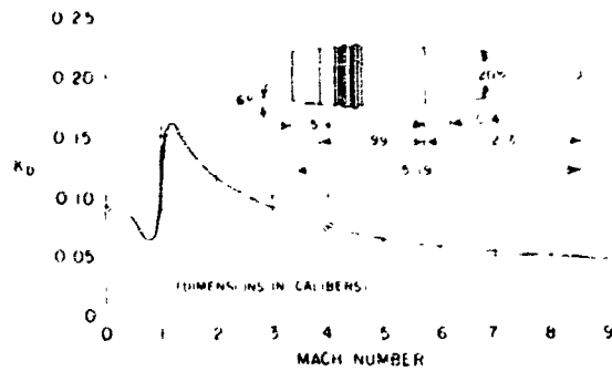
Figure 5-4. Drag Coefficient K_D
