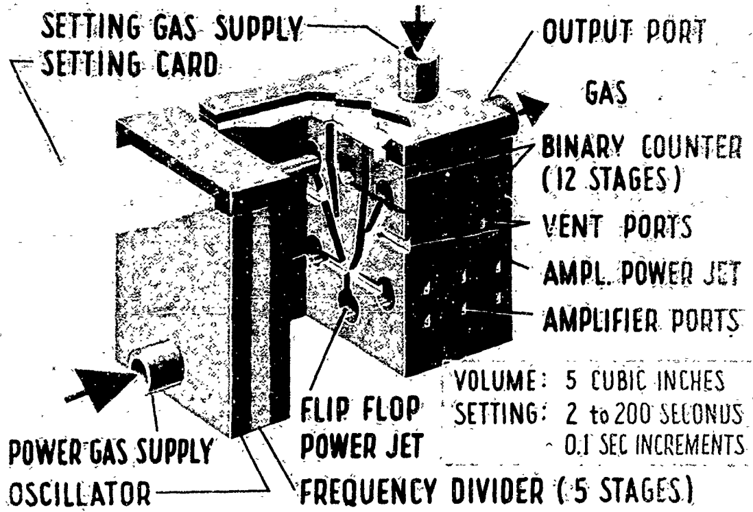
Figure 8-4. Fluoric Timer
