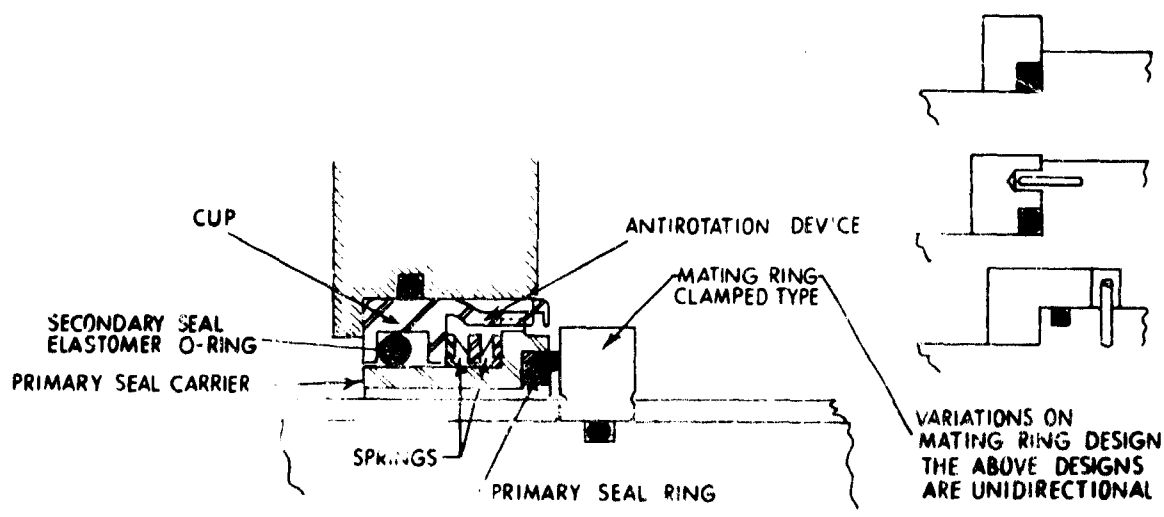
Figure 13 - Cup- or Package-Type Mechanical Face Seal, Stationary Mounted
