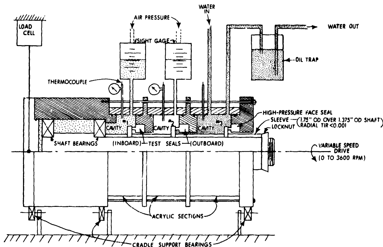
Figure 19 Seal Test Fixture
