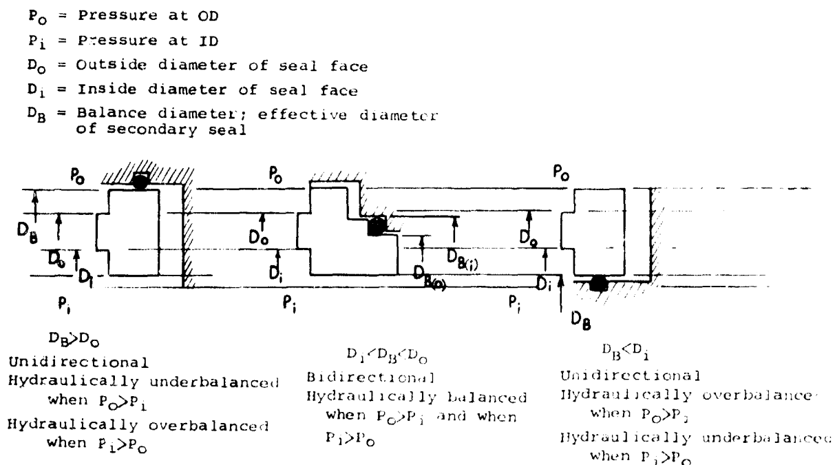
Figure 14 - Directional Sealing Ability of Face Seal
