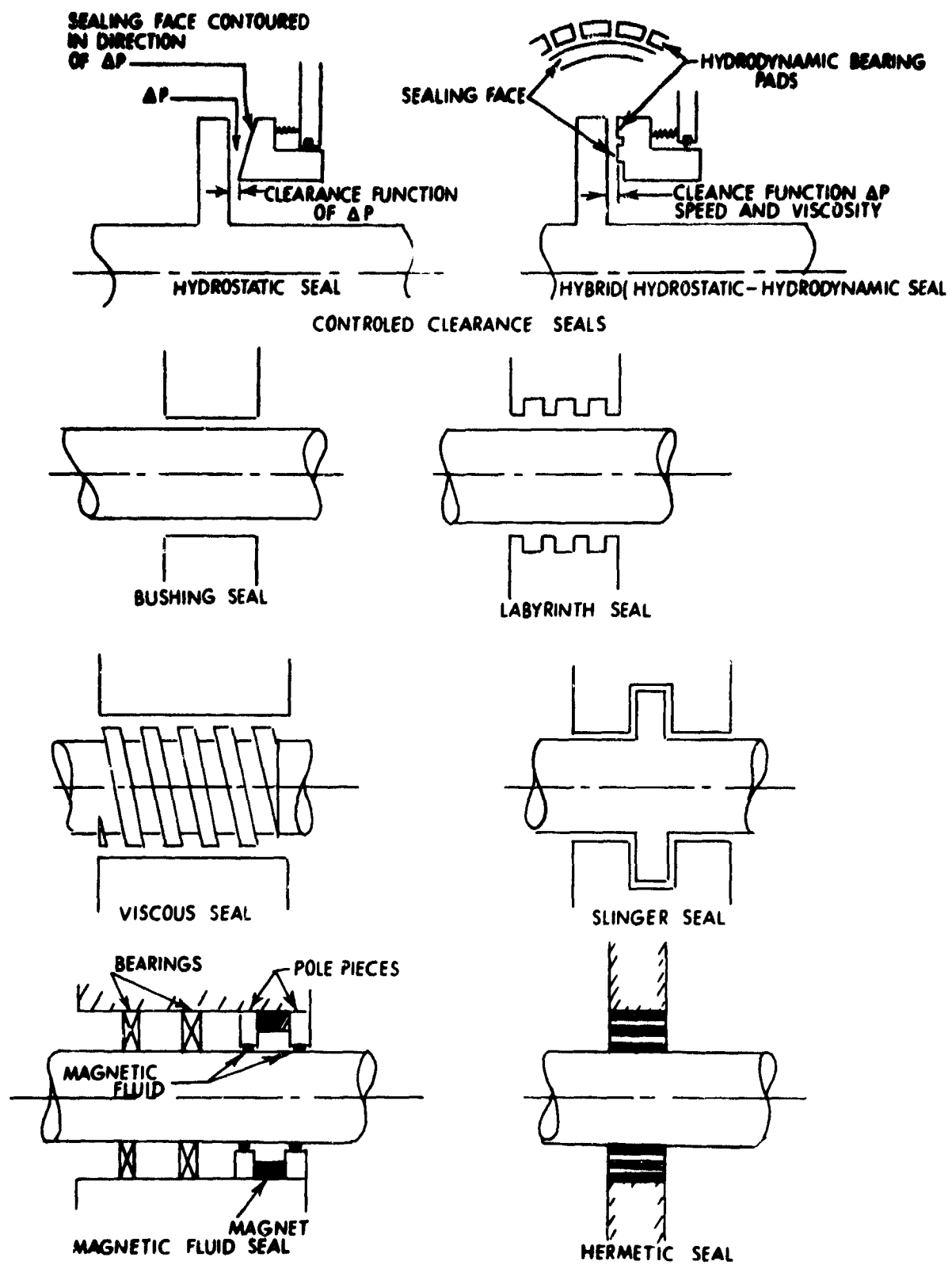
Figure 7 - Various Seal Configurations
