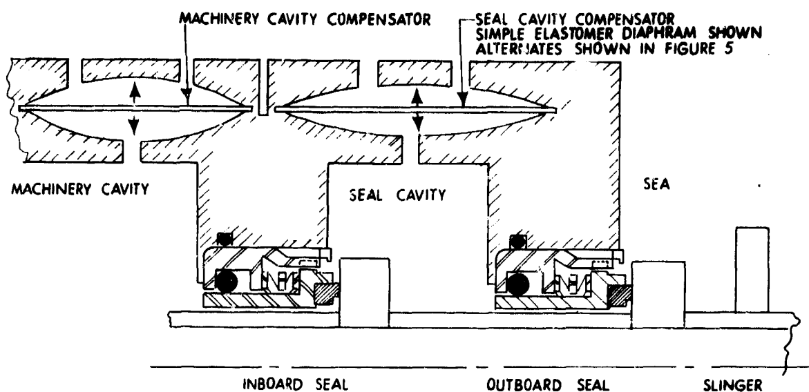
Figure 1 - Double Seal, Redundant Arrangement ( \Delta P Nominally Zero)
