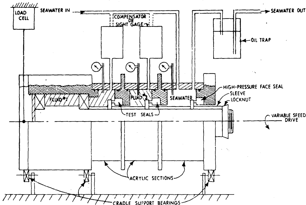
Figure 19 - Seal Test Fixture
