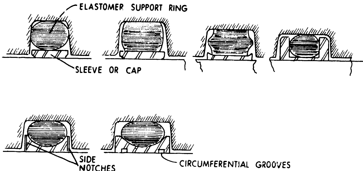
Figure 17 - Examples of Slipper or Cap Seals
