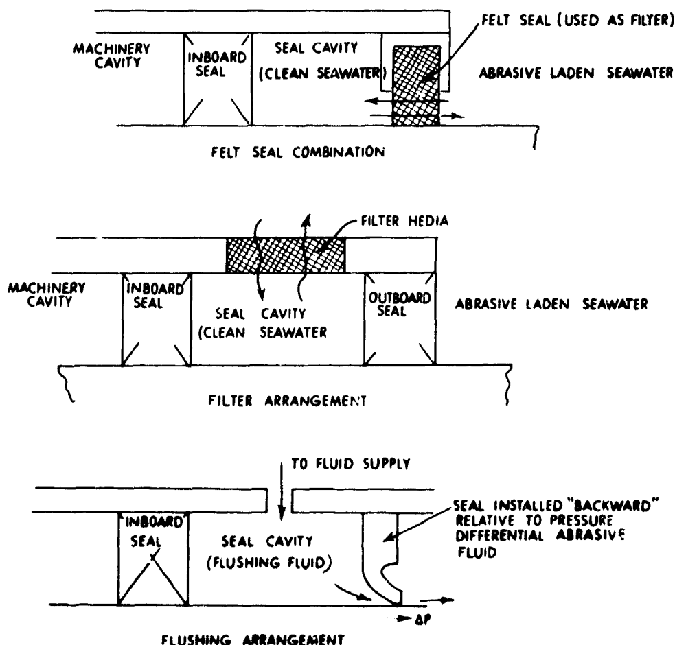
Figure 11 - Possible Arrangements for Abrasive Protection
