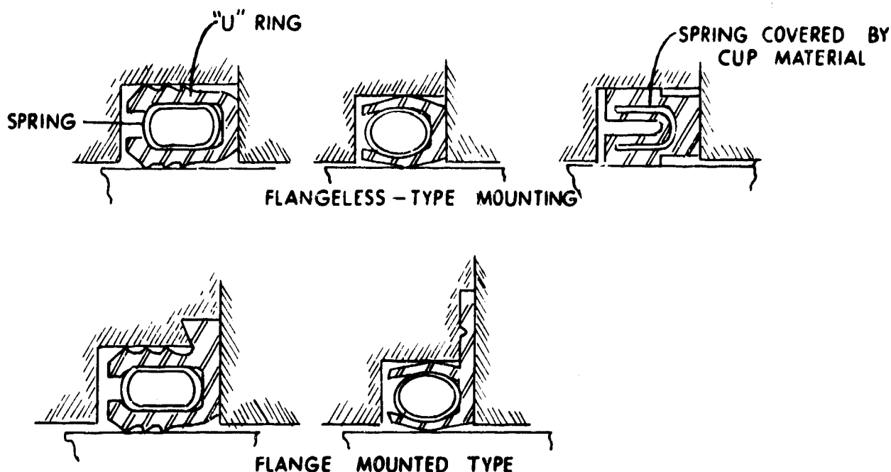
Figure 18 - Examples of U-Cup Seals
