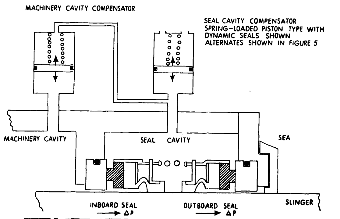
Figure 2 - Double Seal, Pressure Cascaded Arrangement ( \Delta P Nominally 2 to 5 PSID)
