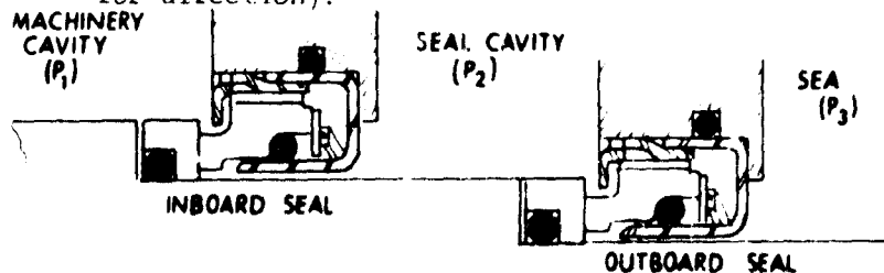
Figure 15 - Examples of Double Face Seal Arrangements in Use
