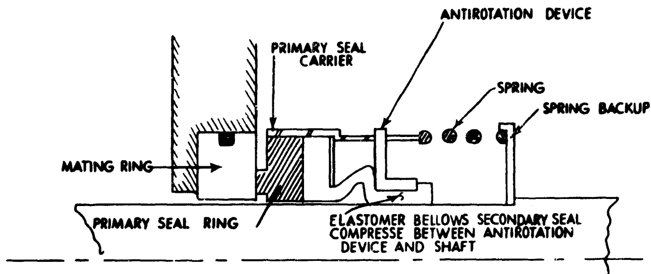
Figure 12 - Shaft-Mounted Face Seal with Elastomer Bellows Secondary Seal
