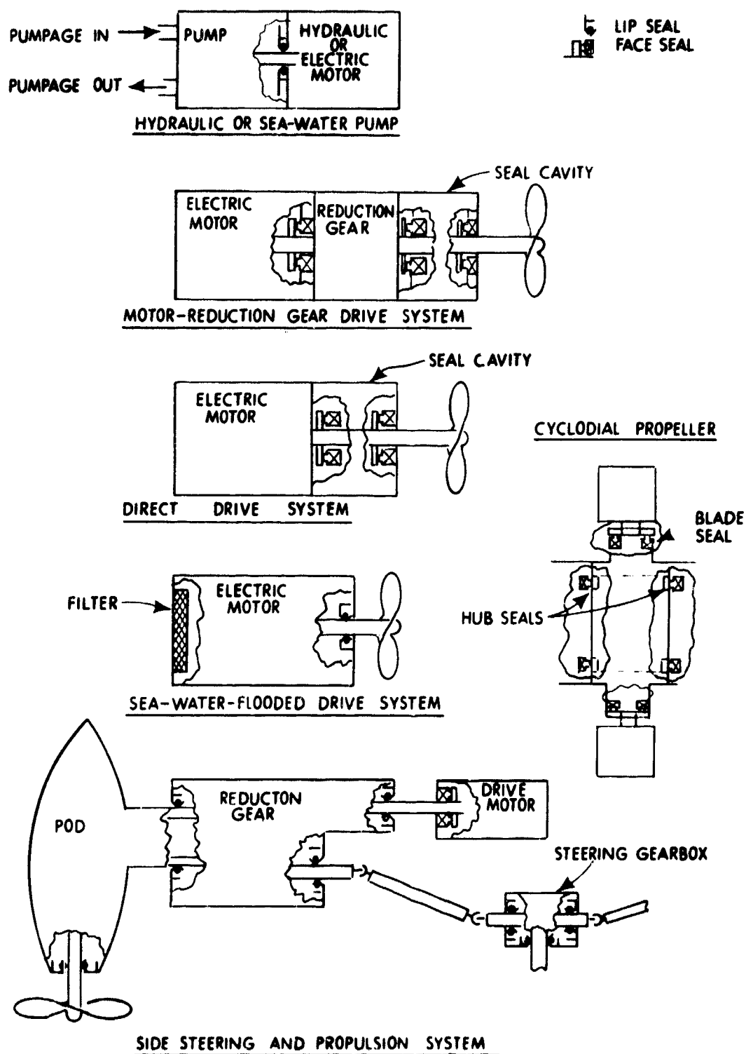
Figure 4 - Typical Deep-Ocean Dynamic Seal Applications
