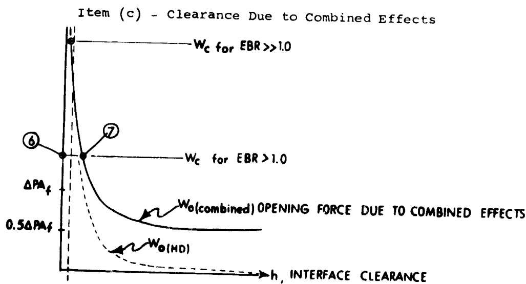
Figure 9 - Forces on Sealing Element as a Function of the Interface Clearance
