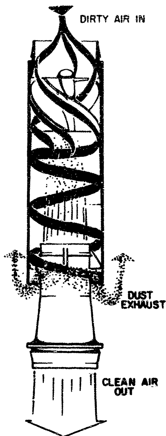
Figure 11-5. Straight-flow Dust Separator Tube Cyclone Principle
