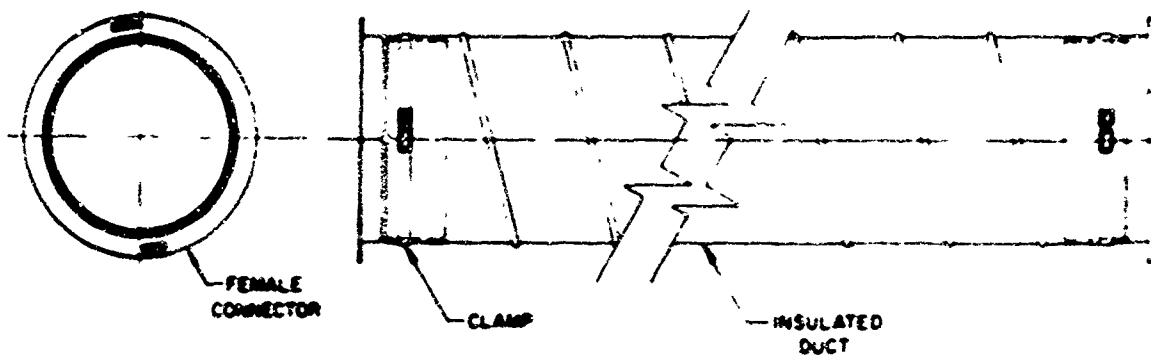
Figure 9-38. Drawing Showing Method of Attaching Flexible Duct to Female Connector With Metal Ring Clamp (Courtesy of Trane Company)
