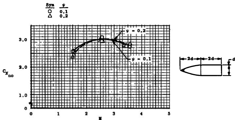
a. 2-cal Nose Length
