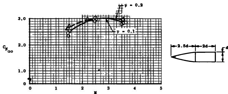
b. 2.5-cal Nose Length
