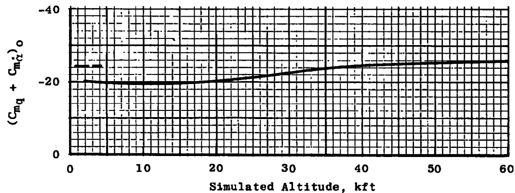
Fig. 39 Damping-in-Pitch Derivatives at M = 2 for Secant-Ogive-Cylinder Configurations with Boattail (Zero Yaw Angle)
