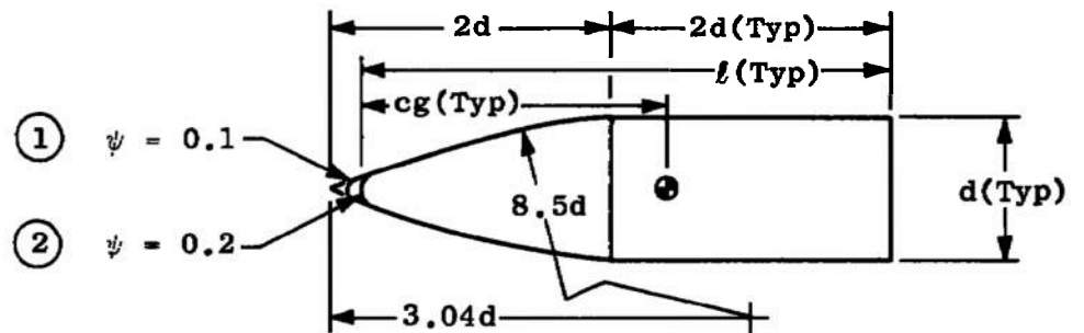
a. 2.0-cal Secant-Ogive Nose
