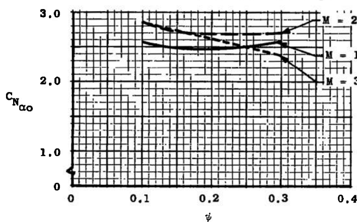
Fig. 24 Effect of Nose Bluntness on C_{N_{\alpha 0}} for Secant-Ogive-Cylinder Configurations at Ground Level
