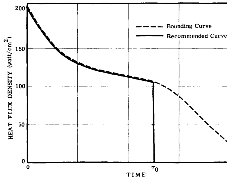
Figure 2-38 Bounding and Recommended Heat Flux Density Curves for the LO 2 /LH 2 Propellant Combination
