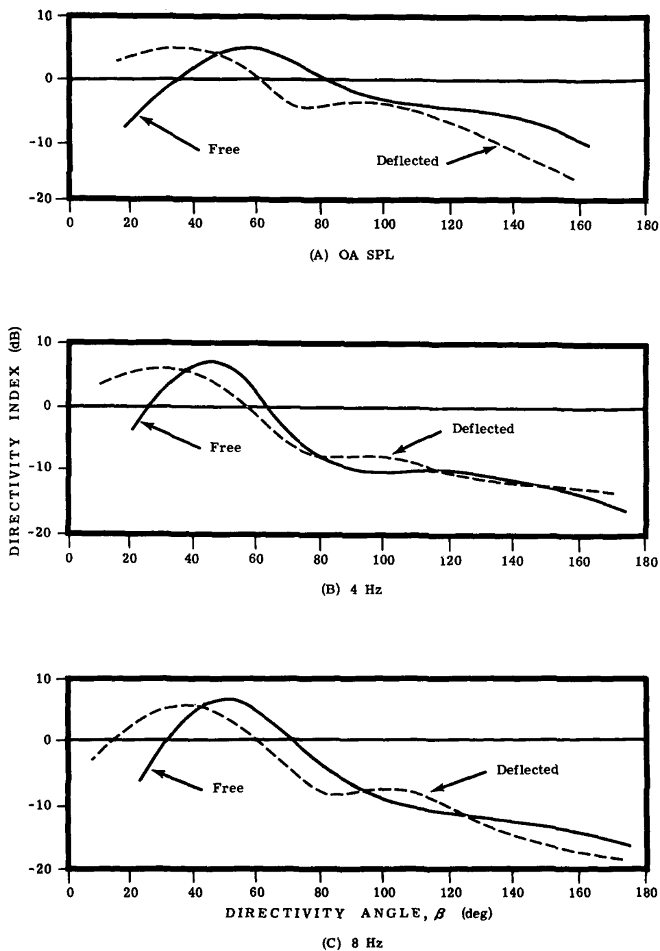
Figure 7-13 Typical Directivity Indices for Deflected and Free Field Condition (Measured from the centerline of the deflected exhaust)
