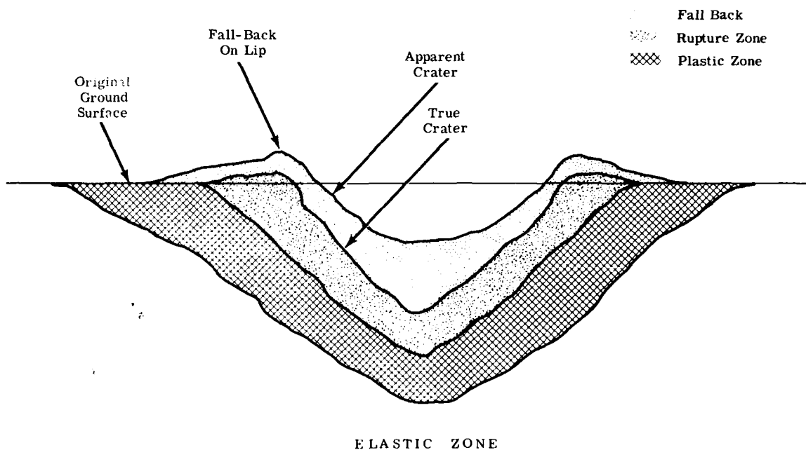
Figure 2-39 Typical Crater Profile
