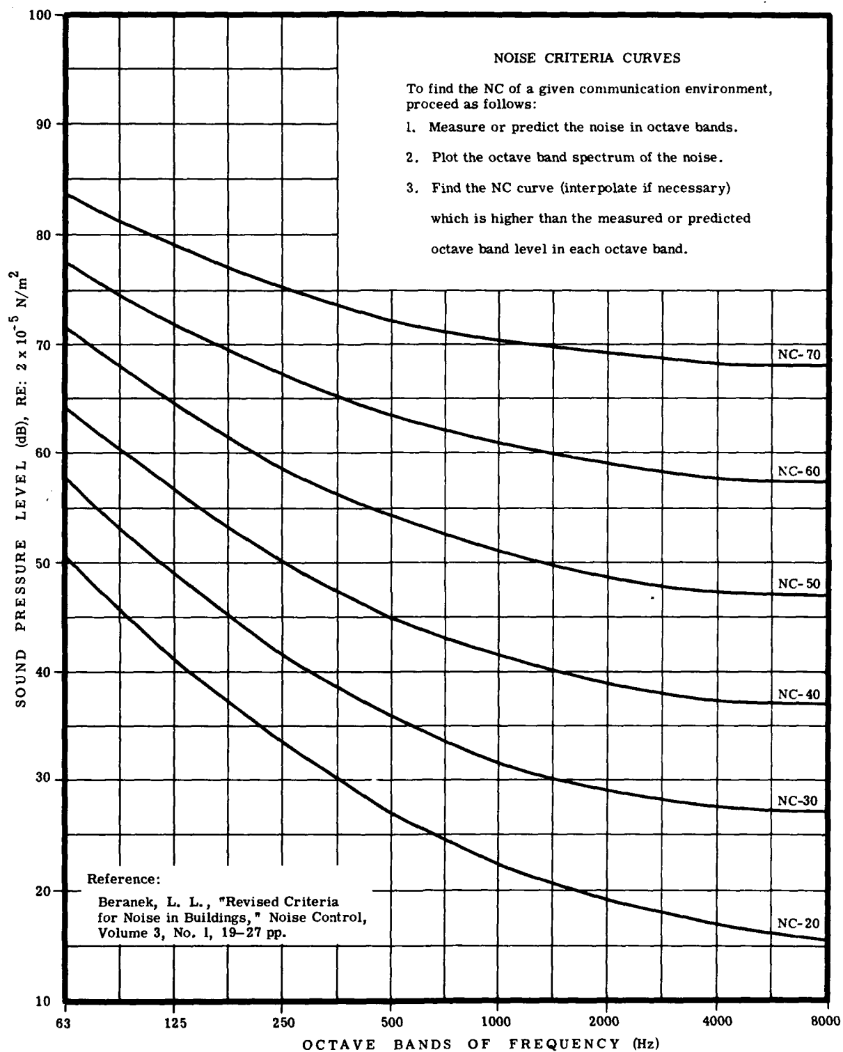
Figure 7-28 Noise Criteria Curves
