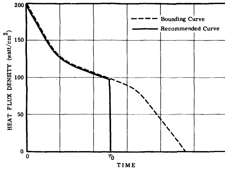
Figure 2-37 Bounding and Recommended Heat Flux Density Curves for the LO 2 /RP-1 Propellant Combination
