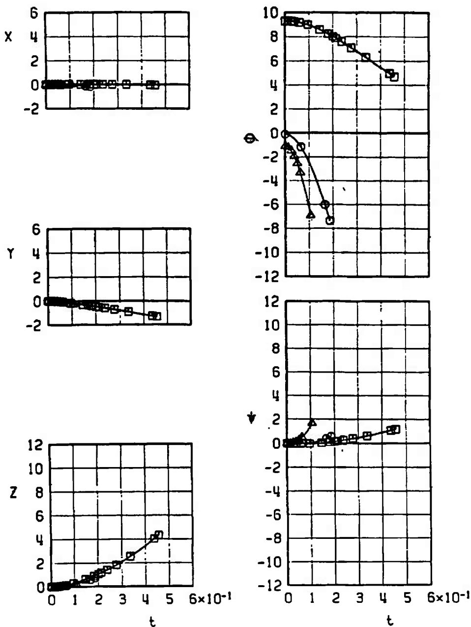
Fig. 14 Effect of Mach Number and Climb Angle on the Separation Trajectories of the M-117R from Center Pylon Station, Inboard and Outboard Pylon Empty
