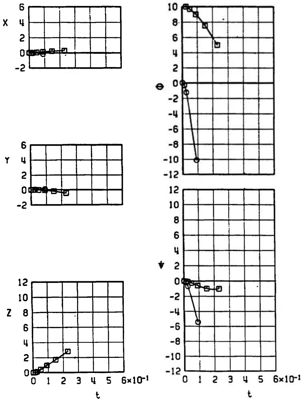
Fig. 20 Effect of Mach Number on the Separation Trajectories of the SUU-42/A from the Outboard Pylon, MER with M-117R on Center Pylon, and an M-117R on Inboard Pylon, Configuration 28L
