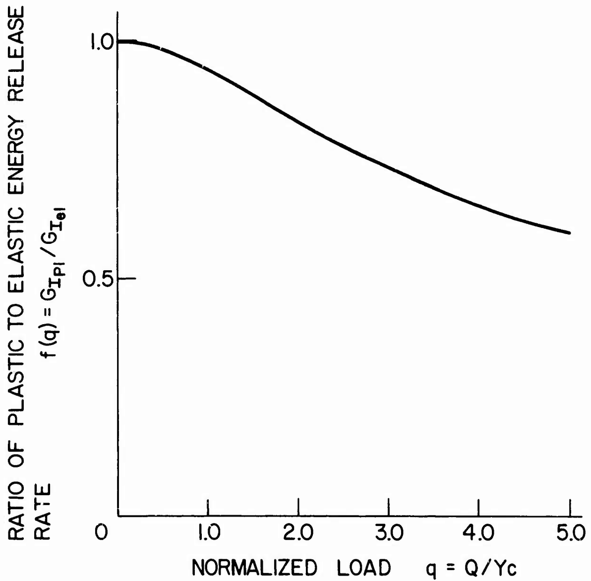
Figure 16. Ratio of Plastic to Elastic Energy Release Rate as a Function of Normalized Load for Semi-Infinite Crack.
