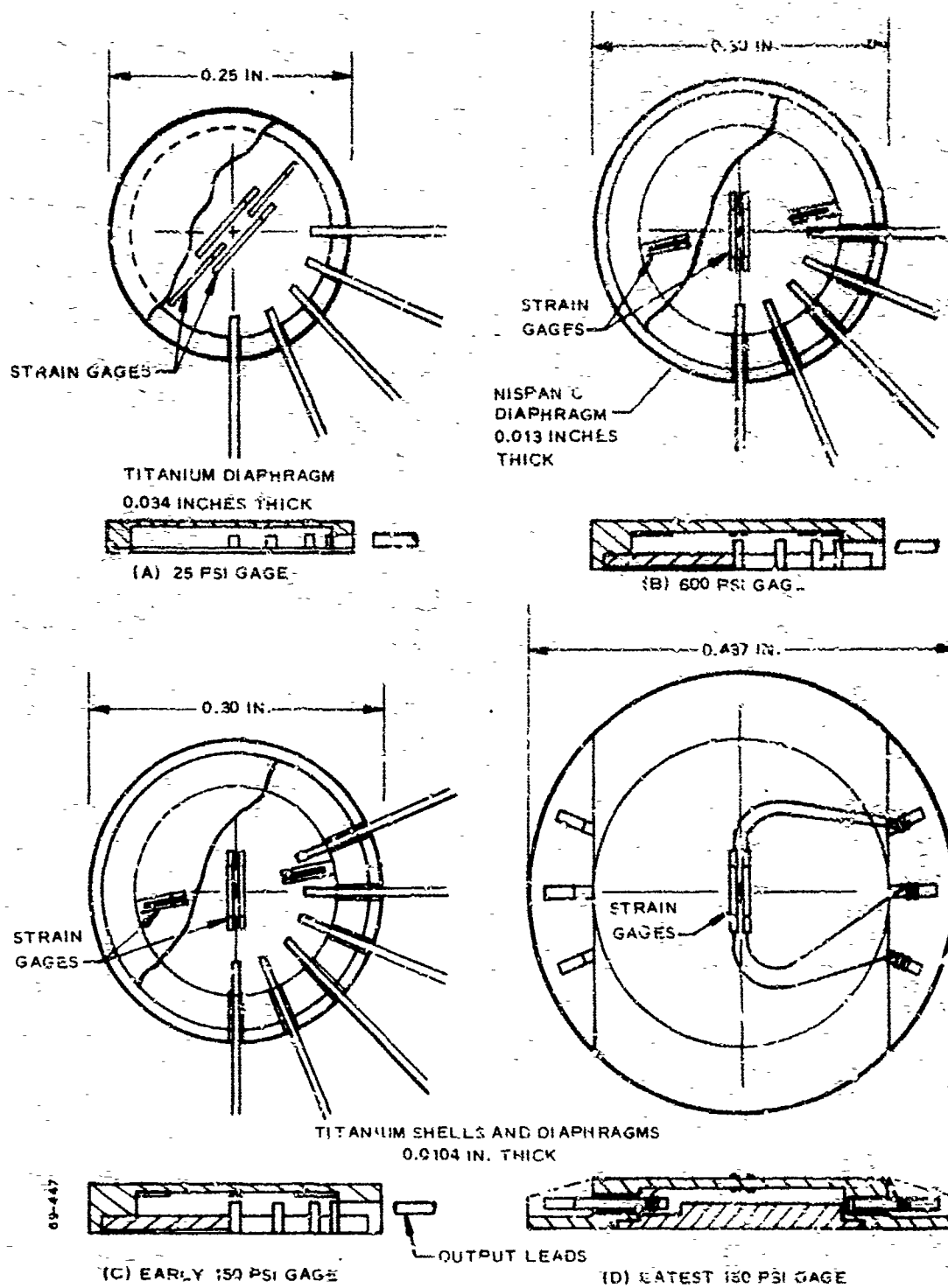
Figure 3-5 Diaphragm Gages Used in STV Program
