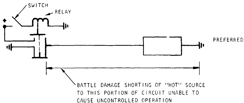
Figure 161. Electrical Circuit Switching Concepts.
