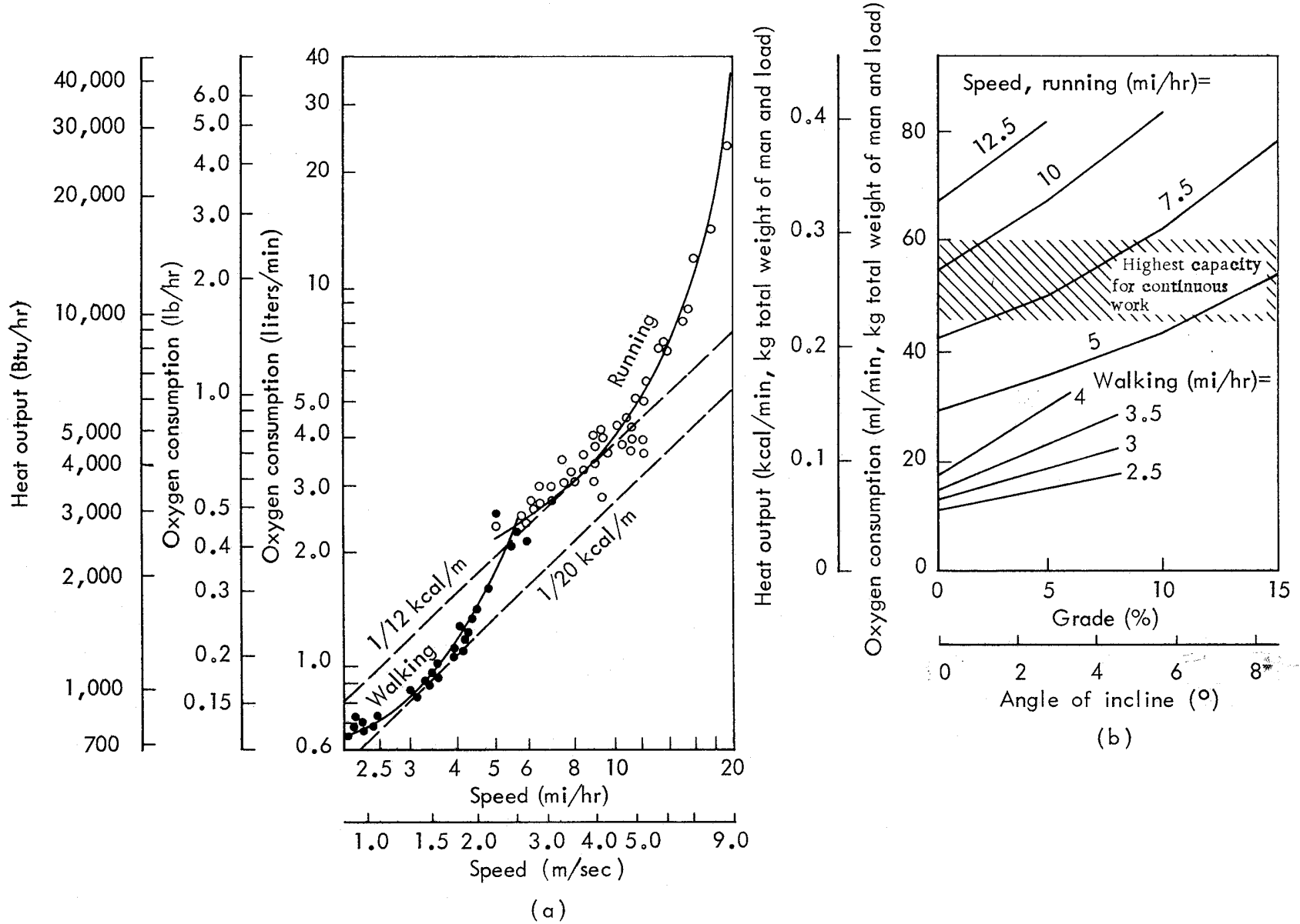
Fig.3—Energy costs of foot travel
