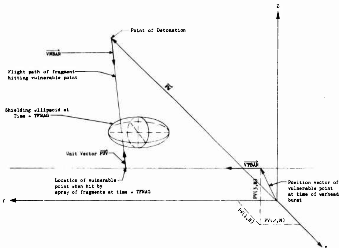
Figure II-10. Shielding Geometry
