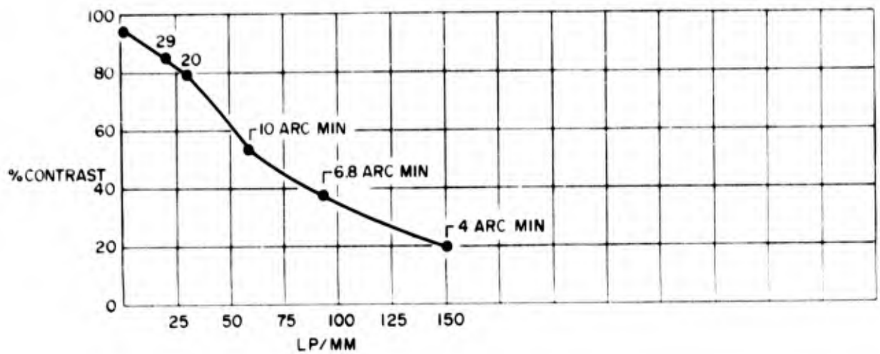
AXIAL CONTRAST TRANSFER PERFORMANCE (MEASURED) \infty TARGET
