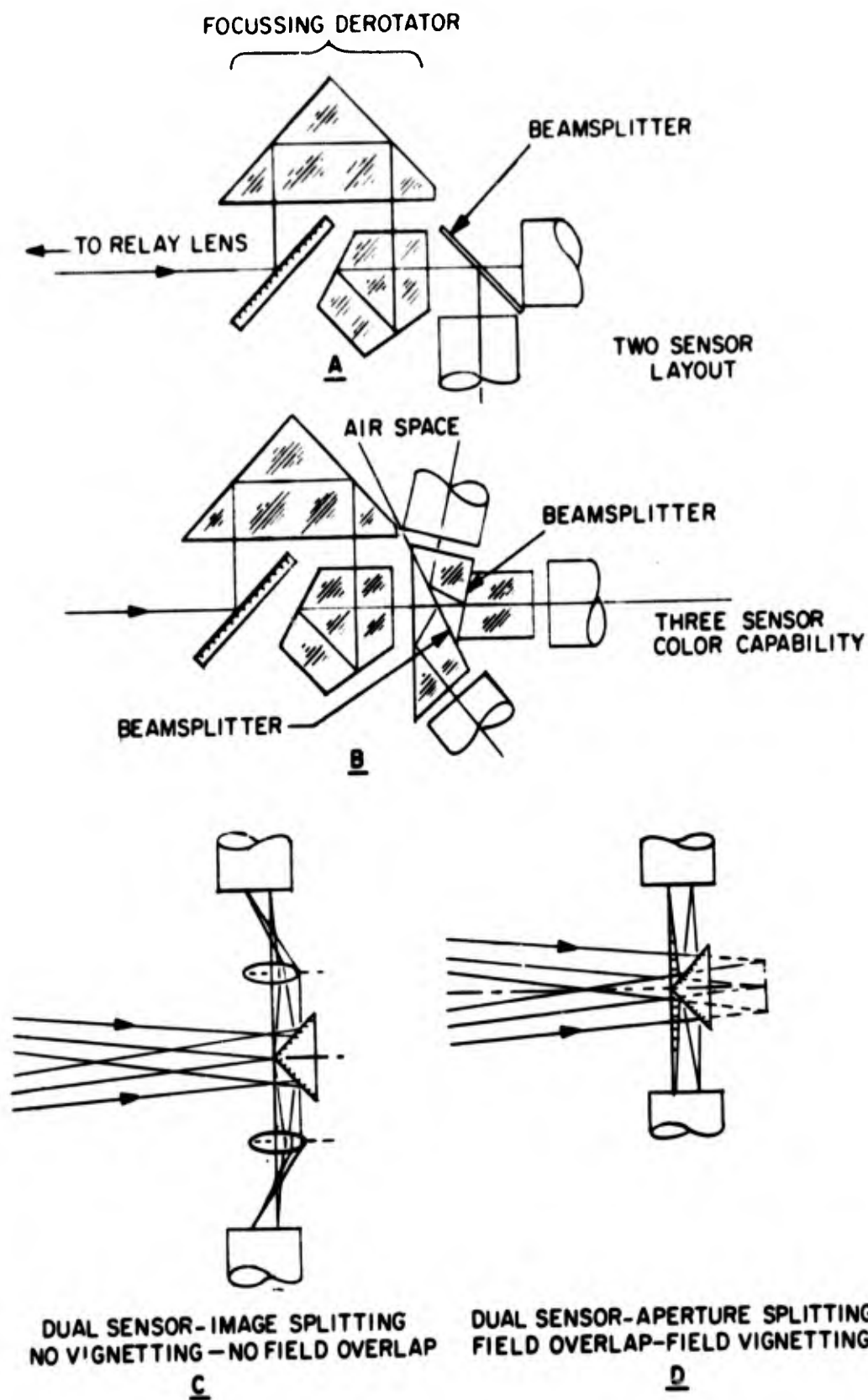
Figure 14. Sensor Interface Configuration
