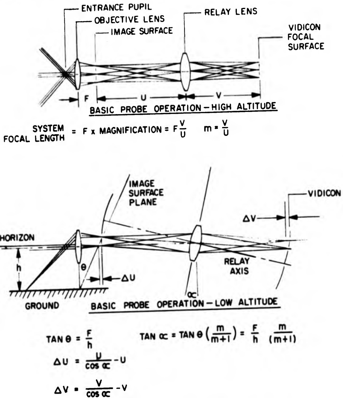
Figure 3. Scheimpflug Probe Geometry for Level Flight Simulation
