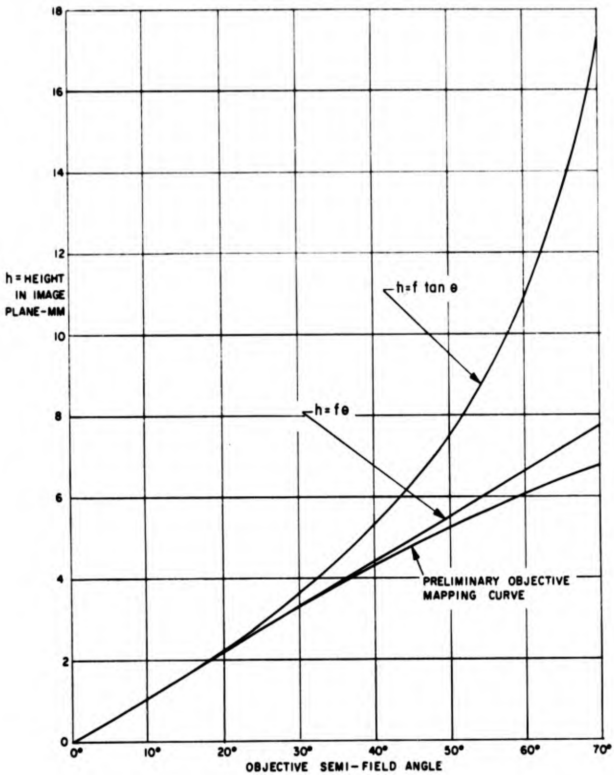
Figure 9. Probe Objective Mapping Functions
