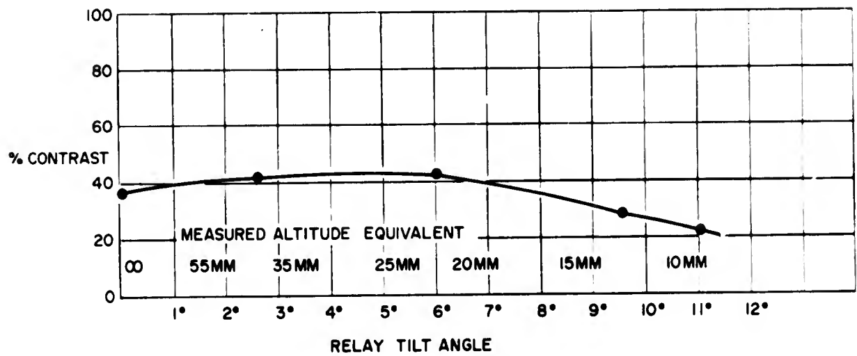
AXIAL CONTRAST TRANSFER VS. RELAY TILT (MEASURED) \infty TARGET, FREQUENCY 92 LP/MM (6.5 ARC MIN. RESOLUTION)
