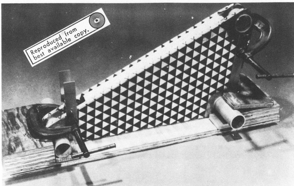
Figure 10. Alignment and Assembly Procedure.
