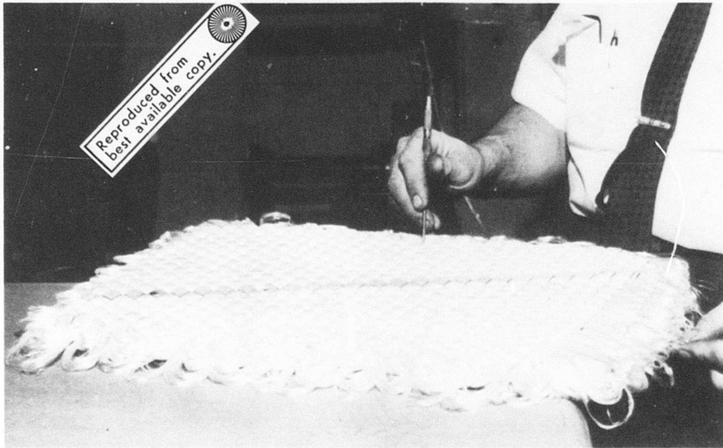
Figure 6. Positioning 20-End S-Glass Roving in Balsa Form.
