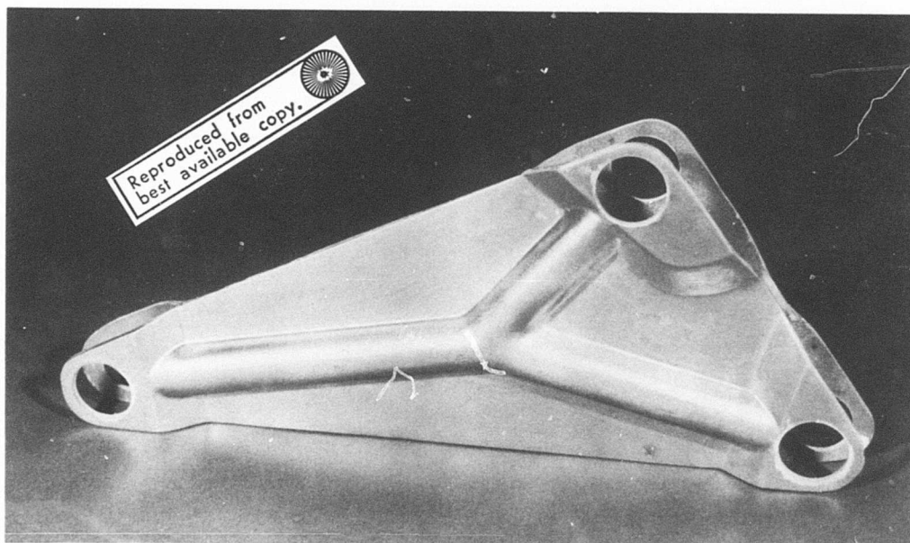
Figure 15. Clamshell Bell Crank After Assembly.
