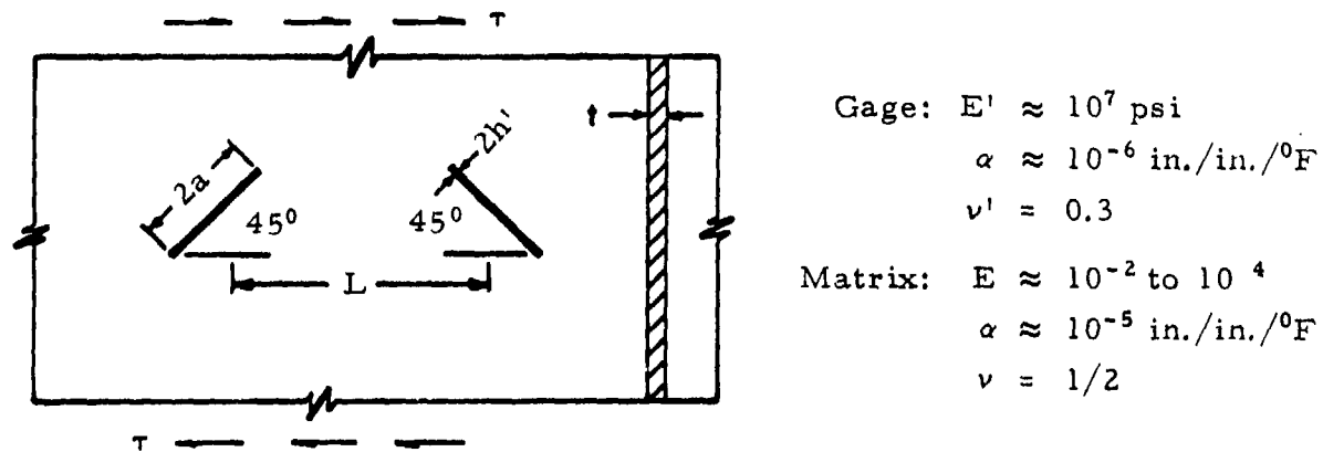
Figure 56. Gage Configuration.
