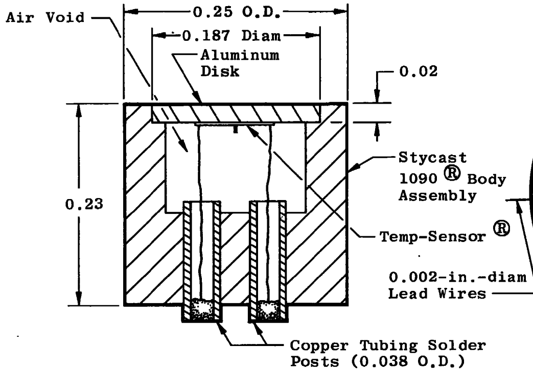
Transducer Assembly
