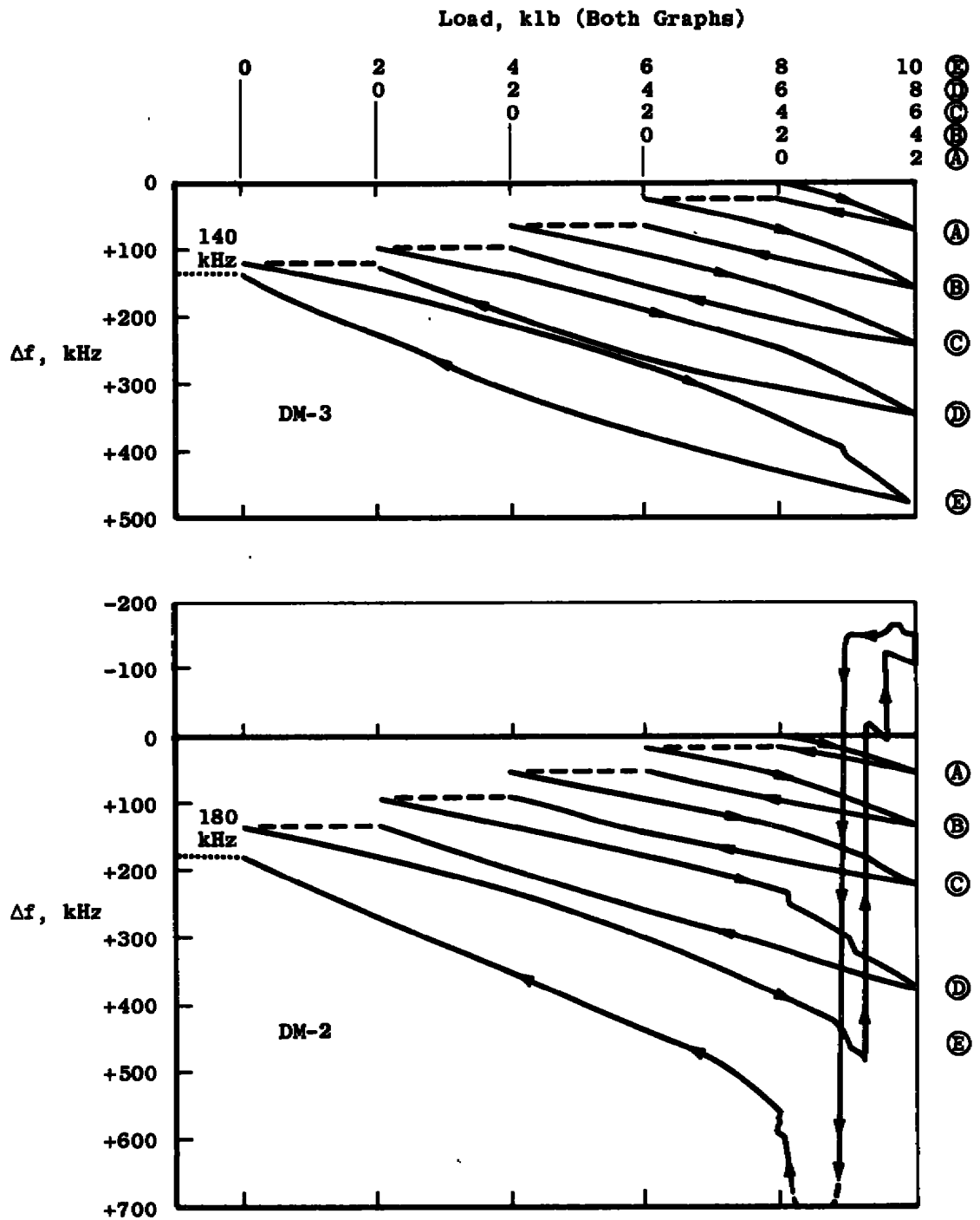
Fig. 14 Load-Frequency Characteristics
