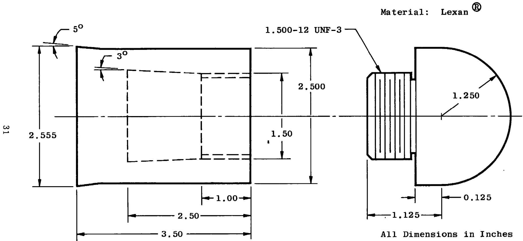
Fig. 1 Impulse Test Model
