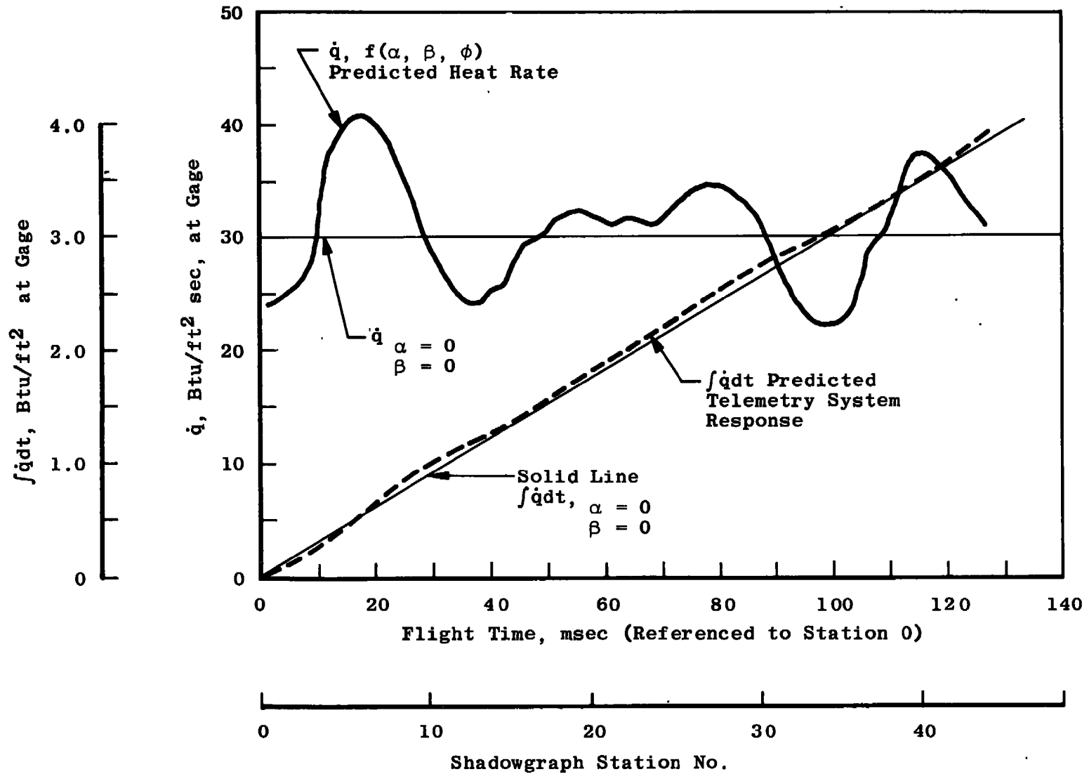
Fig. 20 Shot 2920 Predicted Values
