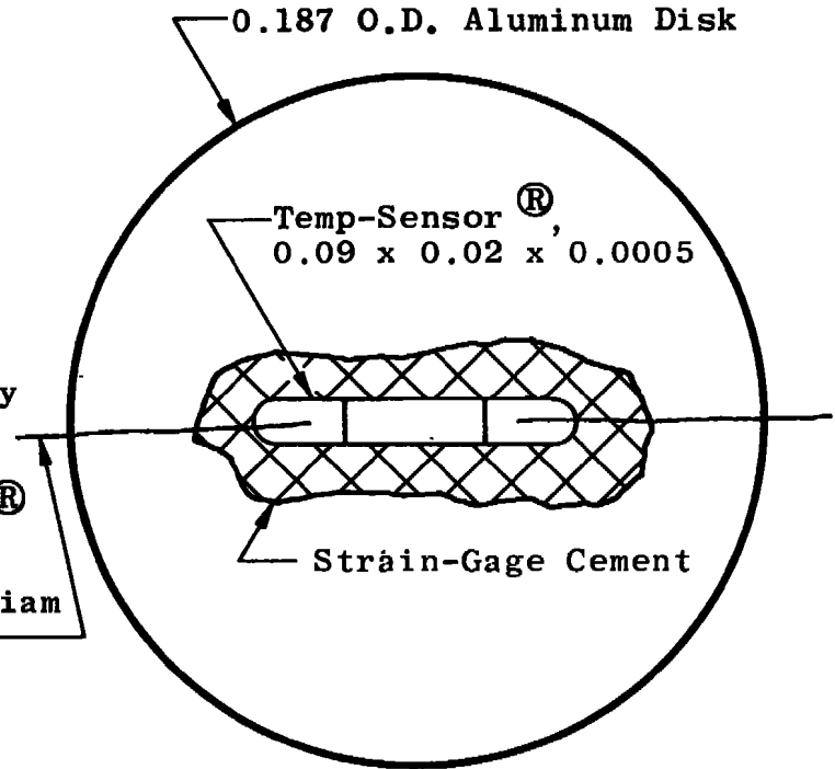
Back View of Sensing Disk
