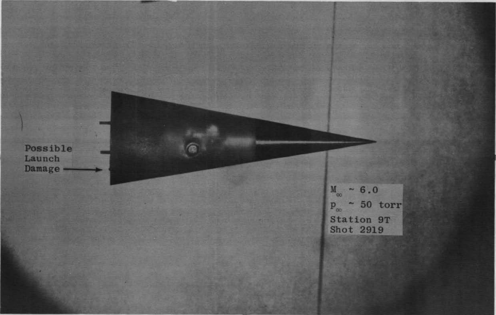
Fig. 25 Shot 2919 Photograph
