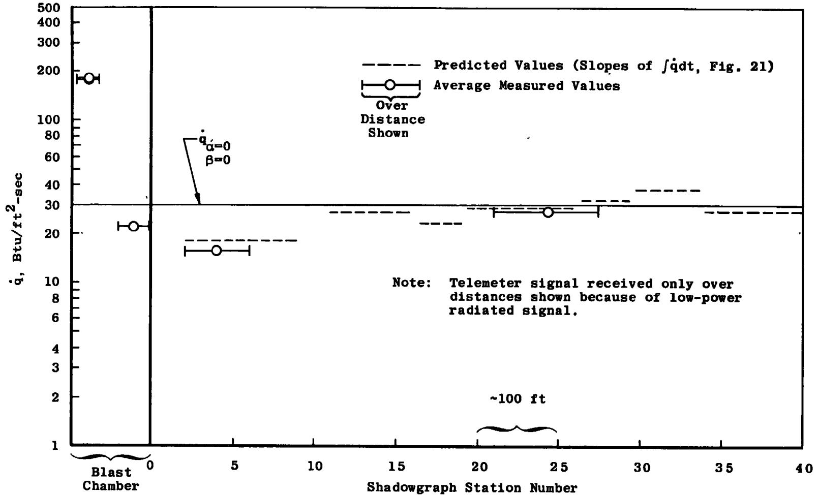
Fig. 22 Comparison of Predicted and Measured Values, Shot 2919
