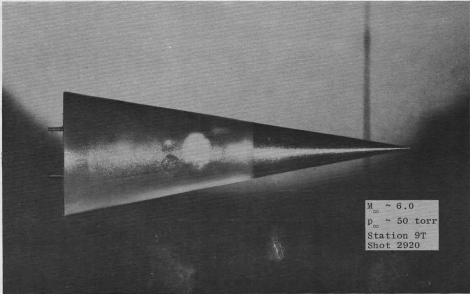
Fig. 26 Shot 2920 Photograph
