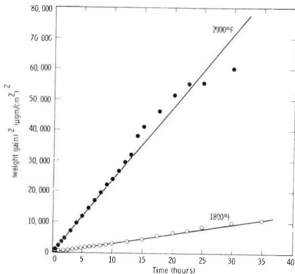
Figure 5.49 — Oxidation of Hot Pressed \text{Si}_3\text{N}_4 in Oxygen at 1 atm
