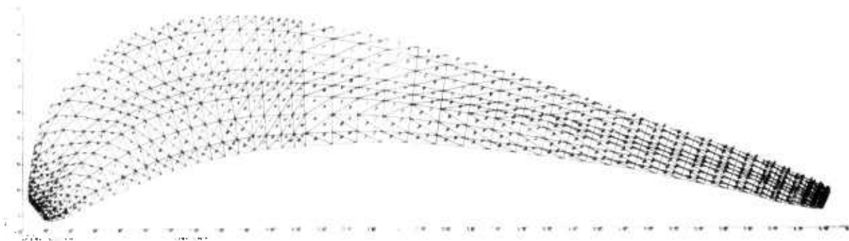
Figure 4.5 — Two-Dimensional Finite Element Mesh for Solid Vane
