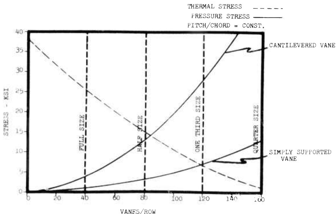
Figure 4.6 — Maximum Stresses in Solid Vane as a Function of Size
