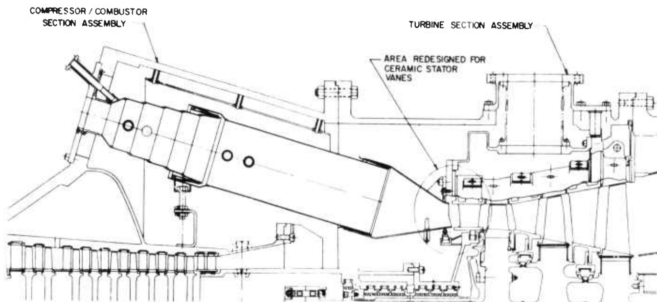
Figure 4.1 — 30Mw Test Turbine Flow Path
