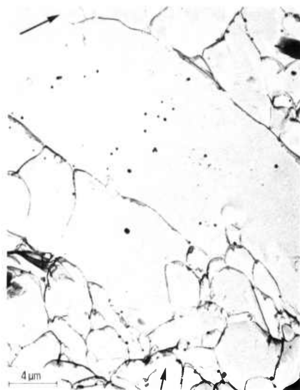
Figure 5.23 — Typical microstructure of hot pressed \text{Si}_3\text{N}_4 . Etched 75 sec. 740°C. Two stage carbon replica
