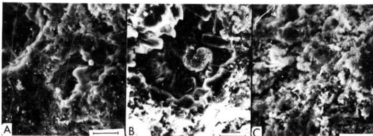
Figure 5.42 — Ford Stator #156. Seanning micrograph of fresh fracture surface, leading edge of blade #17
