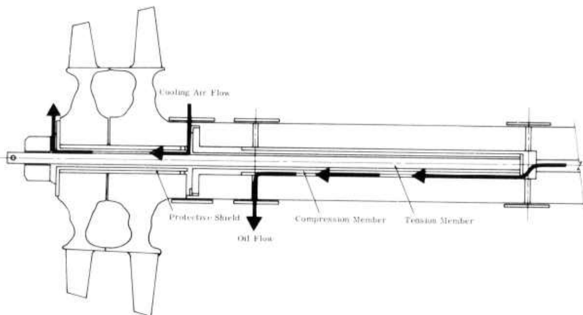
Figure 3.5 — Solid Folded Bolt
