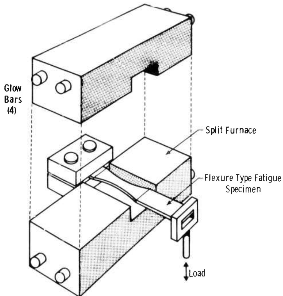
Figure 5.9 — Fatigue Test
