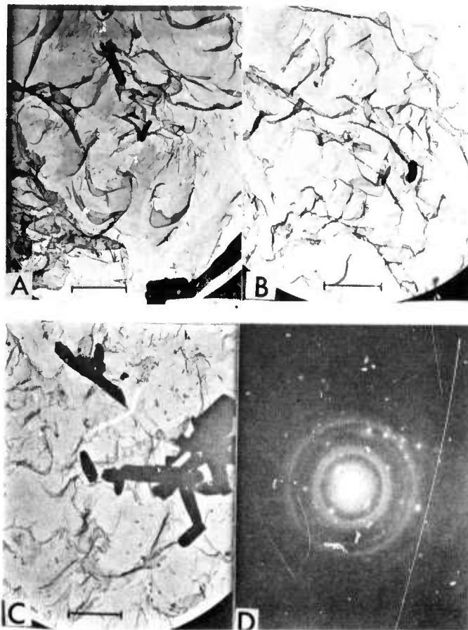
Figure 5.38 — Ford Stator #125, Grid F, white fracture (all \alpha ) A, B, C: Typical surface replicas. Note rugged appearance and elongated \alpha grains (C) D: Diffraction pattern off C. Dominant (100) ZA 5 \mu\text{m} scale bars
