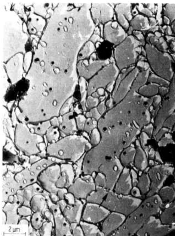
Figure 5.22 — Typical microstructure of hot pressed \text{Si}_3\text{N}_4 . Etched 75 sec. 740°C. Two stage carbon replica
