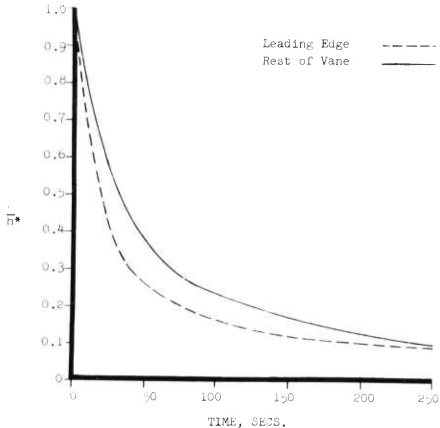
Figure 4.2 — Heat Transfer Coefficient Ratios - vs - Time for a Row 1 Vane Emergency Shutdown Condition
