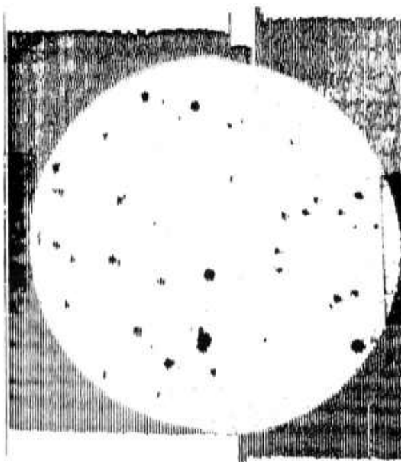
Figure 5.55 — C-Scan of Lithium Aluminum Silicate Disks
