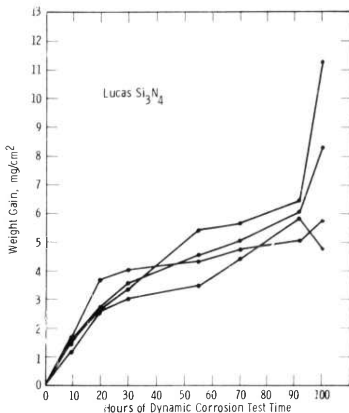
Figure 5.17 — Weight Change vs Hours of Exposure Time for Si 3 N 4 Tested at 2000°F and 3 Atmospheres
