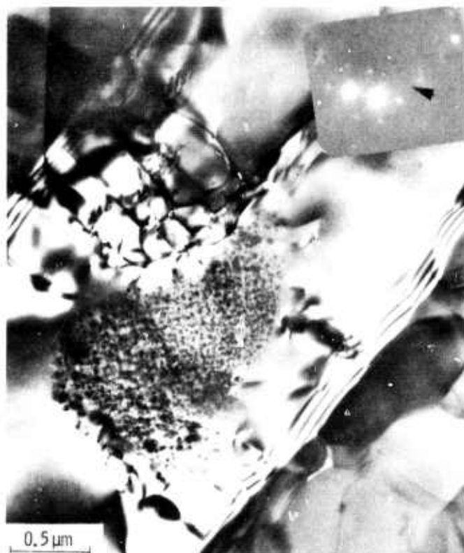
Figure 5.26 — Dark field image of \bar{g} showing a cluster of impurities (a grain, 800 kV)
