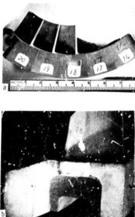
Figure 5.35 — Ford Stator #156, fresh fracture surface of blade #17 examined by replica and scanning electron microscopy and white and grey areas from which replication grids and x-ray sample were taken
