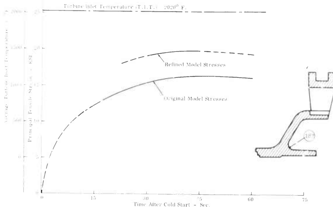
Figure 3.40 — Comparison of Stresses in Original Model and Refined Model - Nose Cone Element 187 - Silieon Carbide
