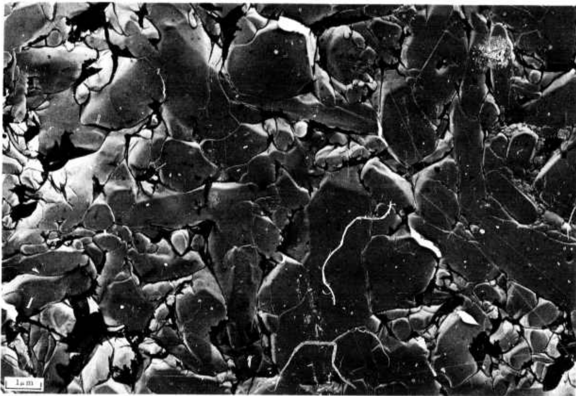
Figure 3.7 — Electron Micrograph 17,300X of Etched Norton Hot Pressed Silicon Nitride
