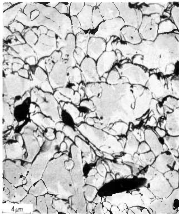
Figure 5.21 — Typical microstructure of hot pressed \text{Si}_3\text{N}_4 . Etched 75 sec. 740°C. Two stage carbon replica
