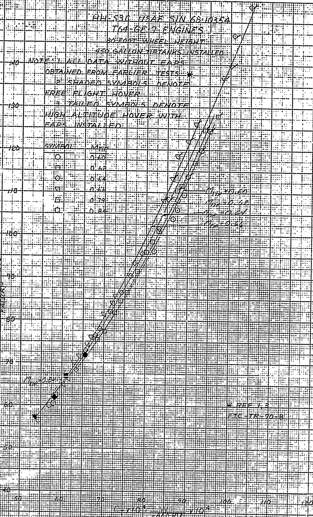
Figure 4 Nondimensional Hovering Performance
