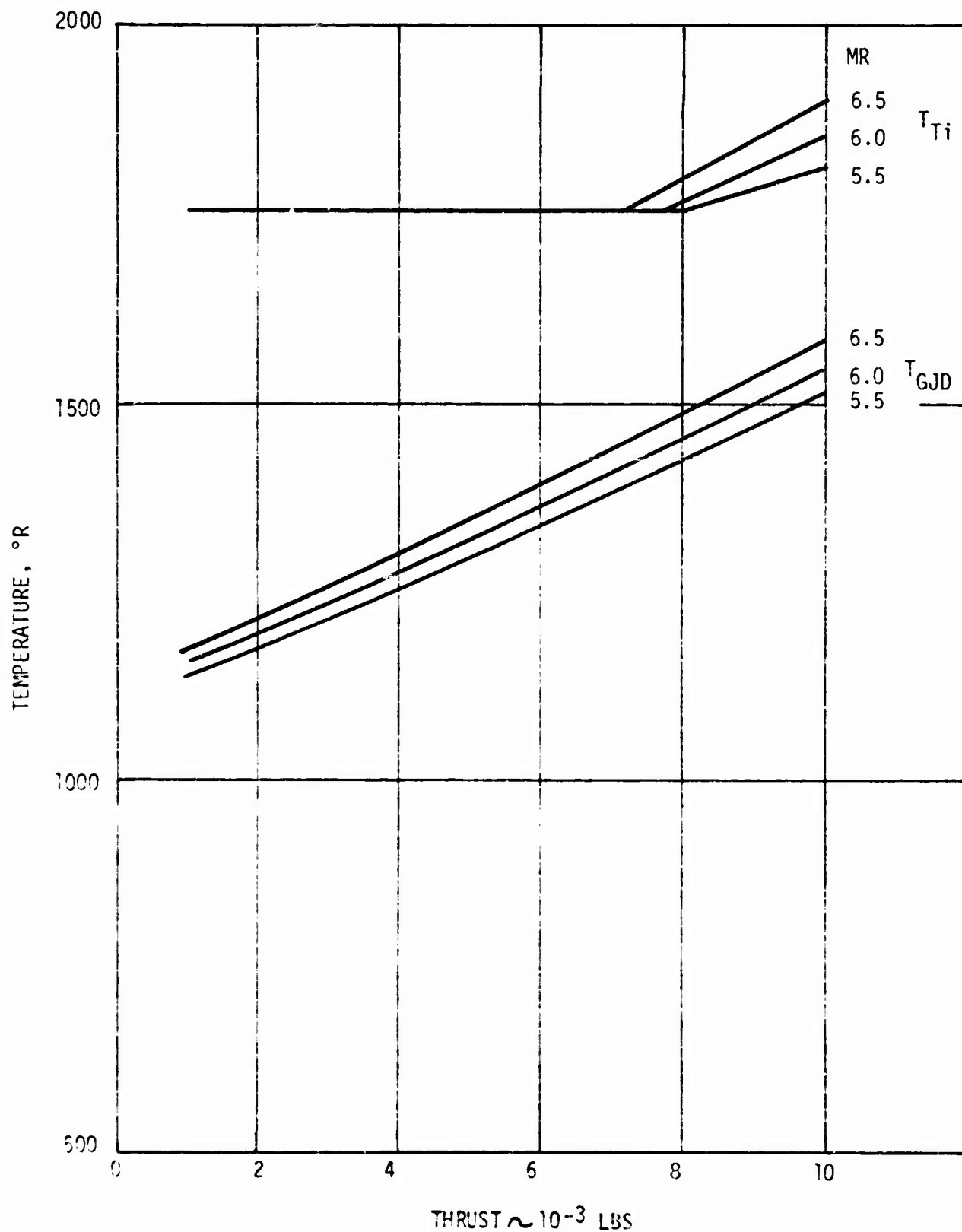
Figure 297. Turbine Inlet Temperature and Gas Inlet Temperature vs Thrust and Mixture Ratio
