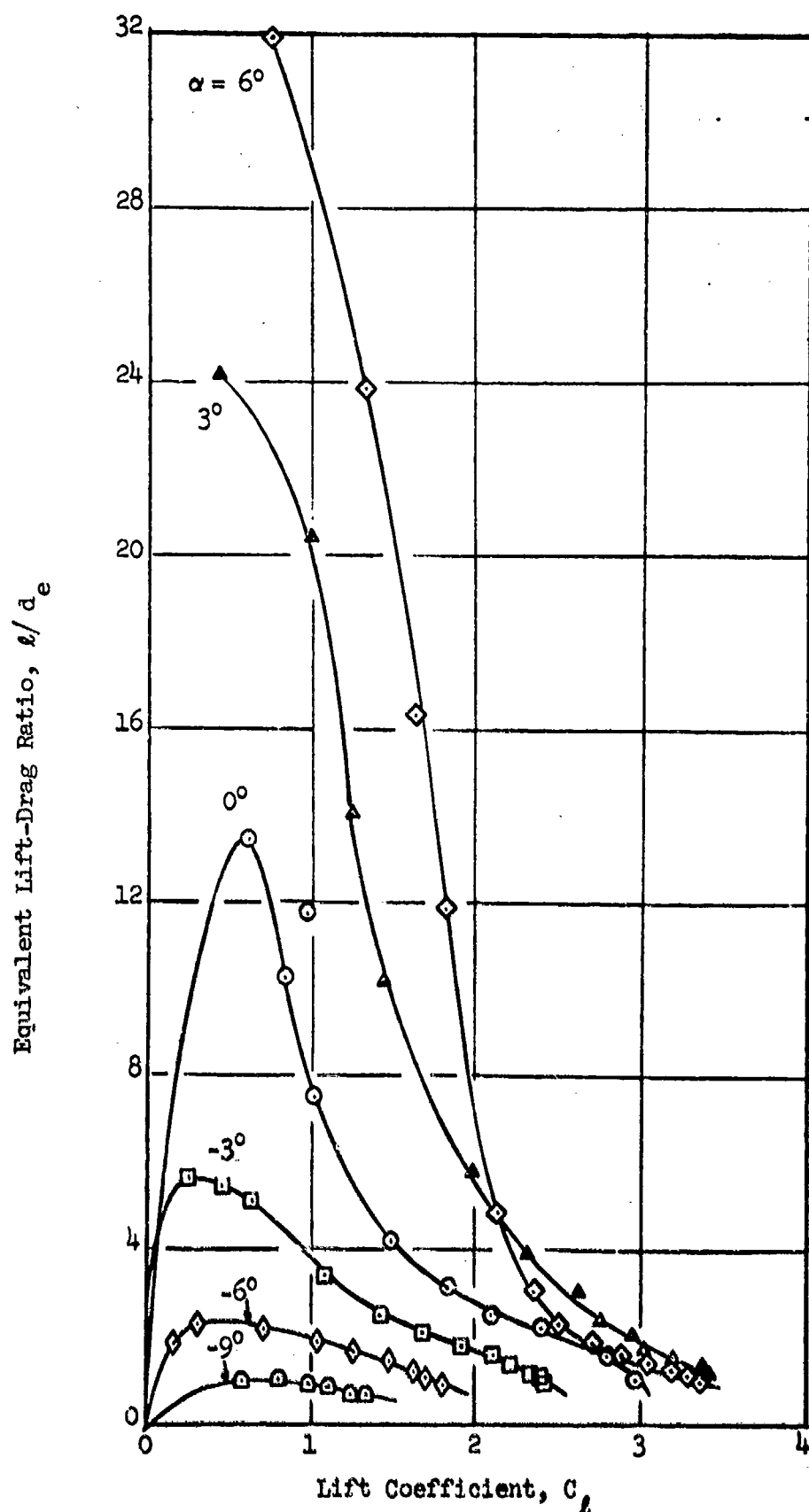
Figure 17 - Equivalent Lift-Drag Ratio for the Pure Ellipse, h = 0.025 inch
