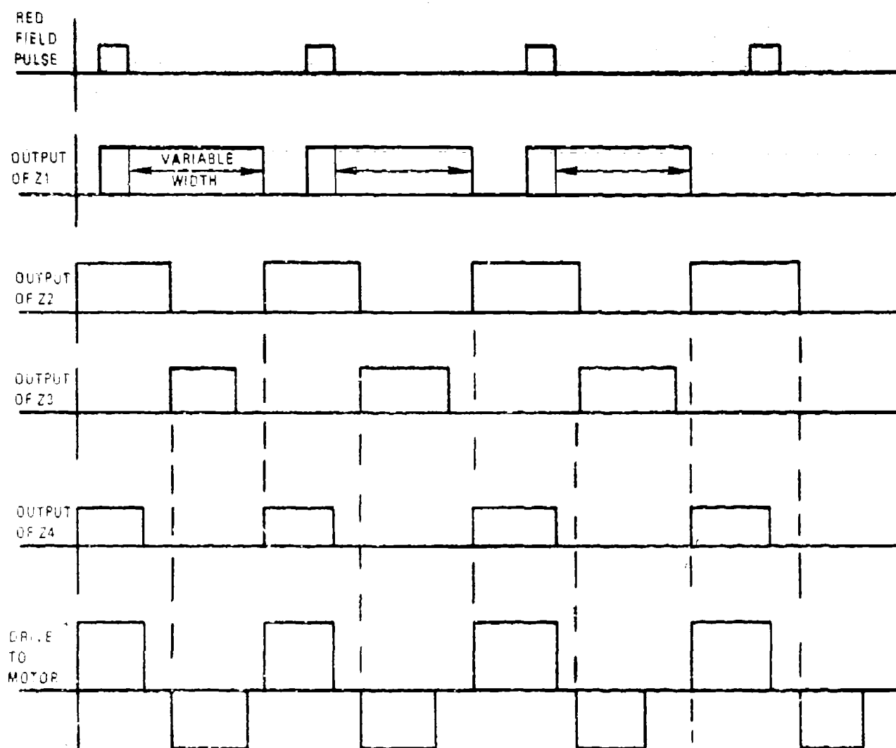
TIMING DIAGRAM
