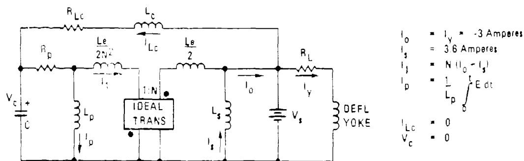
Figure 87 Equivalent Transformer Circuit During First Part of Trace Period
