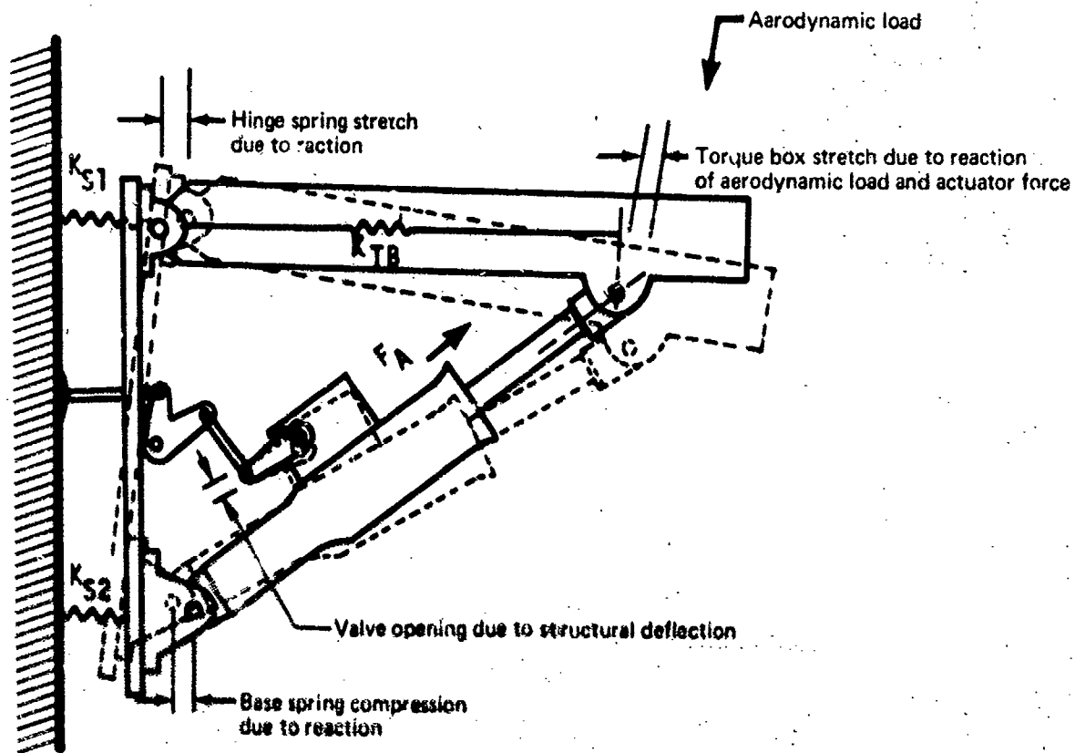
FIGURE 76.—STRUCTURAL FEEDBACK
