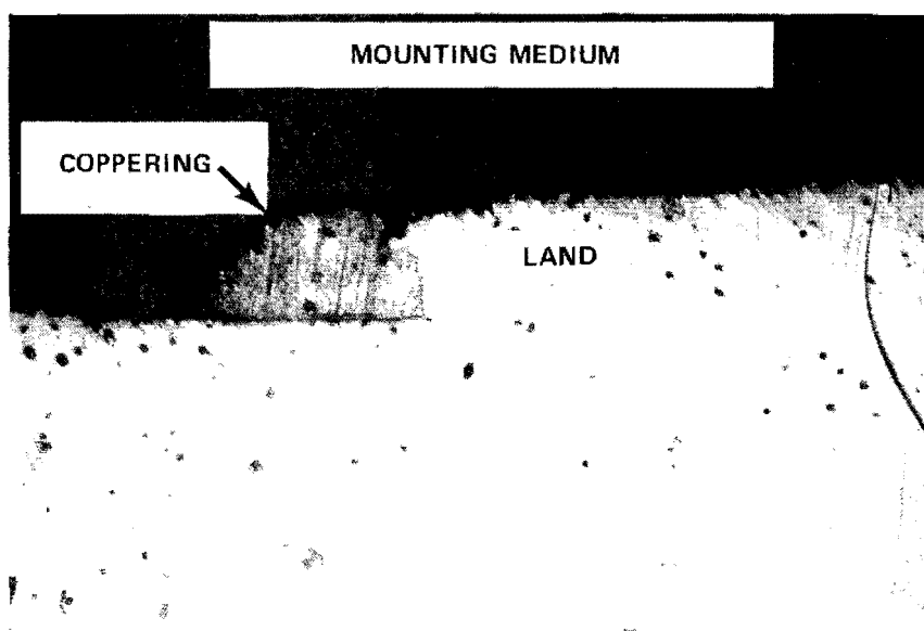
Figure I-17. Section B-B, Barrel No. 10 (50X)
