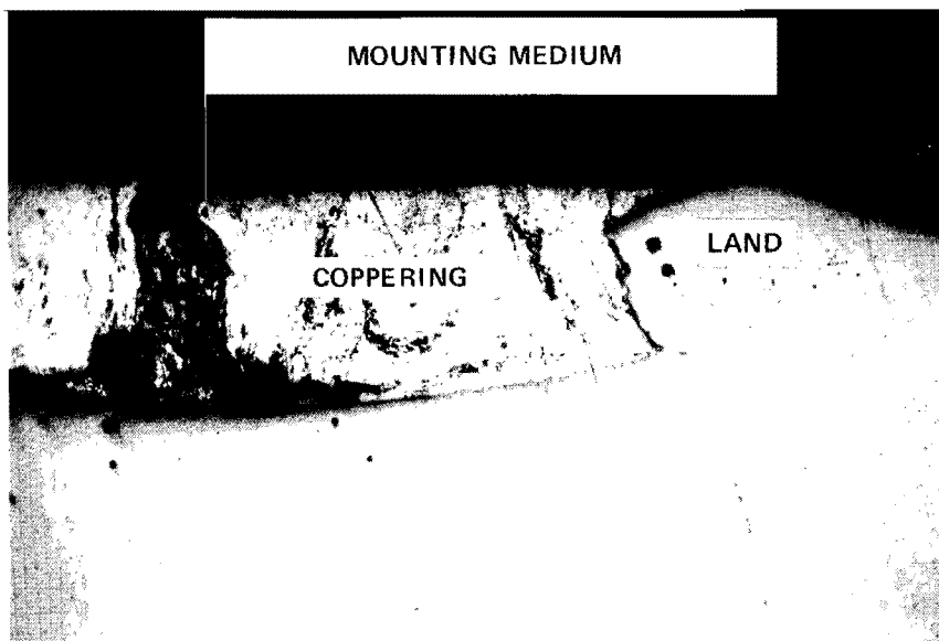
Figure I-23. Section B-B, Barrel No. 11 (50X)
