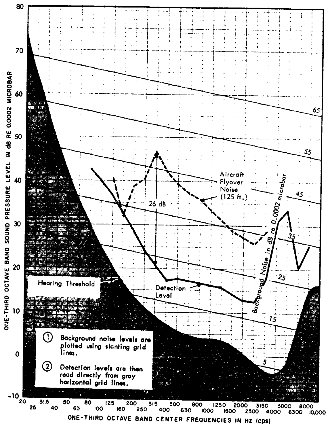
FIGURE 14. PREDICTED DETECTION LEVEL EXAMPLE FOR AIRCRAFT FLYOVER NOISE IN NOISE BACKGROUND
