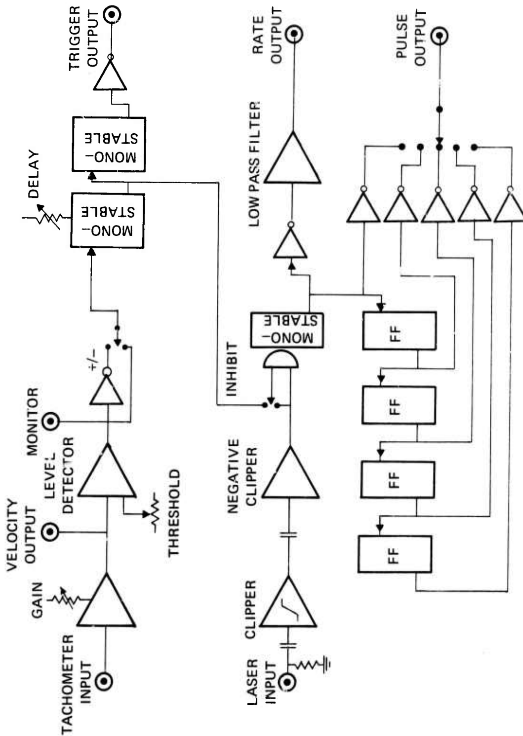
FIGURE 3.7.1 SLIDE VELOCITY TEST SET, BLOCK DIAGRAM
