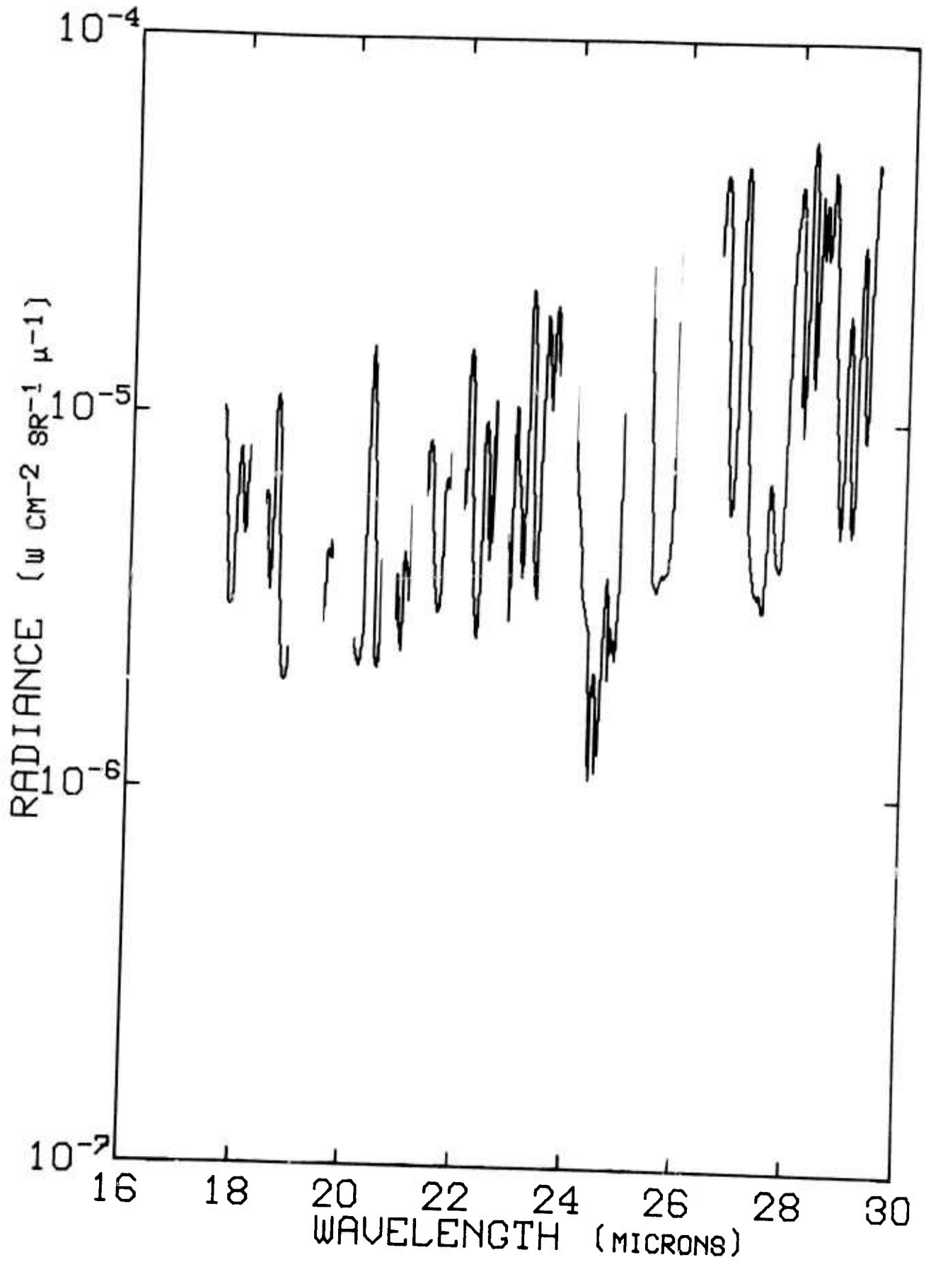
Figure 183. Radiance vs Wavelength at 29.5 kft and 0321 ADT, 23 September 1971.
