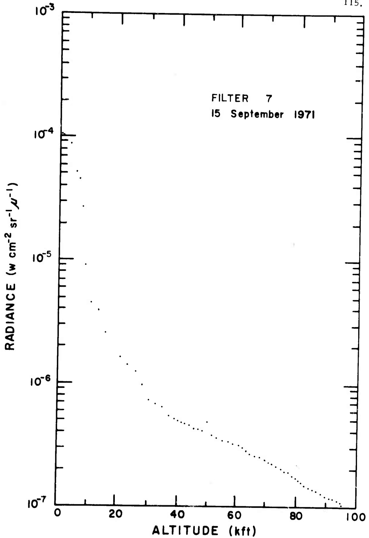
Figure 102. Radiance vs Altitude for Filter 7, 15 September 1971.
