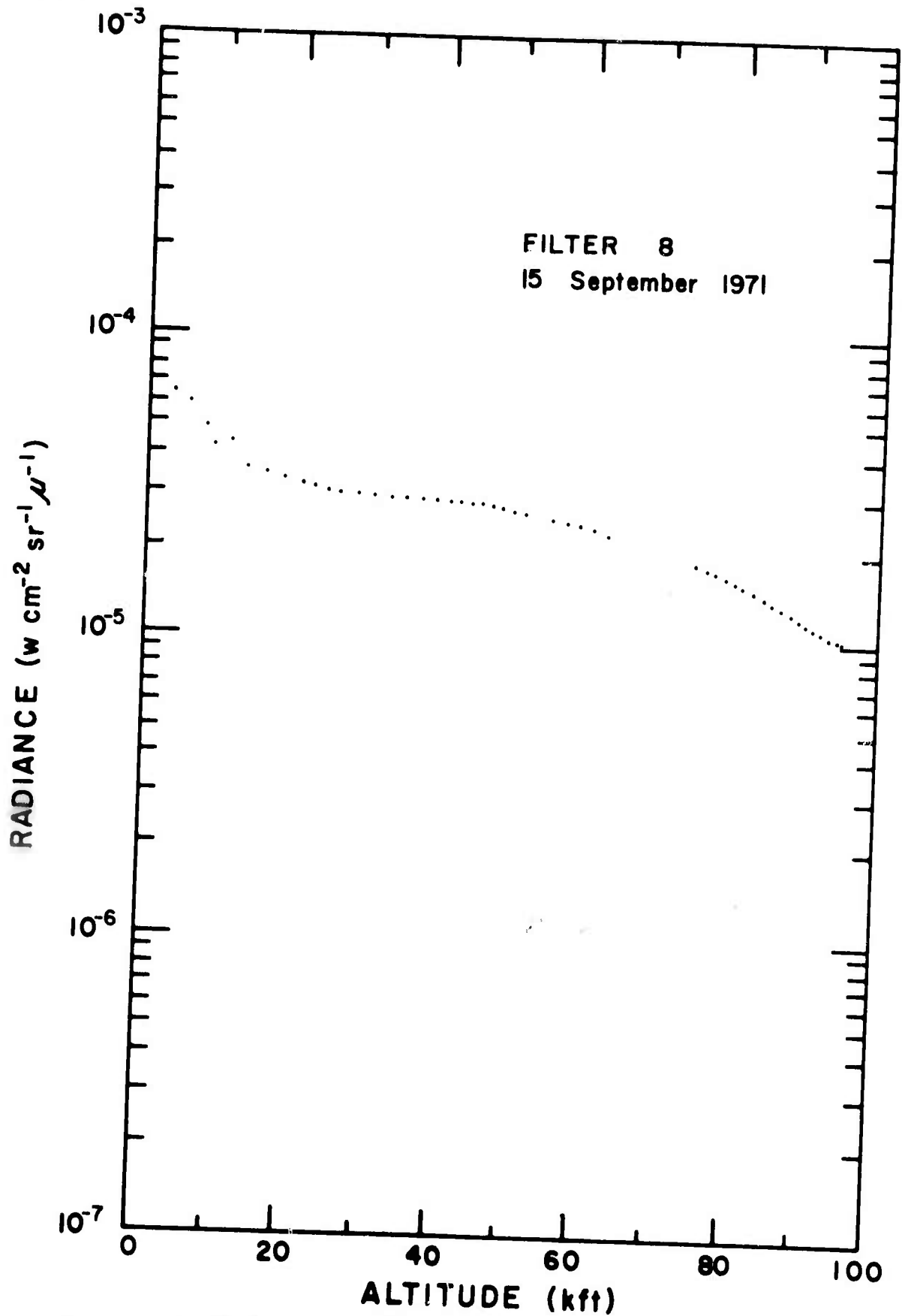
Figure 99. Radiance vs Altitude for Filter 8, 15 September 1971.
