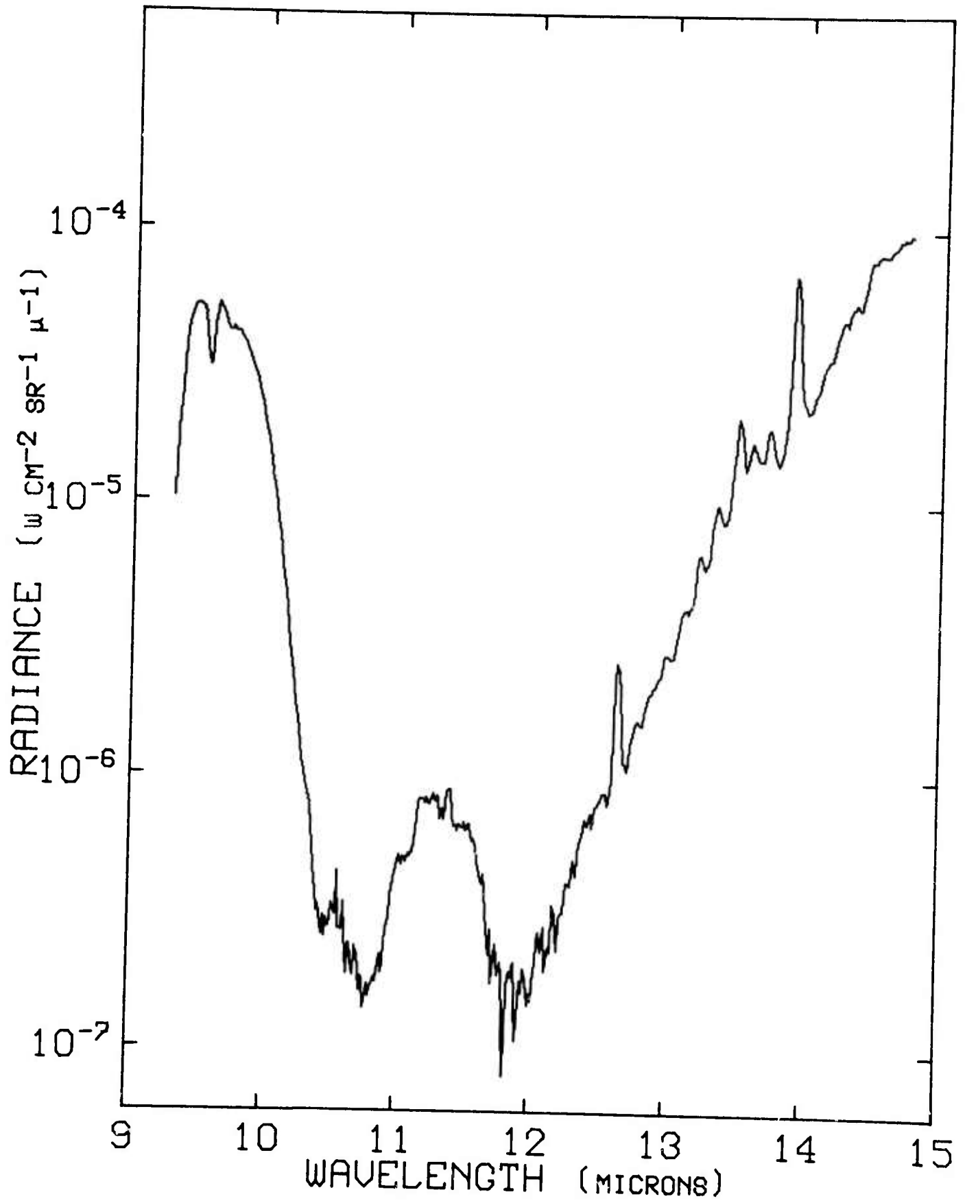
Figure 142. Radiance vs Wavelength at 71.8 kft and 0210 ADT, 15 September 1971.
