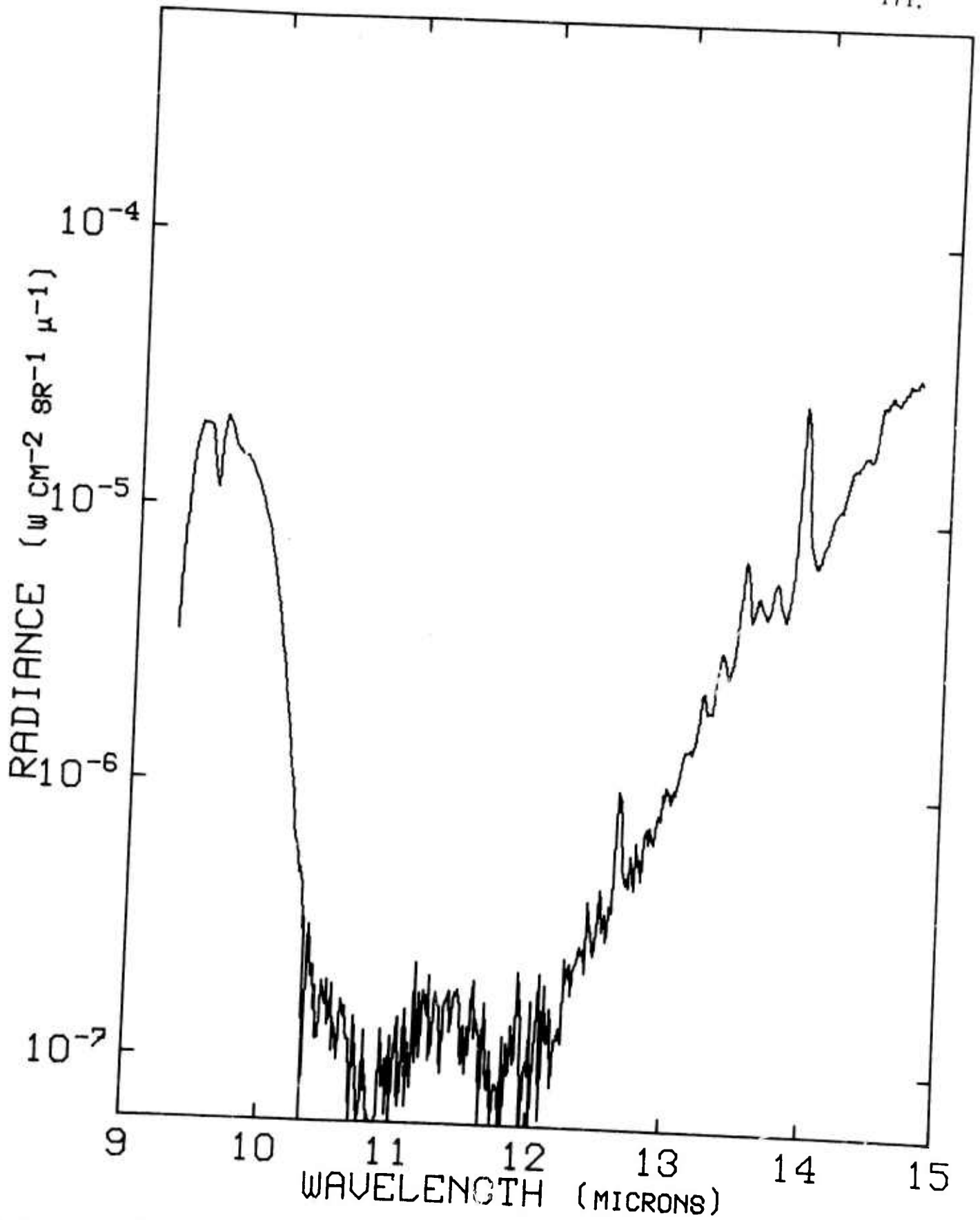
Figure 158. Radiance vs Wavelength at 93.2 kft and 0241 ADT, 15 September 1971.
