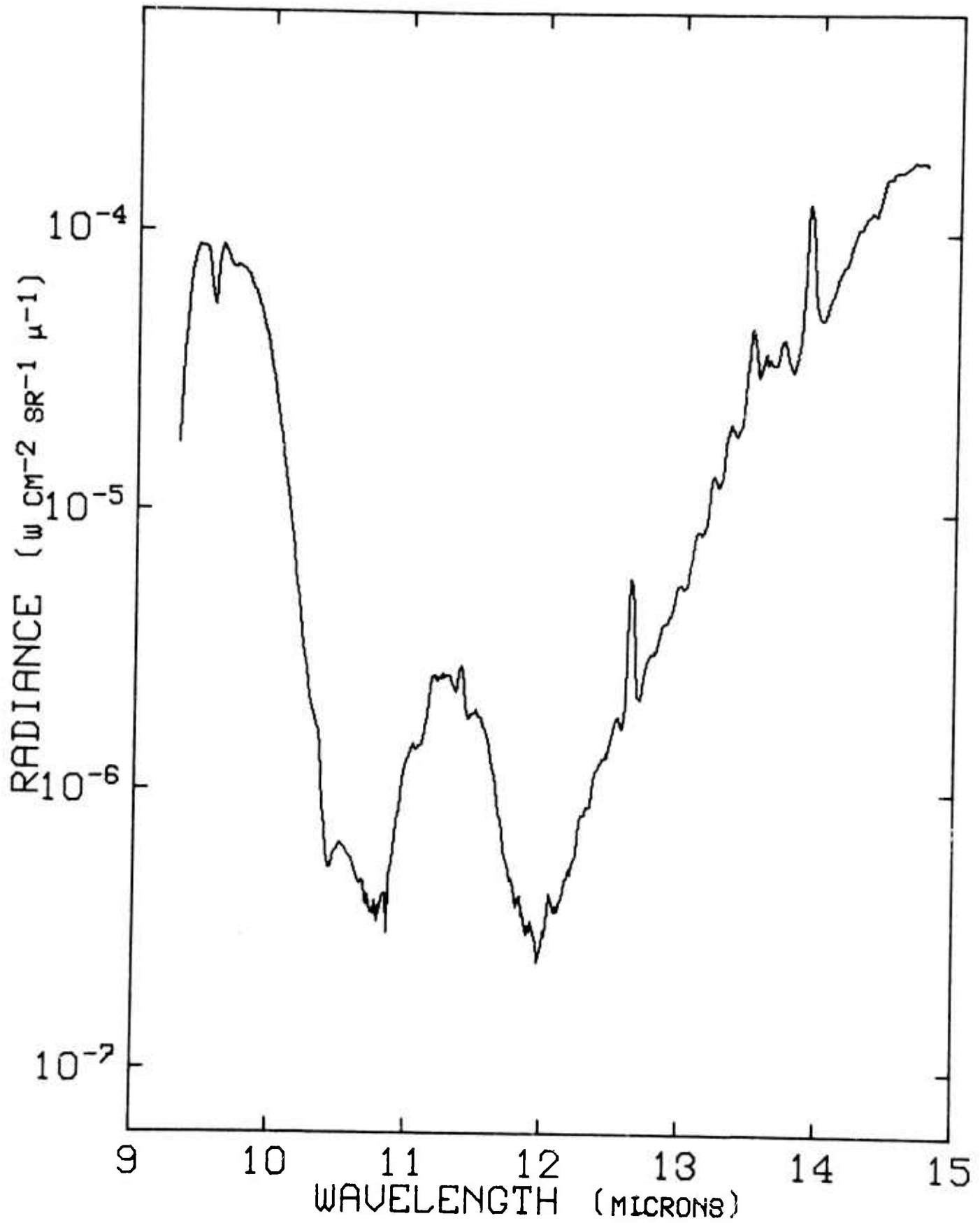
Figure 131. Radiance vs Wavelength at 53.4 kft and 0149 ADT, 15 September 1971.
