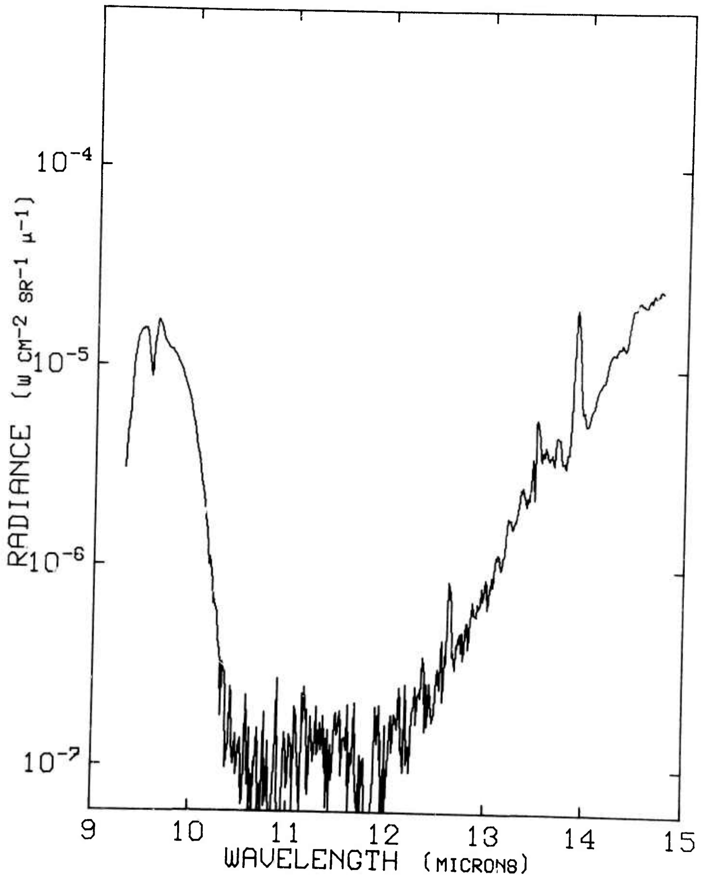
Figure 76. Radiance vs Wavelength at 95.4 kft and 0422 ADT, 12 September 1971.
