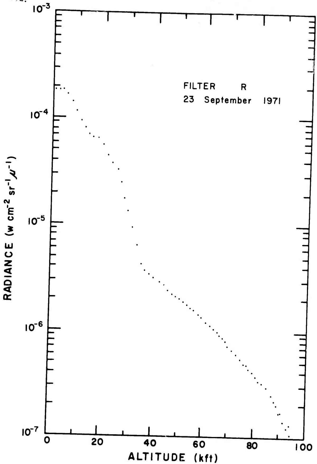
Figure 179. Radiance vs Altitude for Filter R, 23 September 1971.
