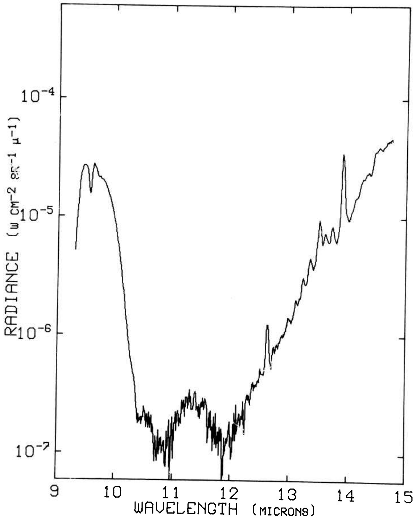
Figure 153. Radiance vs Wavelength at 86.5 kft and 0231 ADT, 15 September 1971.
