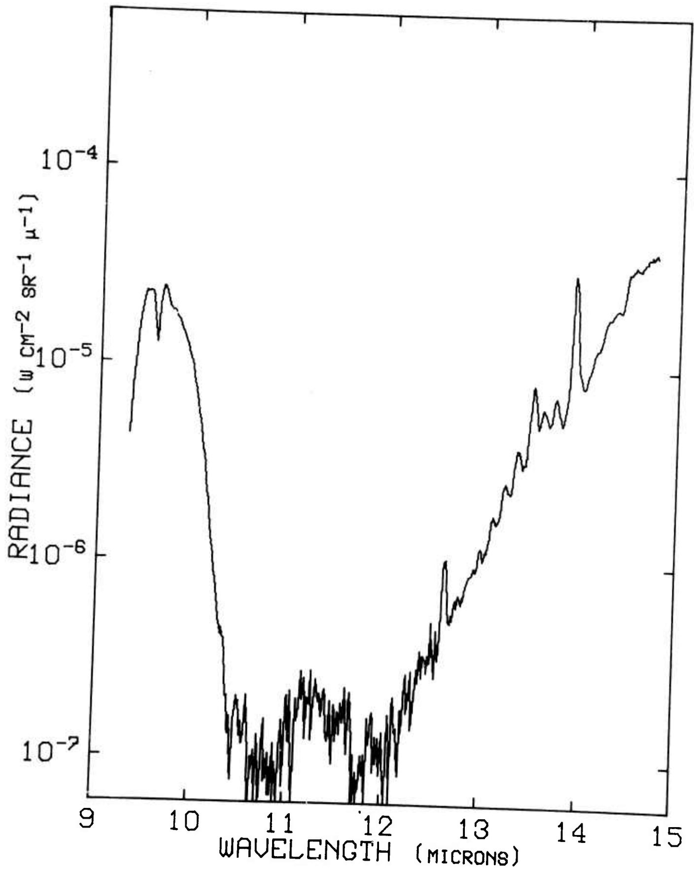
Figure 155. Radiance vs Wavelength at 89.6 kft and 0235 ADT, 15 September 1971.
