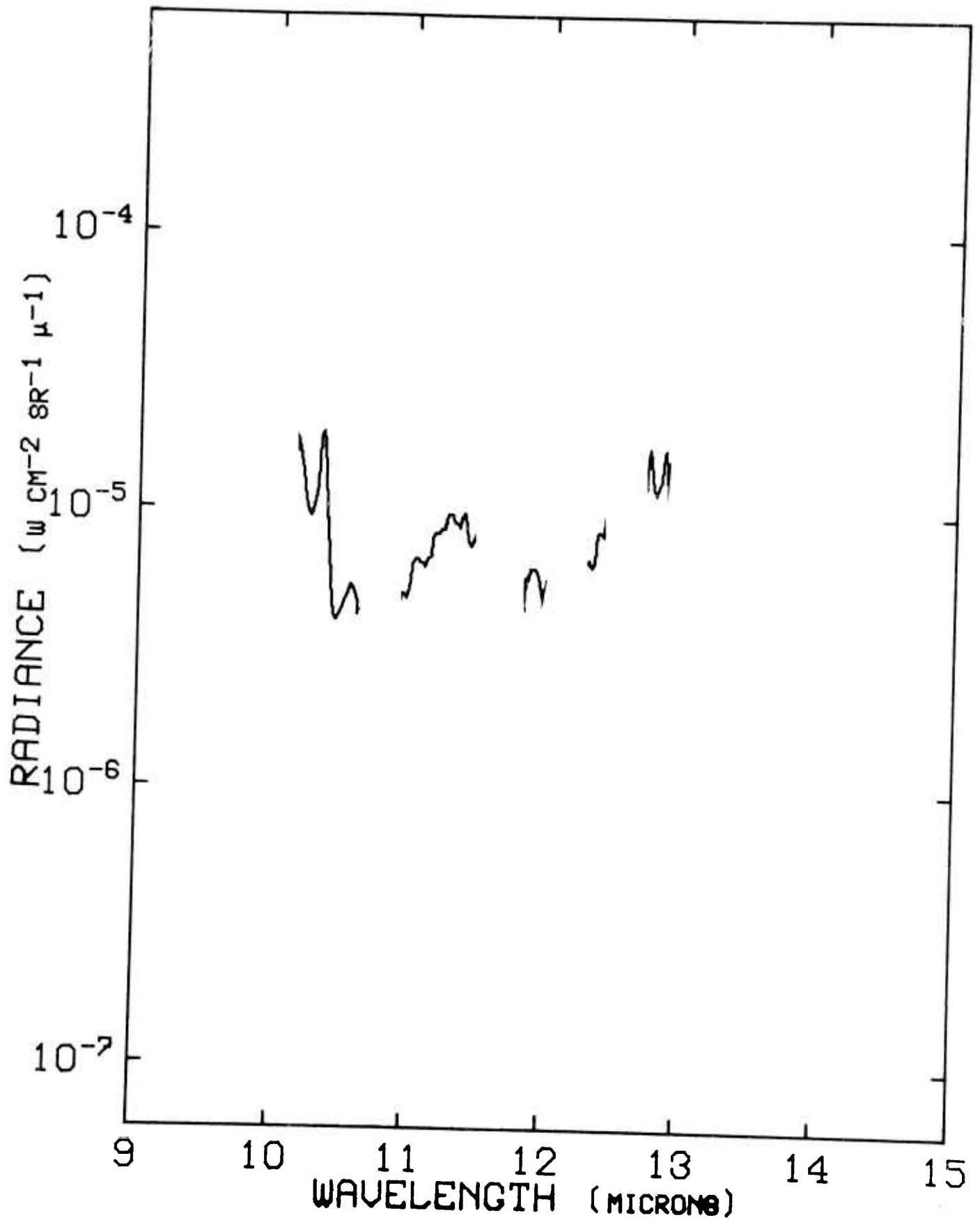
Figure 26. Radiance vs Wavelength at 20.7 kft and 0151 ADT, 12 September 1971.
