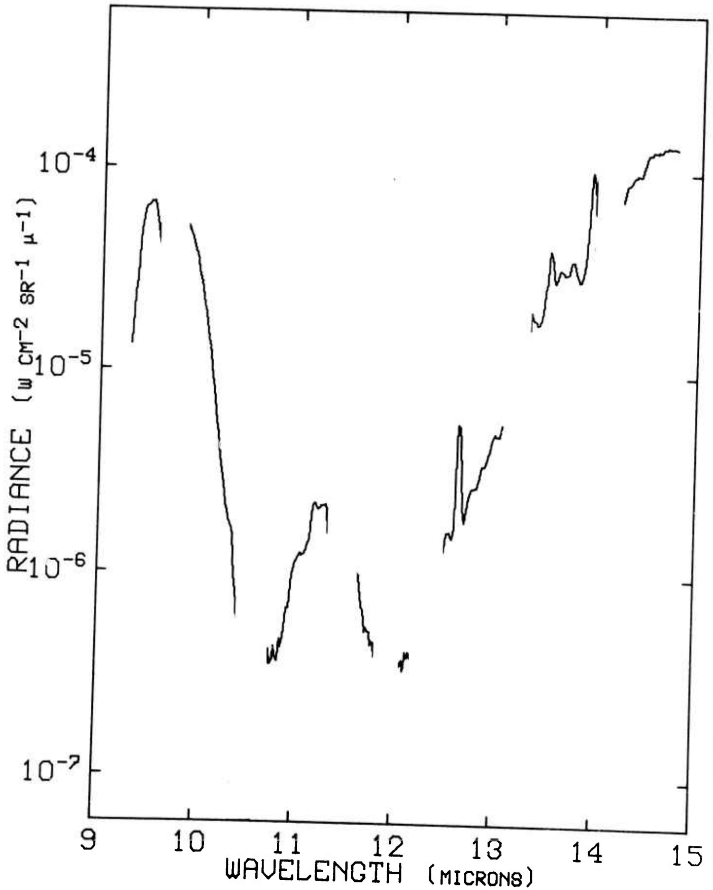
Figure 40. Radiance vs Wavelength at 48.9 kft and 0239 ADT, 12 September 1971.
