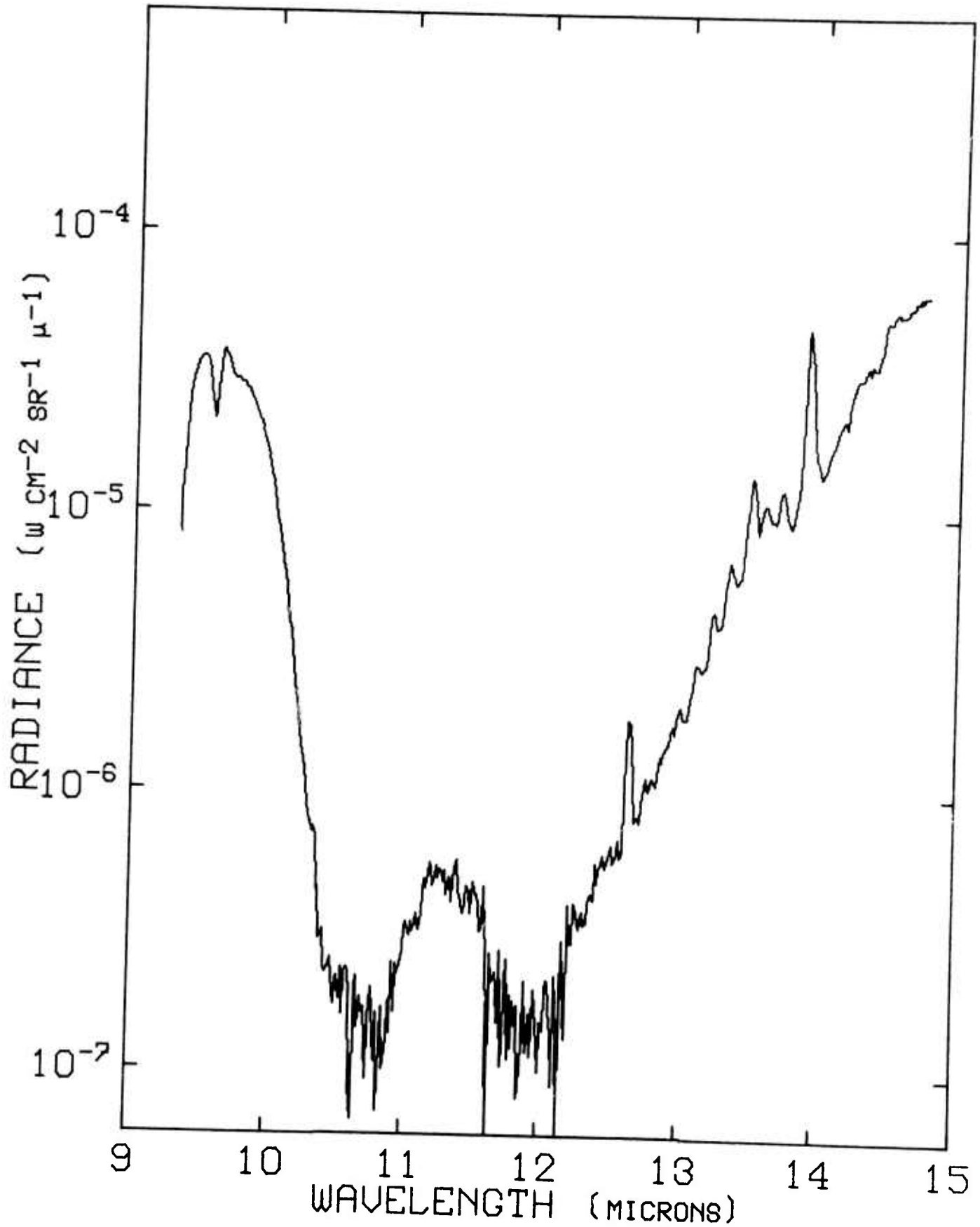
Figure 58. Radiance vs Wavelength at 74.4 kft and 0324 ADT, 12 September 1971.
