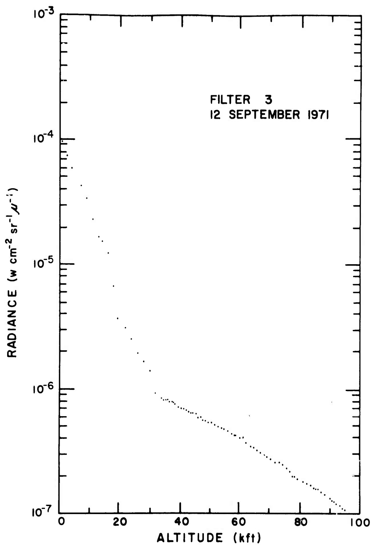
Figure 6. Radiance vs Altitude for Filter 3, 12 September 1971.
