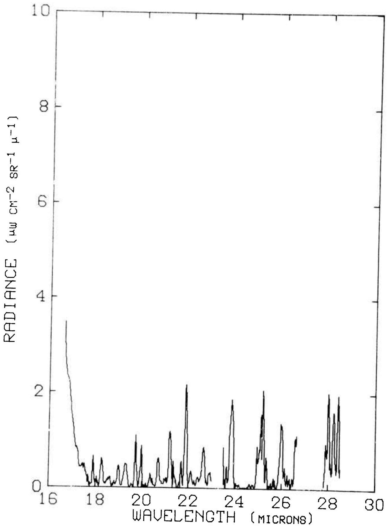
Figure 213. Radiance vs Wavelength at 93.0 kft and 0444 ADT, 23 September 1971.
