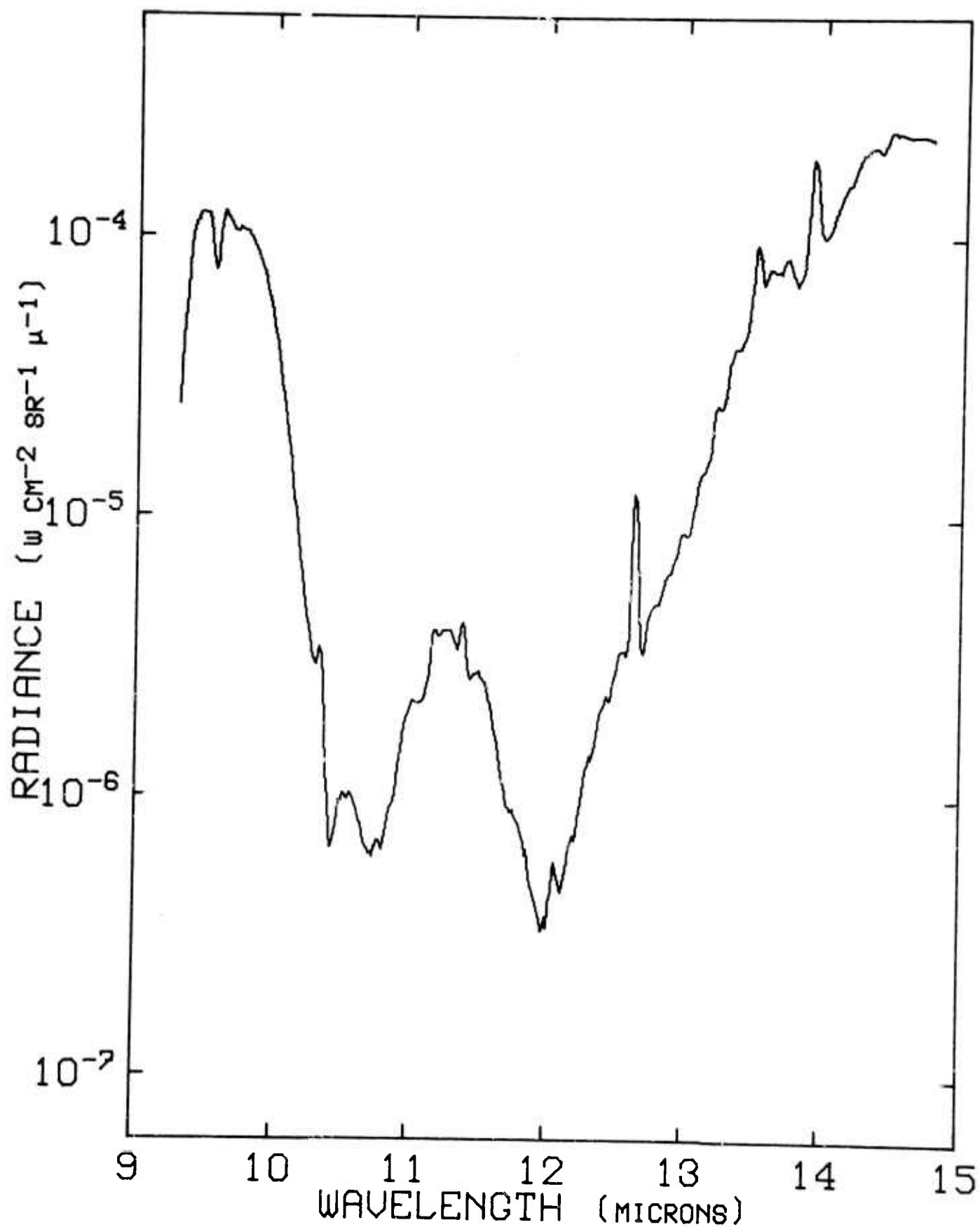
Figure 120. Radiance vs Wavelength at 35.1 kft and 0128 ADT, 15 September 1971.
