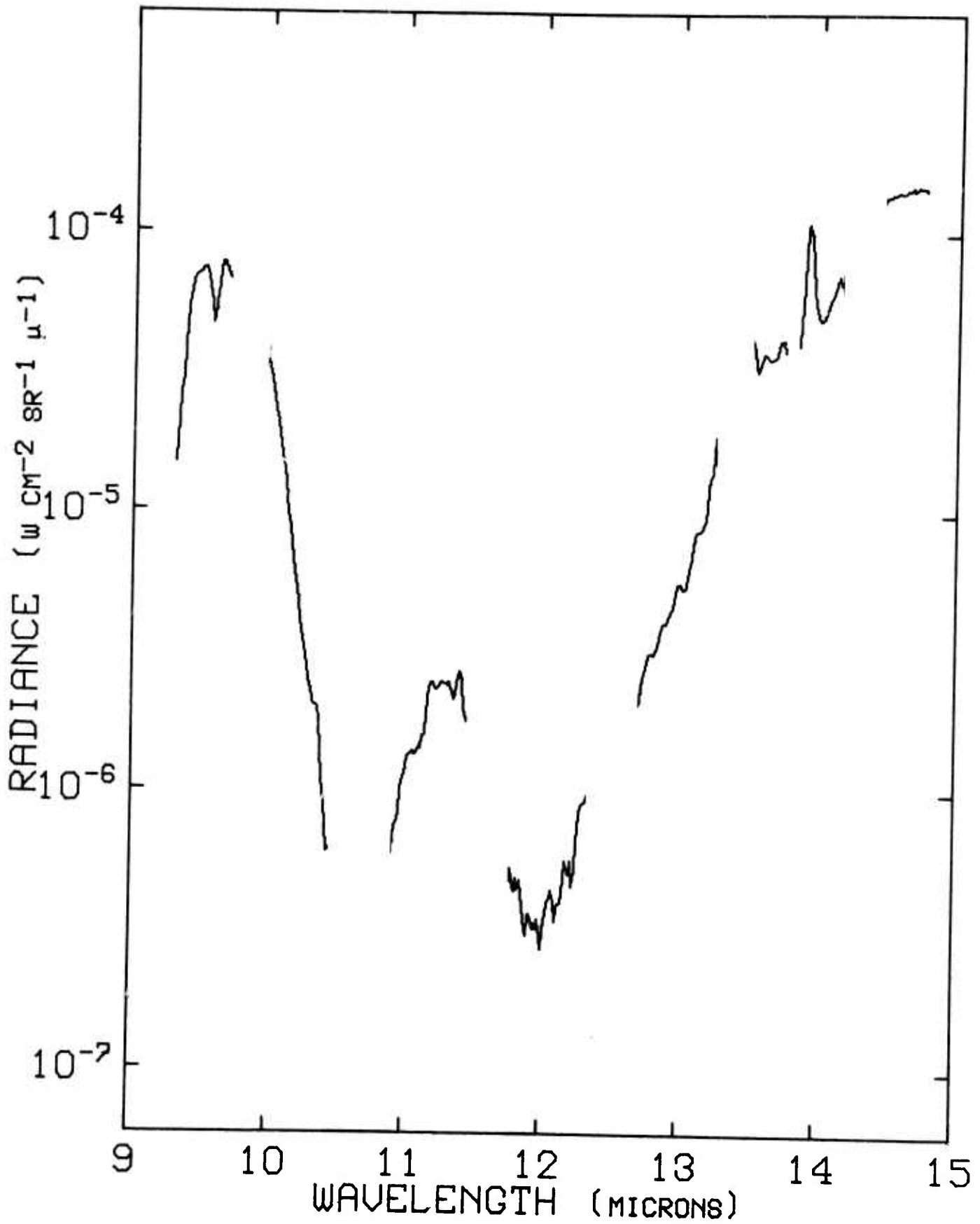
Figure 39. Radiance vs Wavelength at 47.0 kft and 0235 ADT, 12 September 1971.
