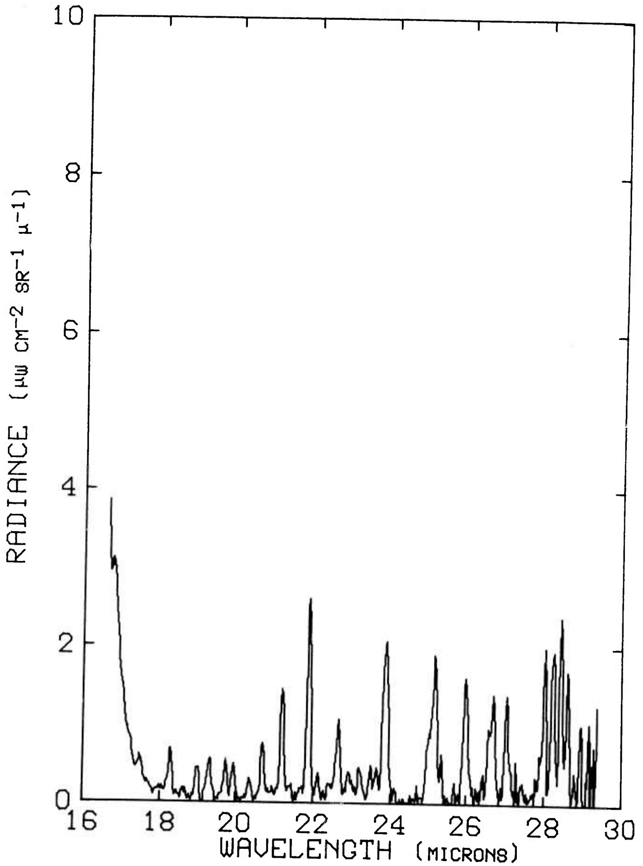
Figure 209. Radiance vs Wavelength at 88.5 kft and 0437 ADT, 23 September 1971.
