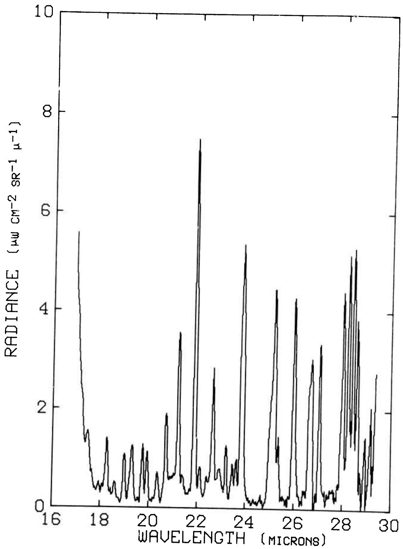
Figure 193. Radiance vs Wavelength at 65.5 kft and 0407 ADT, 23 September 1971.
