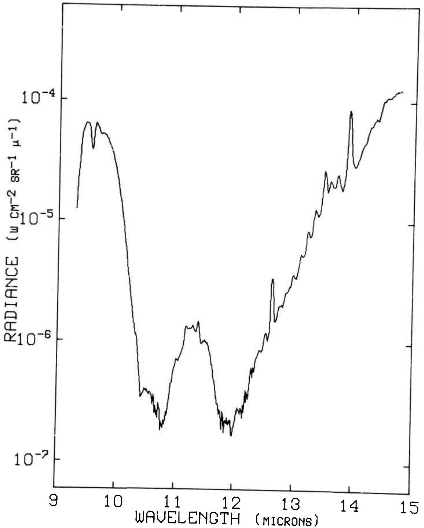
Figure 138. Radiance vs Wavelength at 66.1 kft and 0203 ADT, 15 September 1971.
