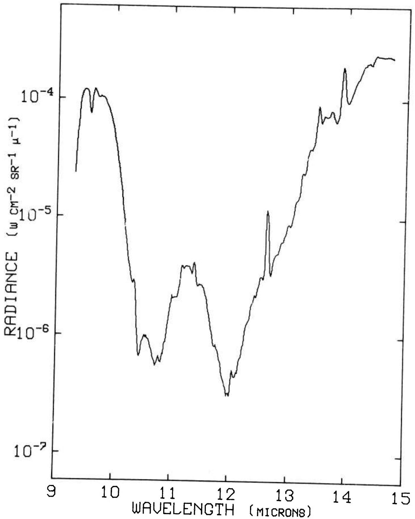
Figure 121. Radiance vs Wavelength at 37.3 kft and 0130 ADT, 15 September 1971.
