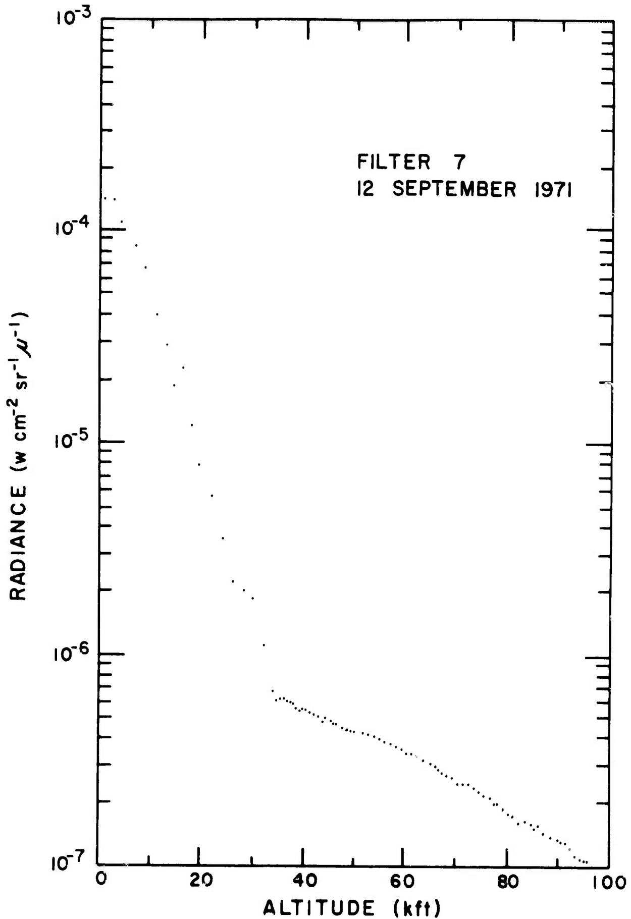
Figure 8. Radiance vs Altitude for Filter 7, 12 September 1971.
