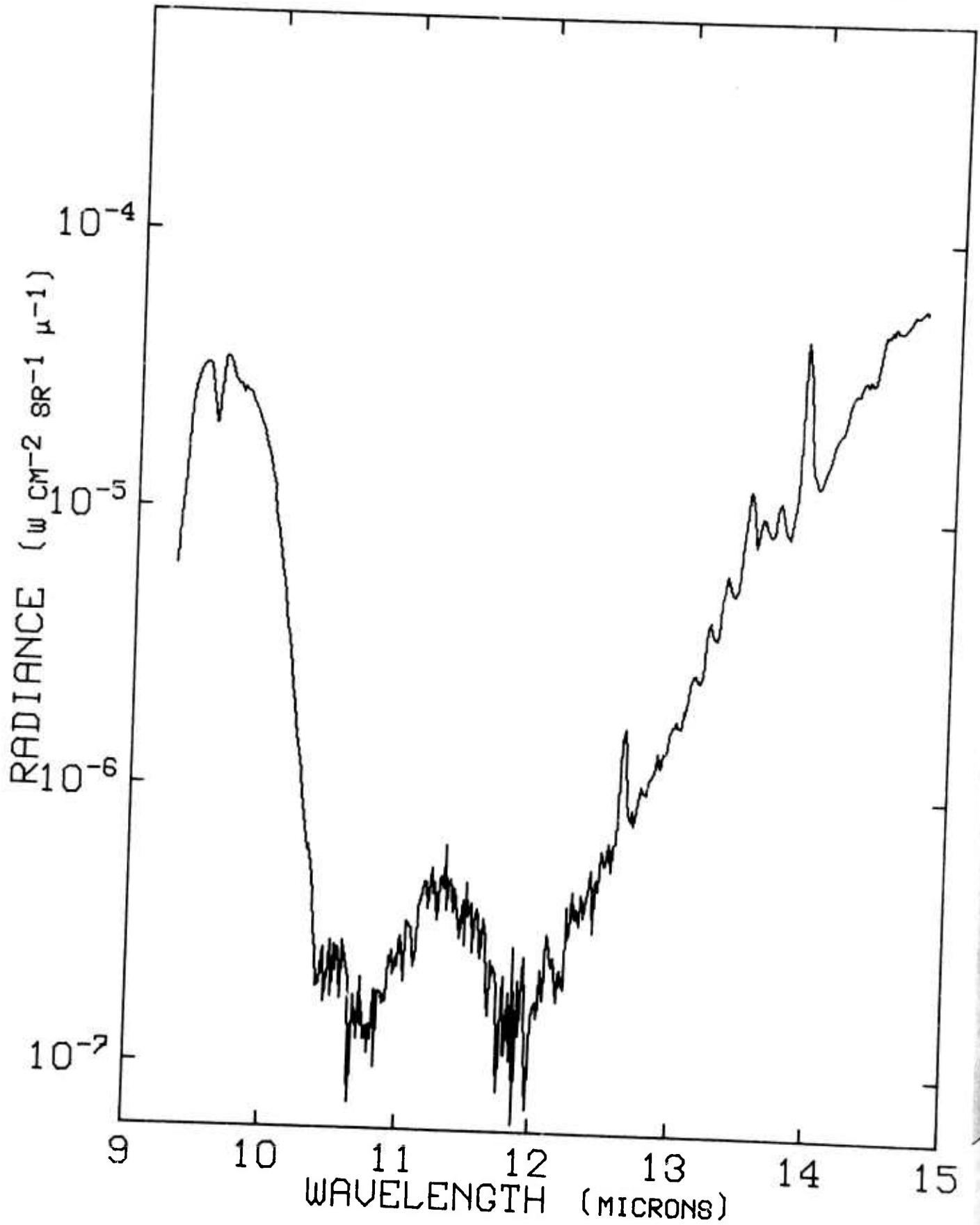
Figure 60. Radiance vs Wavelength at 76.8 kft and 0328 ADT, 12 September 1971.
