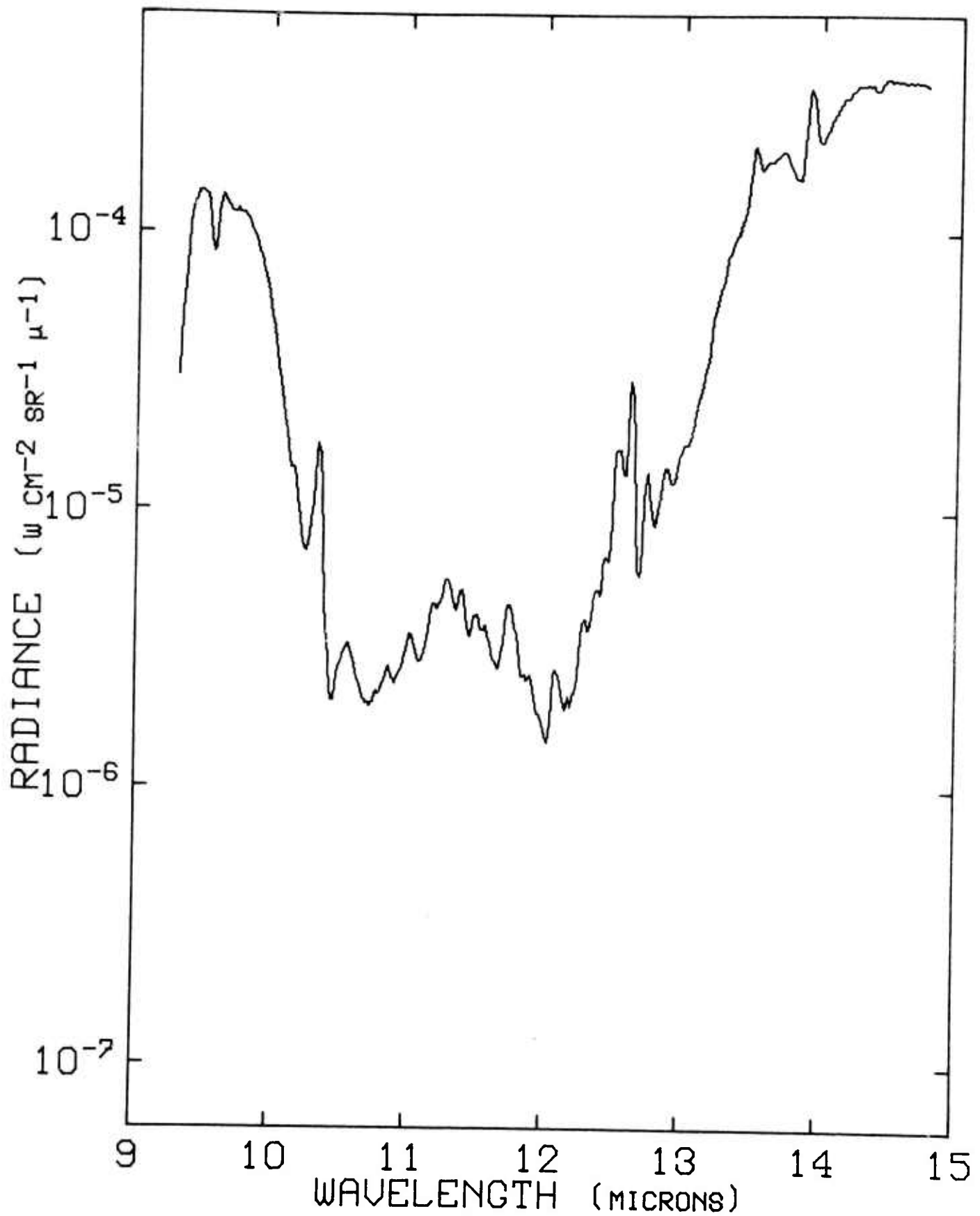
Figure 113. Radiance vs Wavelength at 18.5 kft and 0114 ADT, 15 September 1971.
