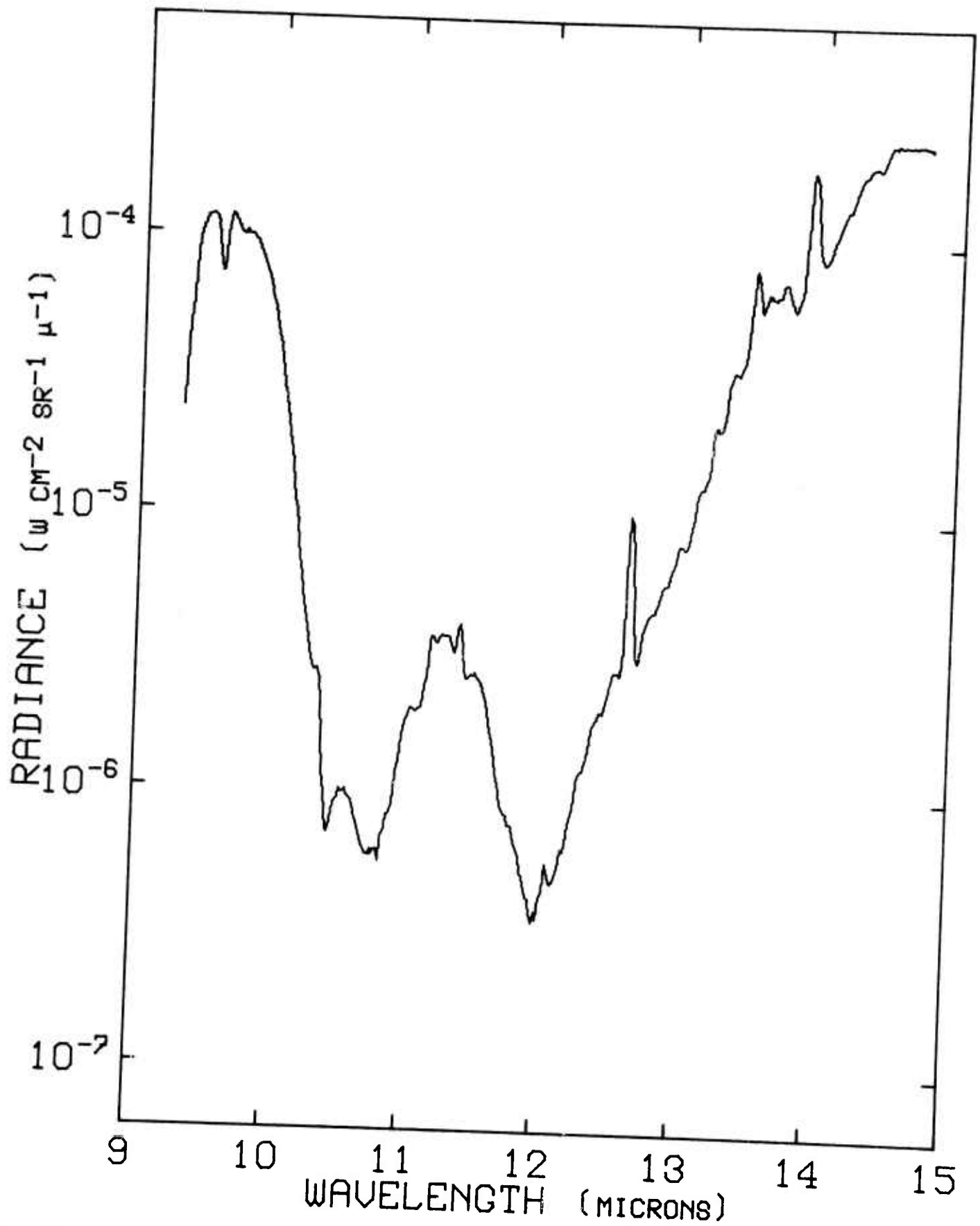
Figure 123. Radiance vs Wavelength at 40.9 kft and 0134 ADT, 15 September 1971.
