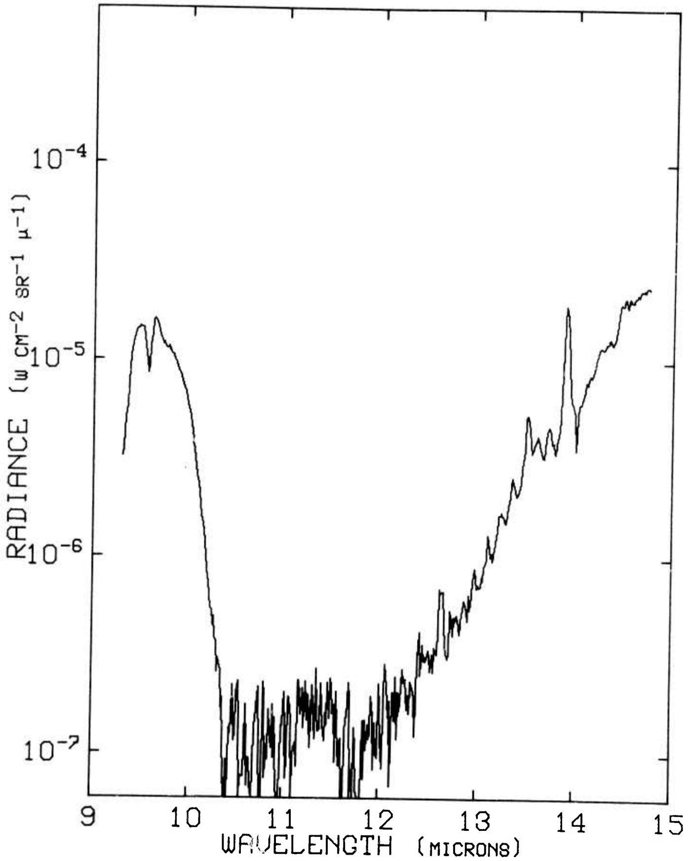
Figure 81. Radiance vs Wavelength at 95.4 kft and 0431 ADT, 12 September 1971.
