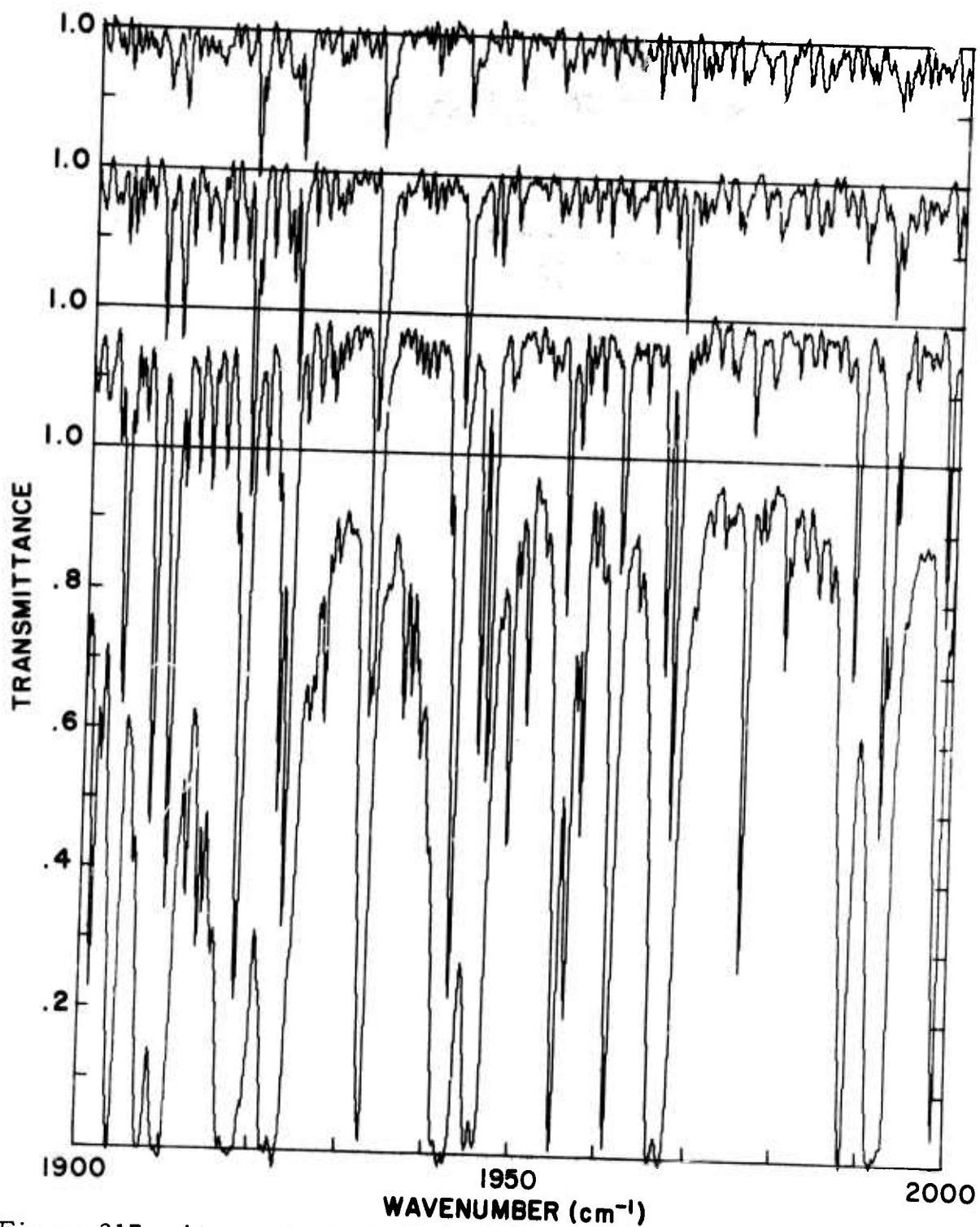
Figure 217. Atmospheric transmittance vs wavenumber at 5.8, 27.6, 42.1 and 68.6 kft with the lowest altitude on the bottom and 0.2 offset in transmittance between each spectrum.
