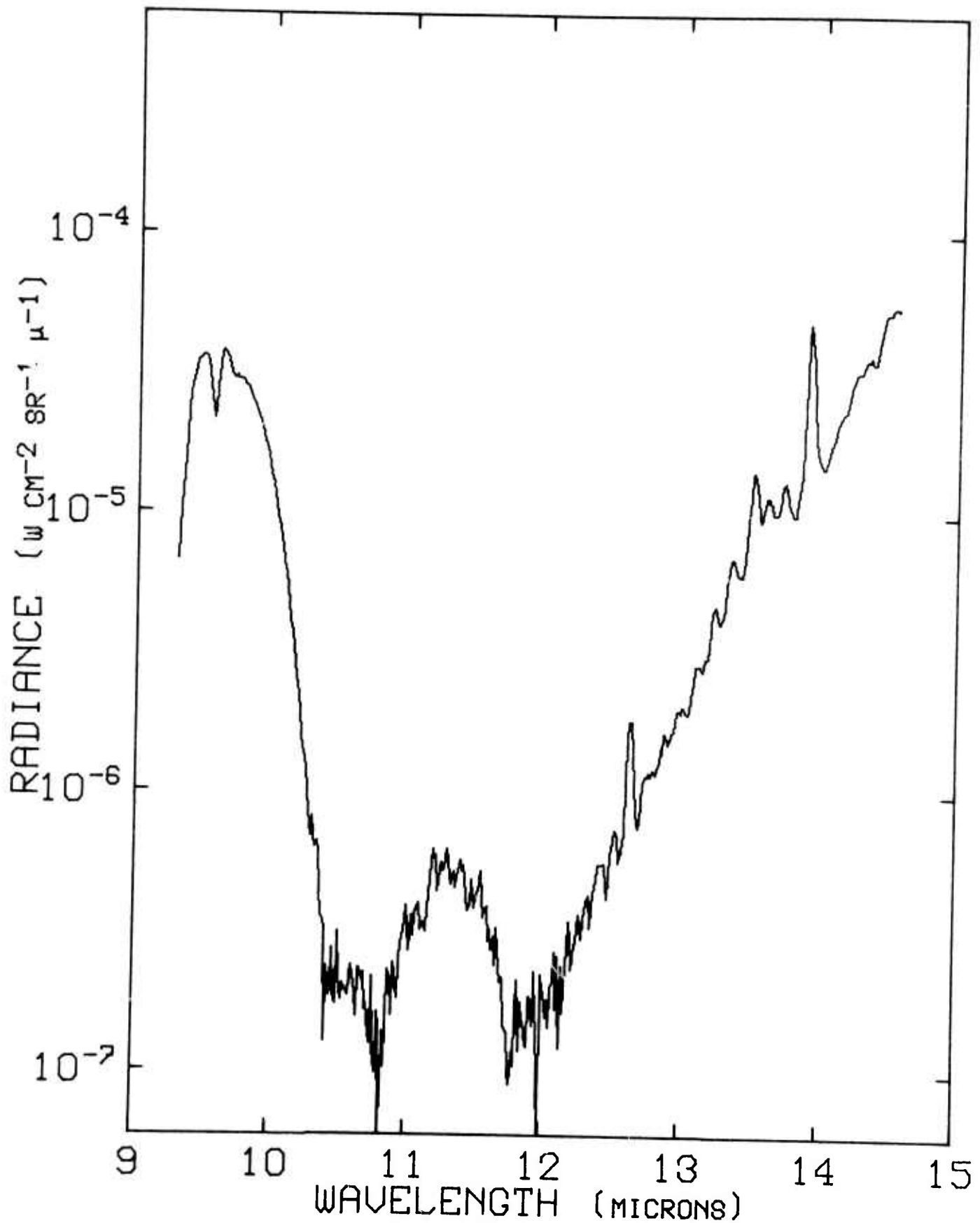
Figure 57. Radiance vs Wavelength at 73.4 kft and 0322 ADT, 12 September 1971.
