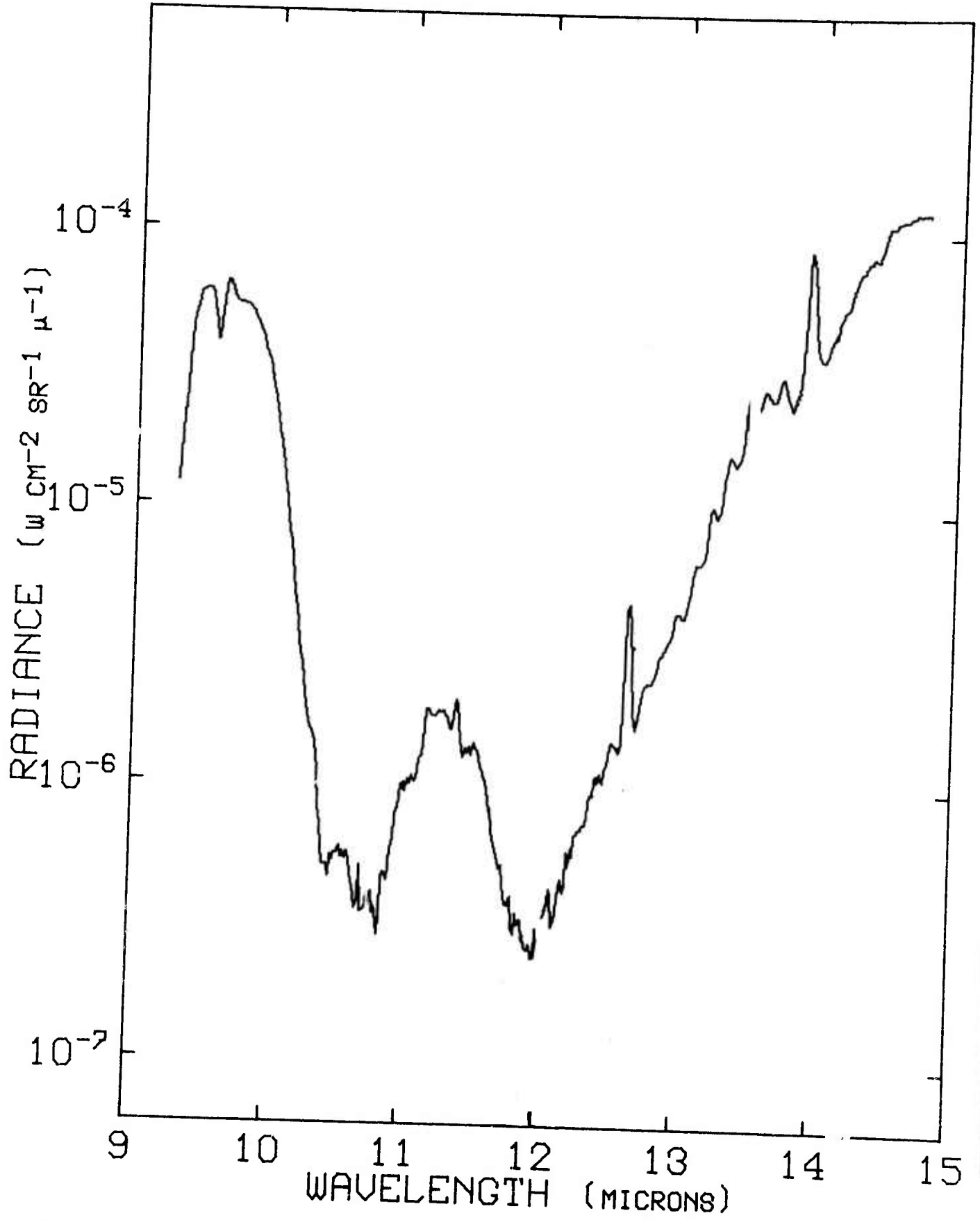
Figure 44. Radiance vs Wavelength at 53.4 kft and 0247 ADT, 12 September 1971.
