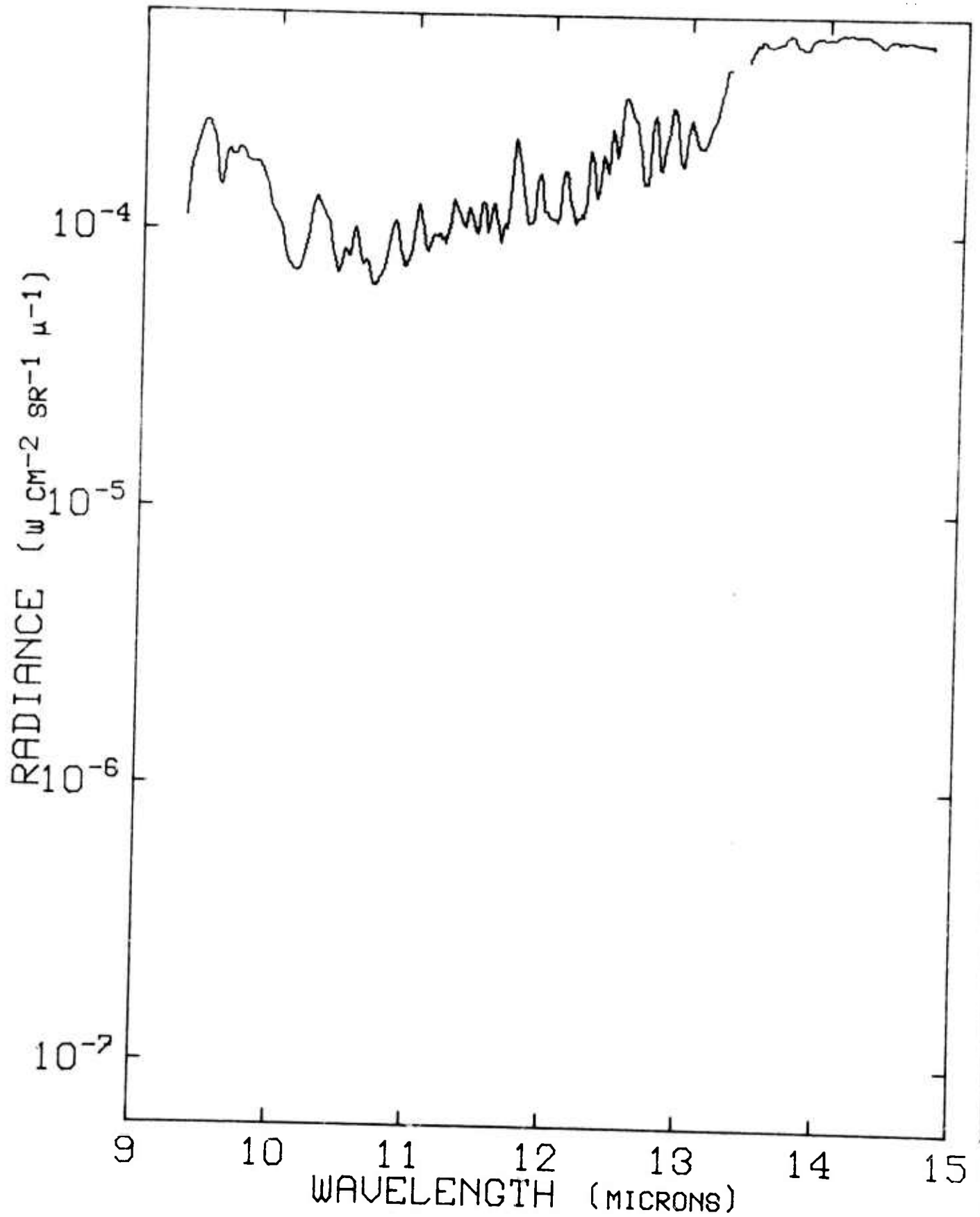
Figure 104. Radiance vs Wavelength at 0.4 kft and 0053 ADT, 15 September 1971.
