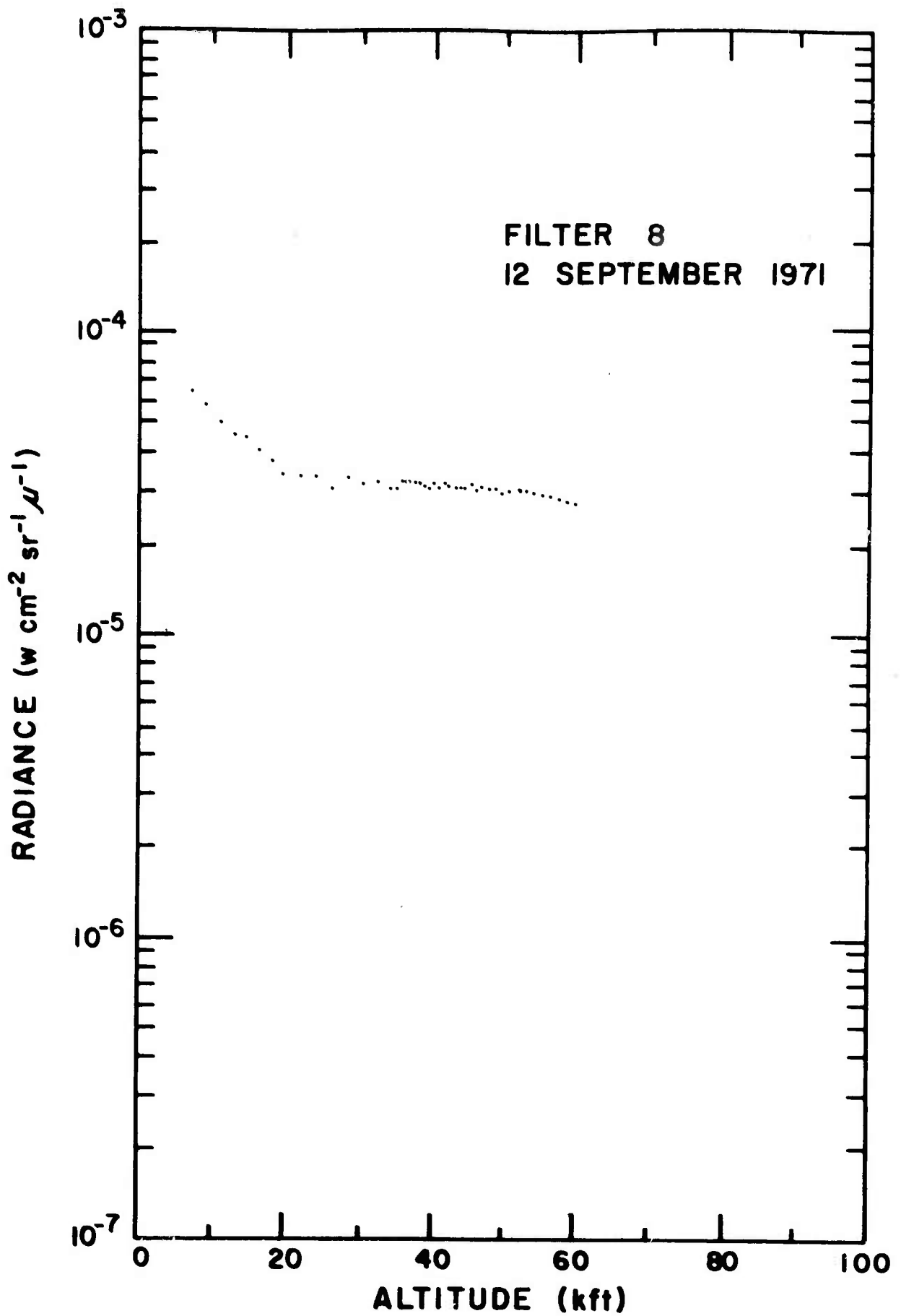
Figure 5. Radiance vs Altitude for Filter 8, 12 September 1971.
