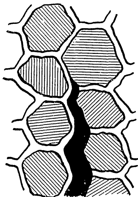
INTERGRANULAR SEPARATION
