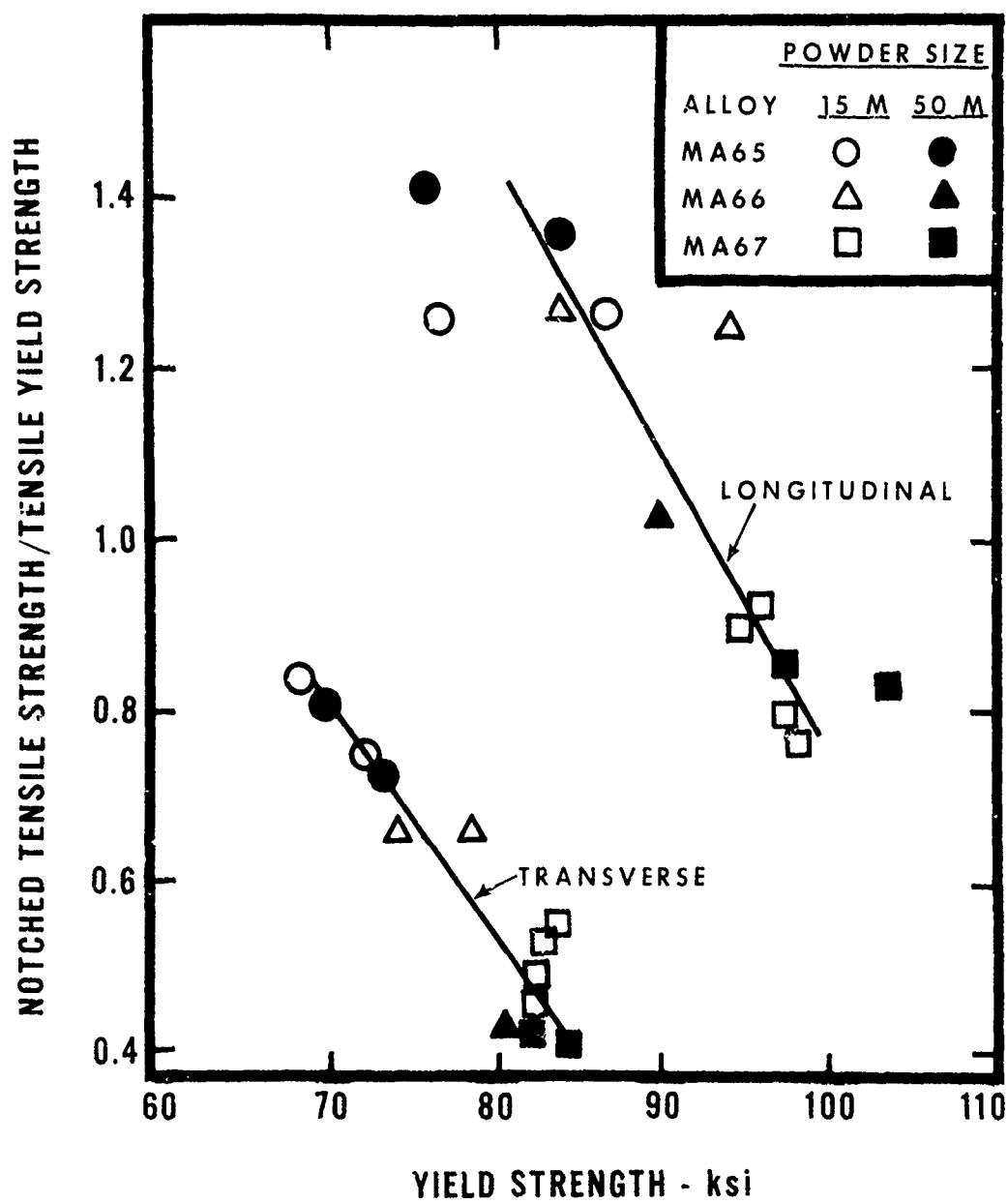
EFFECT OF POWDER SIZE ON THE YIELD STRENGTH TO NTS/YS RELATIONSHIP FOR OCTAGONAL EXTRUDED BAR.
