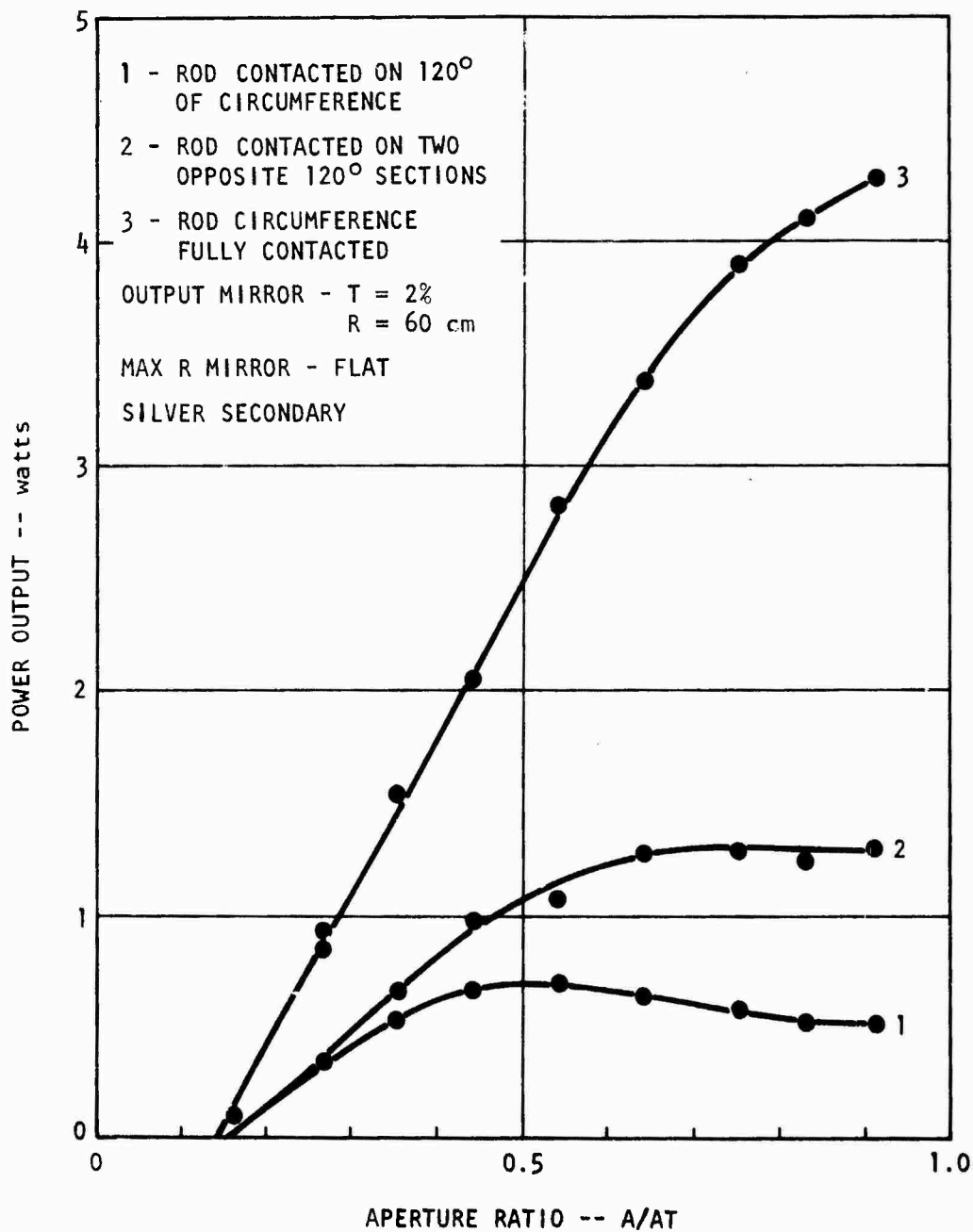
Figure 10 Sun Pumped Laser Performance With the Various Rod-Heat Sink Configurations
